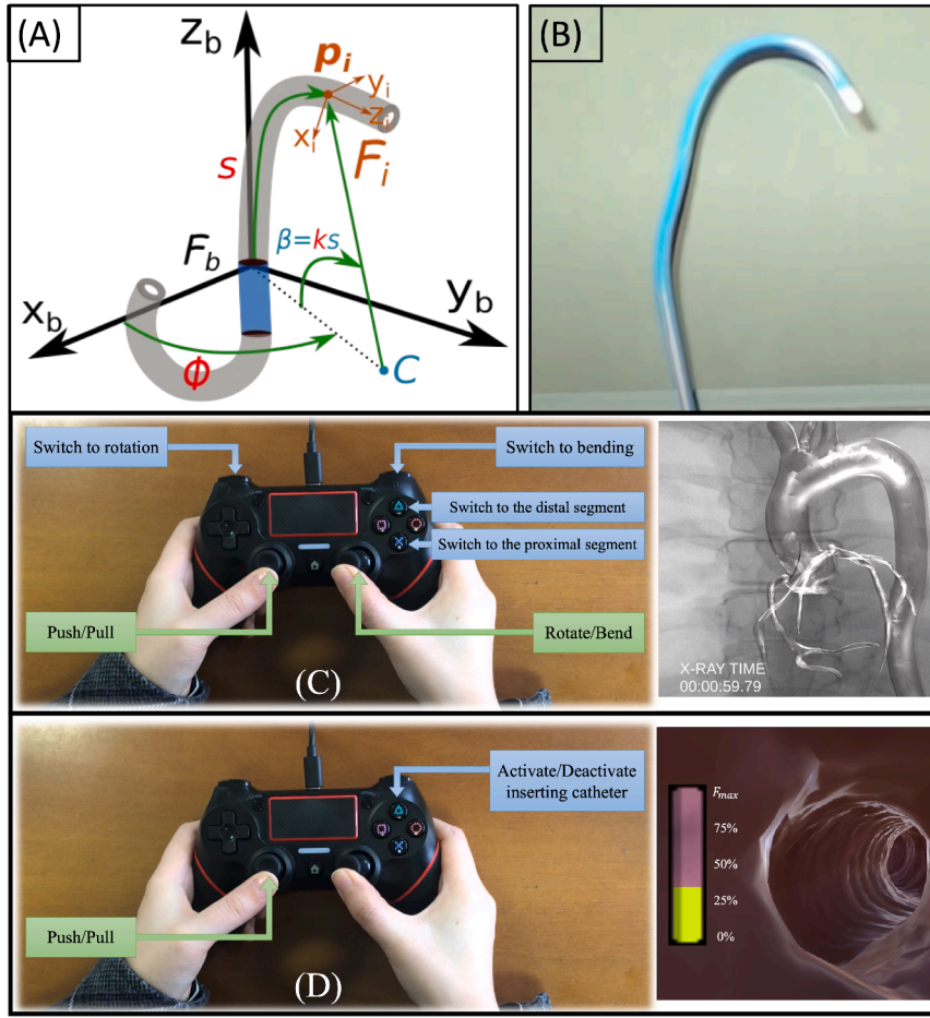
Fig. 4. (A) Parameterization of the steerable segment modeling: \phi denotes the arc rotation angle around z-axis, s is the arc length at p_i , and \kappa is the arc curvature. C denotes the arc center. (B) Megellan robotic catheter. The joystick controller settings for (C) steerable catheter and (D) flexible guidewire. The GUI includes a fluoroscopy view with operation time, and an internal view with visual feedback of collision force.
