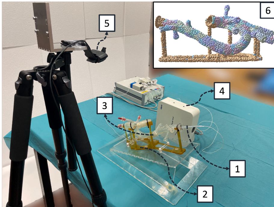
Fig. 5. The in-vitro experimental setup: (1) a catheter with EM sensor embedded at the tip (2) an aortic phantom with support (3) the second EM sensor attached to the surface of the phantom (4) Aurora EM field generator (5) an external camera for filming the experiments (6) The PBD model in the simulator with fixed particles marked in orange.
