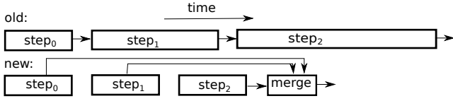
Figure 3: Datagen: old vs new execution flow.
