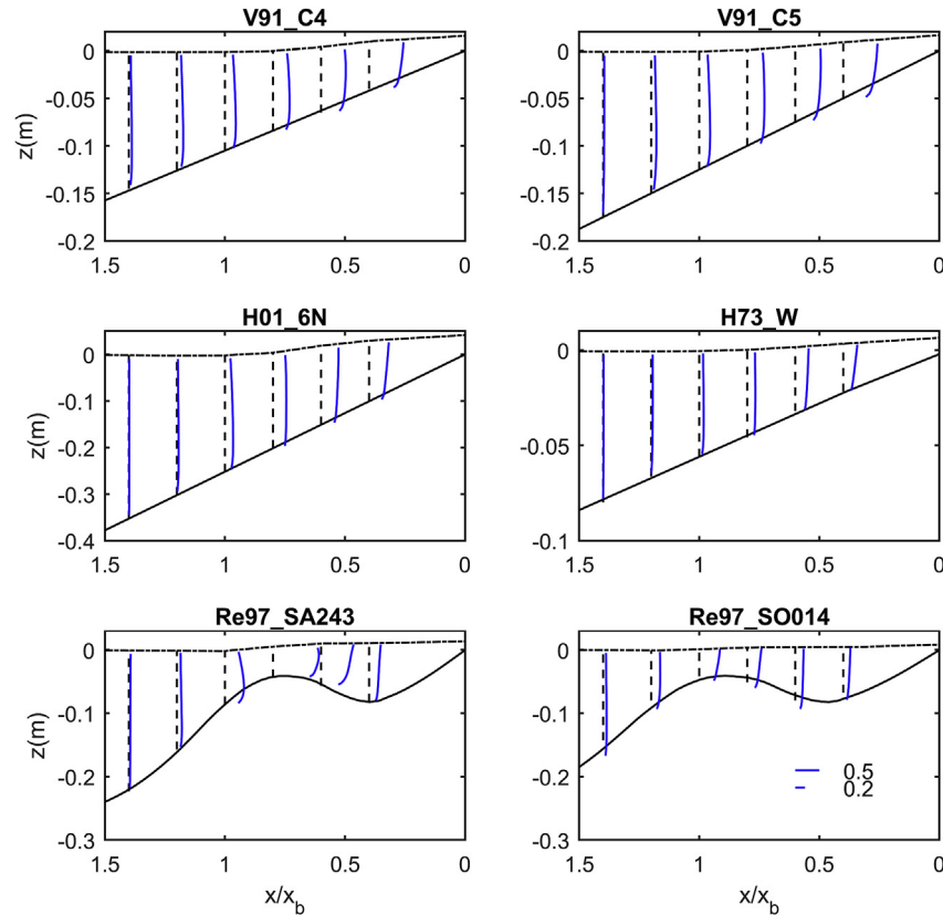
Fig. 12. The vertical profiles of normalised longshore shore current \bar{v}/c , c(=\sqrt{gd}) is local wave celerity. The vertical black dash line denotes the vertical profile location and indicates the zero value of each vertical profile of \bar{v}/c (blue line). The dash dot and solid black lines represent the mean water level and slope bottom, respectively. The scale is given in Re97_SO014 figure. (For interpretation of the references to colour in this figure legend, the reader is referred to the Web version of this article.)
