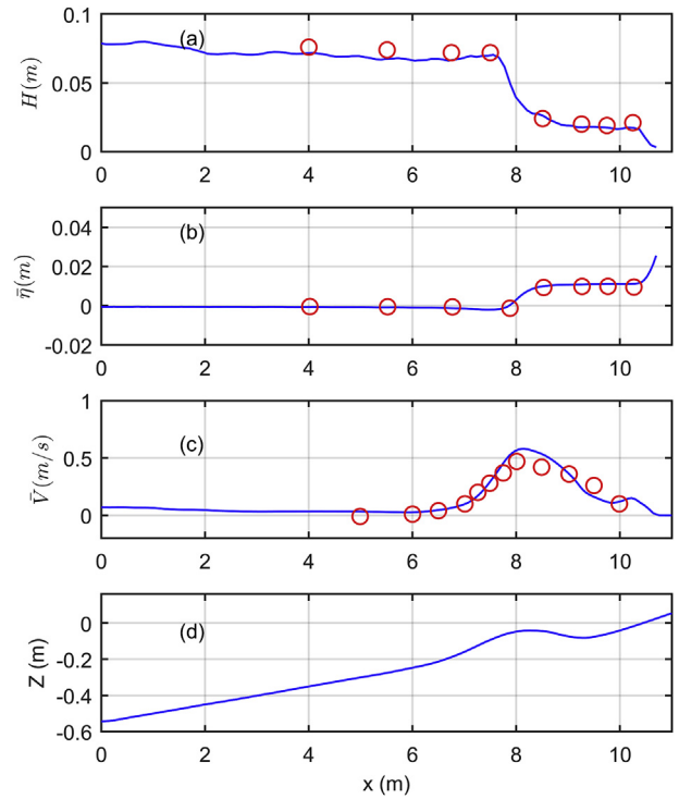
Fig. 8. Case R97_SA243 ( H = 0.08 m, T = 1 s, \theta = 30^\circ ); the cross-shore distribution of wave height (a), wave set up (b), longshore current (c) and the bottom profile (d), (blue lines: simulations, red circles: measurements). (For interpretation of the references to colour in this figure legend, the reader is referred to the Web version of this article.)
