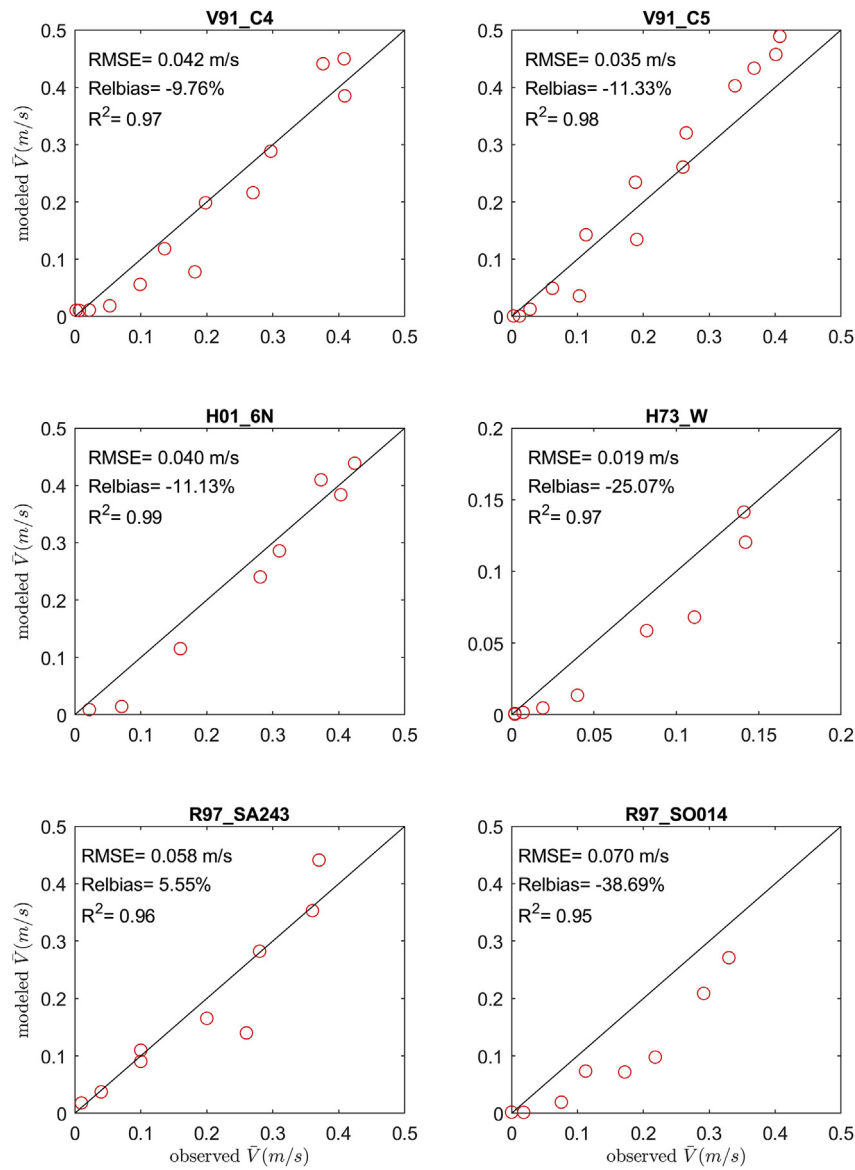
Fig. 10. Comparison of modelled and observed longshore current velocities for each experiment showing RMSE, Bias, and R^2 values. Black solid lines represent perfect agreement.
