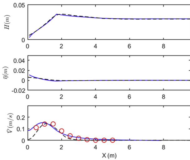
Fig. 13. Comparison between the simulated results of the H73_W experiment by the 1D model (blue line) and the results obtained by the SWASH model (black dash line), (red circles: measurements). (For interpretation of the references to colour in this figure legend, the reader is referred to the Web version of this article.)
