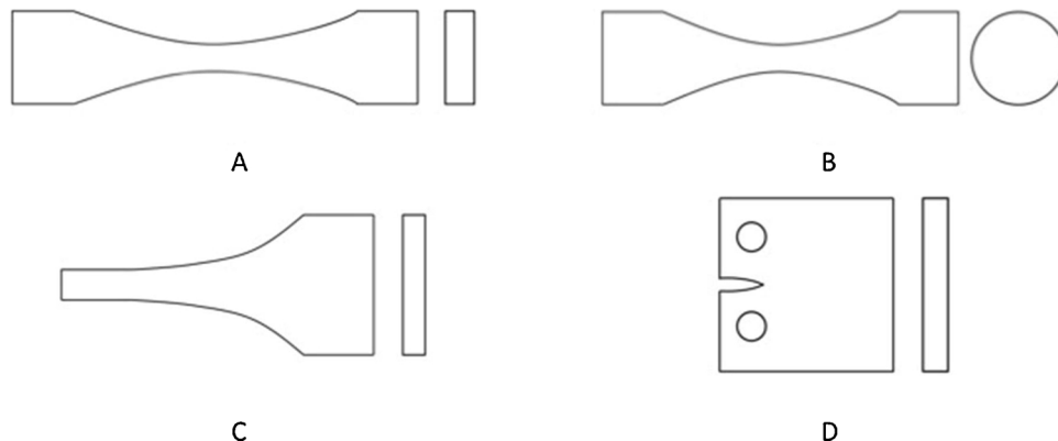
Fig. 3. Four examples of fatigue testing specimens that include A) an axial loading specimen, B) a rotating bending specimen, C) a reverse bending specimen, and D) a fracture mechanical test specimen.
