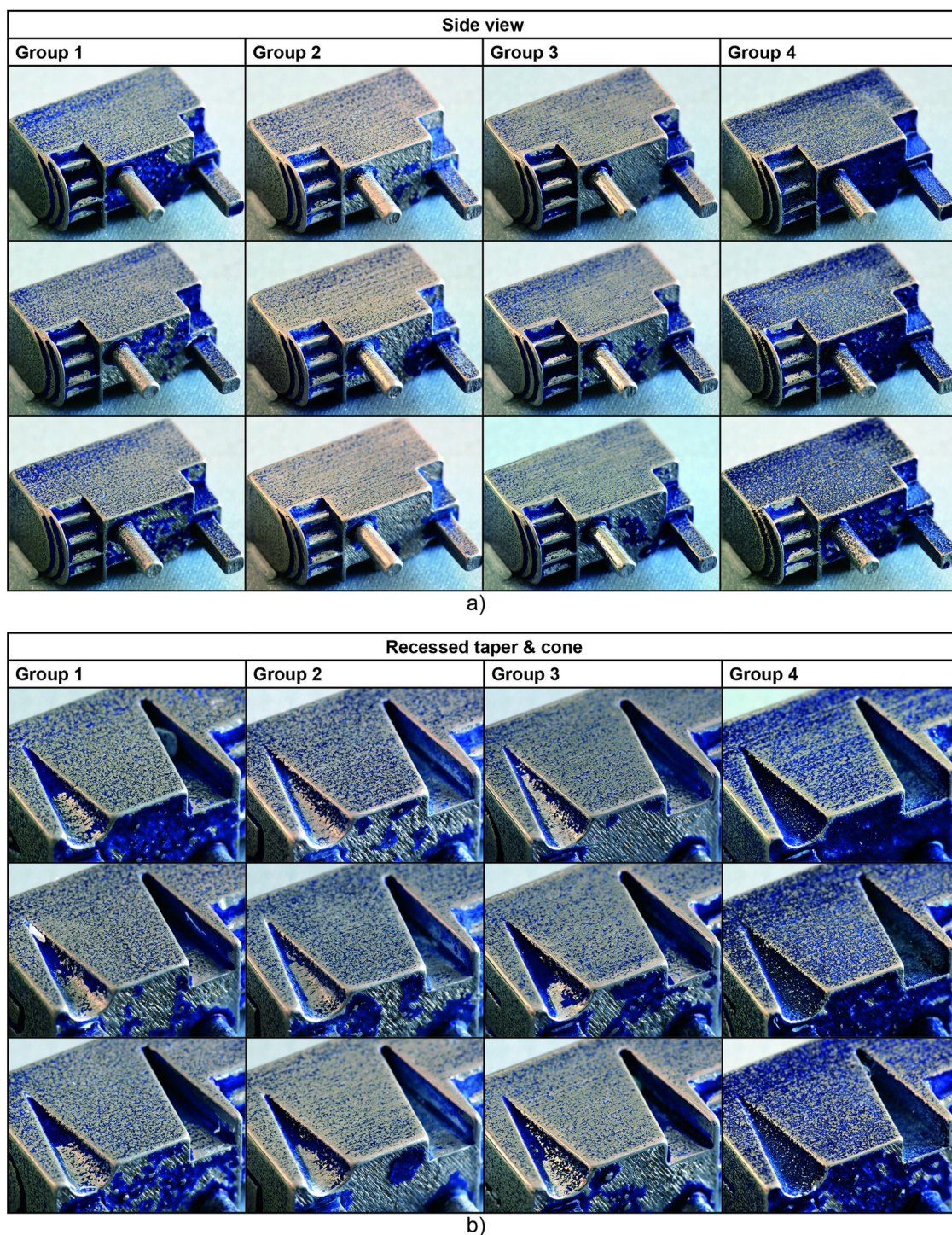
Fig 5. Remaining blue lacquer on the test parts after polishing. a) Side view of all test parts per group. b) Close up of the recessed taper and cone on the other side of the test parts.
