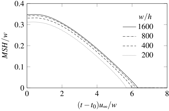
Figure 3: Corresponding Mach stem height evolution for d\vartheta_2(t)/dt = 0.01w/u_\infty \text{ rad s}^{-1} and different grid sizes h = \Delta x = \Delta y .
