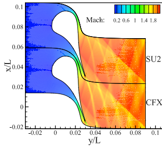
Figure 7: Mach contour.
