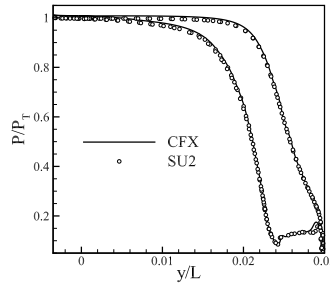
Figure 8: Pressure distribution along the blade surface.
