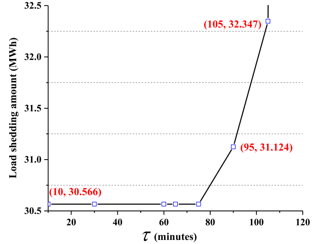
Fig. 8. Sensitivity of total amount of load shedding to \tau in case 3.
