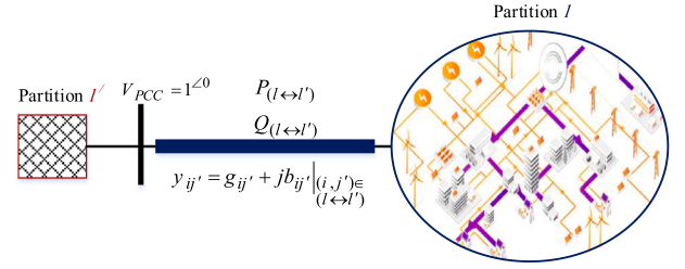
Fig. 2. Simplified representation of l' partition as seen from partition l side.
