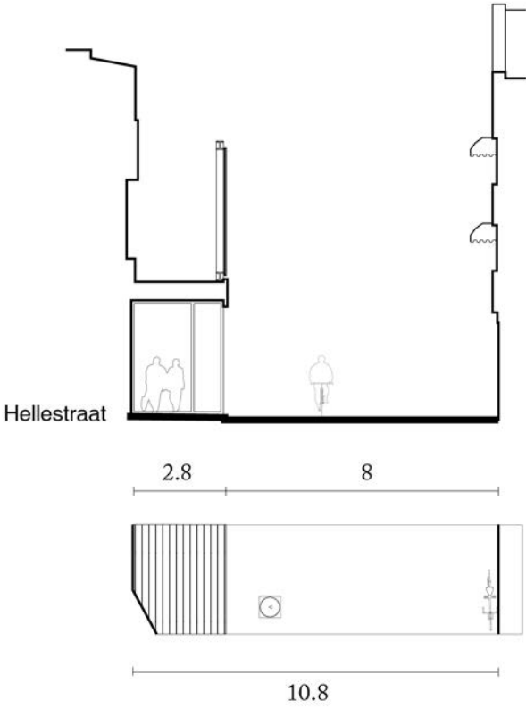
SECTION C SECONDARY STREET
