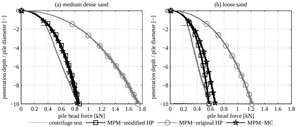
Figure 5.8: Load-displacement curve of the pile head during pile installation for a) medium dense sand ( e = 0.68, R_D = 54\% ) and b) loose sand ( e = 0.75, R_D = 36\% ). Comparison of centrifuge test results and MPM simulations using Mohr Coulomb model (MPM-MC) and hypoplastic model (MPM-original HP and MPM-modified HP).
