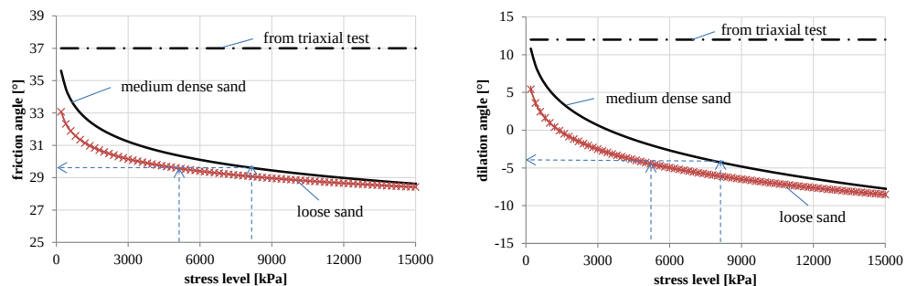
Figure 5.5: Calculated friction and dilation angle used in Mohr-Coulomb model for both medium and loose sand to simulate the pile installation according to Bolton.
