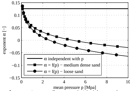
Figure 5.6: Dependency of exponent \alpha on cell pressure in triaxial response
