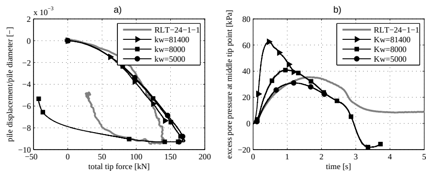
Figure 7.6: Influence of water bulk modulus K_w on the rapid load test results.(simulation with K_0 = 0.46 and k = 8.85 \times 10^{-5} m/s)
