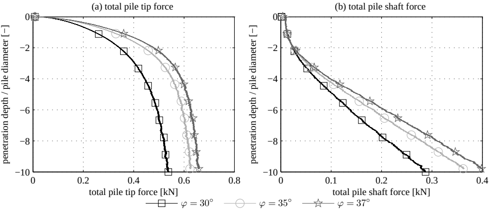
Figure D.4: Influence of friction angle on analysis results. Simulations with Mohr-Coulomb model, E = 30 MPa and \psi = 0^\circ .
