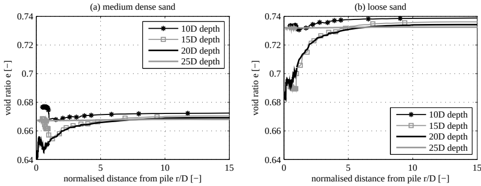
Figure 5.18: Void ratio distribution in horizontal cross sections at different depth after 10D penetration for a) medium dense sand ( e = 0.68 , R_D = 54\% ) and b) loose sand ( e = 0.75 , R_D = 36\% ).
