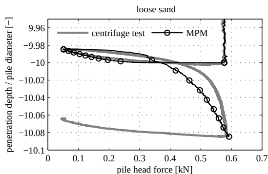
Figure 5.10: Load-displacement curve of the pile head during unloading and reloading phase for loose sand ( e_0 = 0.75 , RD = 36\% ). Comparison of centrifuge test results and MPM simulations.
