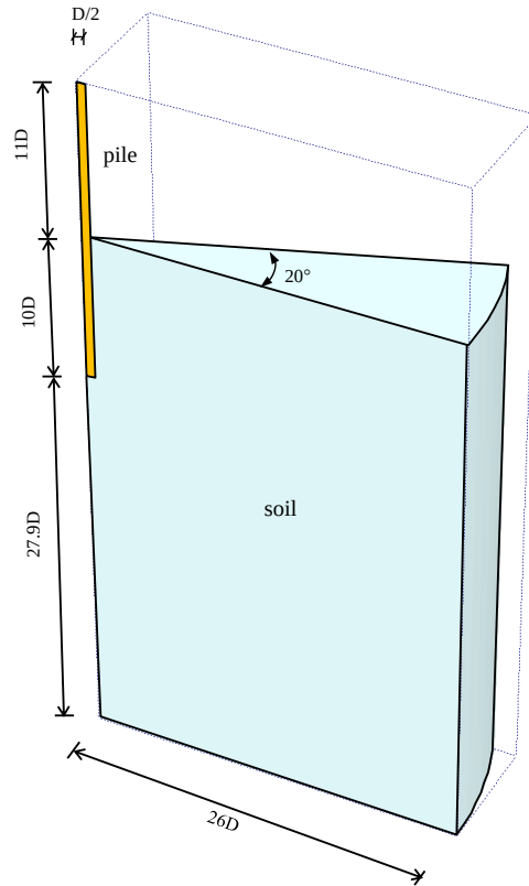
Figure 5.2: Geometry of considered problem
