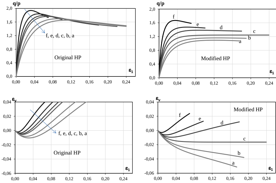
Figure 5.23: Triaxial response of Baskarp sand at elevated cell pressures: a = 30 \text{ MPa} , b = 16 \text{ MPa} , c = 6 \text{ MPa} , d = 4 \text{ MPa} , e = 2 \text{ MPa} , f = 0.5 \text{ MPa} . Comparison between original HP and modified HP model.
