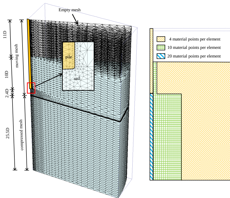
Figure 5.3: Mesh discretization and the distribution of material point method used for numerical analysis with MPM
