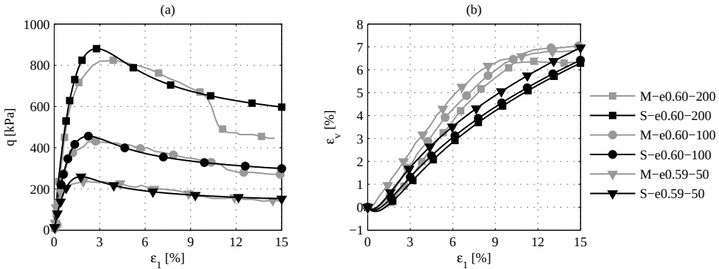
Figure C.2: Numerical simulation of triaxial compression test on dense sand specimens. (a) Deviatoric stress vs. axial strain and (b) Volumetric strain vs. axial strain. M-e0.60-200 means measurement data for specimen with void ratio of 0.6 at confining pressure of 200 kPa; S-e0.60-200 means simulation data for specimen with void ratio of 0.6 at confining pressure of 200 kPa
