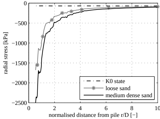
Figure 5.14: Radial stresses after 10D penetration at horizontal cross section AA' for medium dense and loose sand, hypoplastic model.
