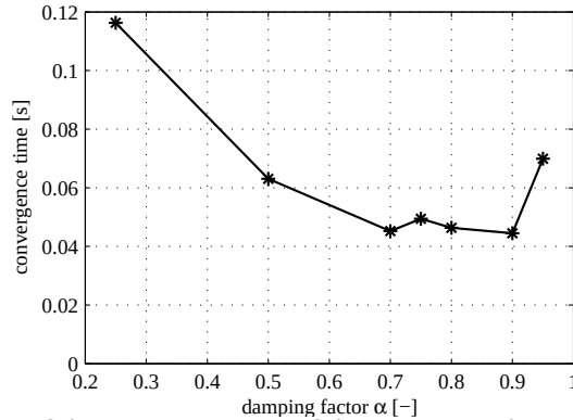
Figure 3.5: Dependency of the convergence time of the compression beam simulation on the local damping factor \alpha
