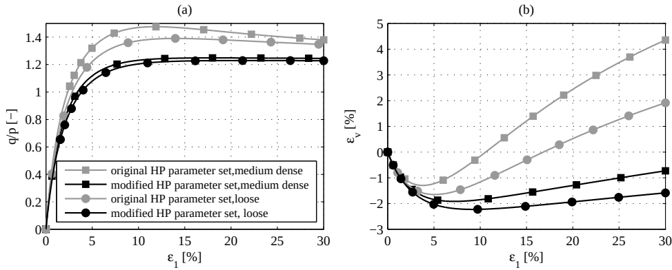
Figure 5.7: Comparison of triaxial element test simulations at 10 MPa on Baskarp sand using the modified hypoplastic parameter set ( \alpha_{modified} = 0.02 ) with one using the original parameter set ( \alpha_{original} = 0.12 )
