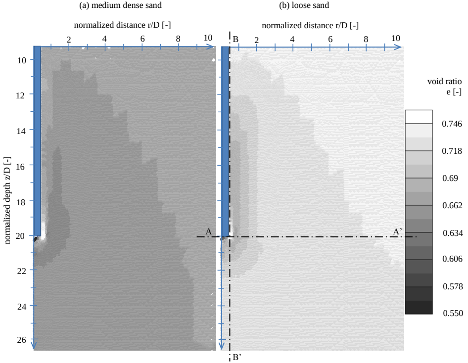
Figure 5.16: Void ratio change after 10D penetration. MPM simulation for a) medium dense sand ( e = 0.68 , R_D = 54\% ) and b) loose sand ( e = 0.75 , R_D = 36\% ).
