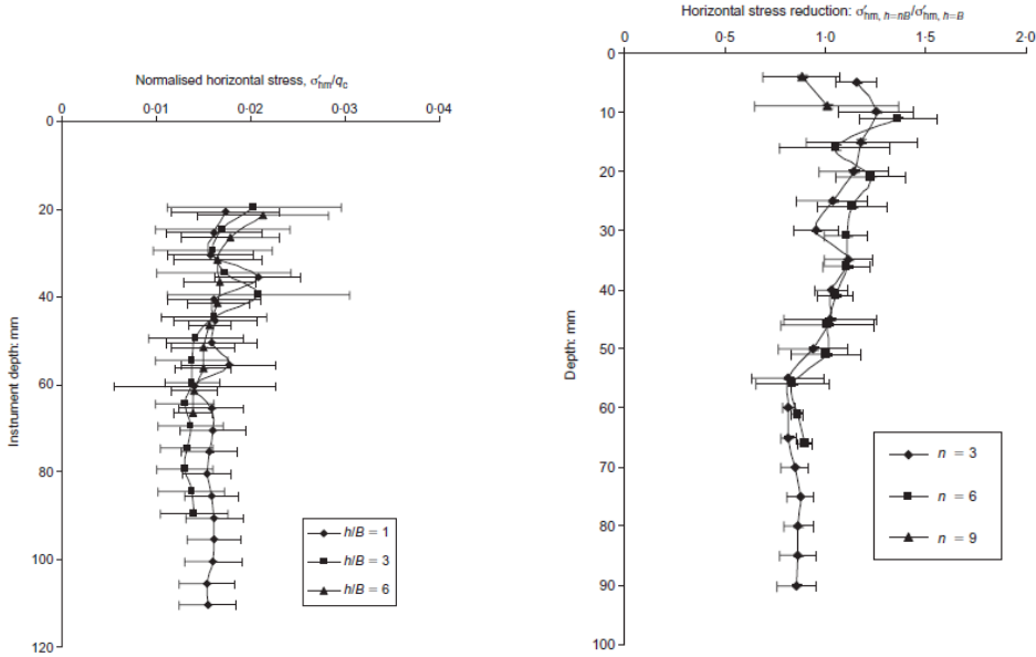
(a) normalised horizontal stress during monotonic installation (mean of all four tests).
