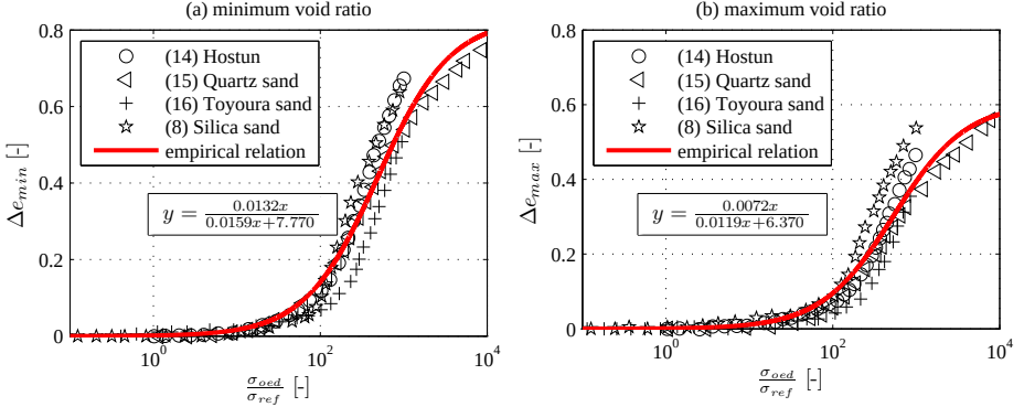
Figure 4.2: Dependency of the minimum (a) and maximum (b) void ratio on stress level for various sands listed in Table 4.1.
