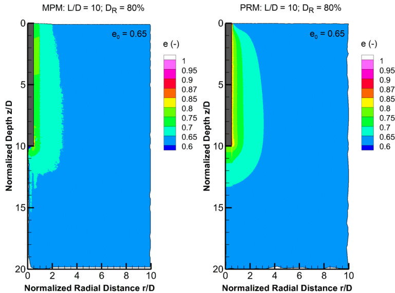
(c) MPM in the dense sand
