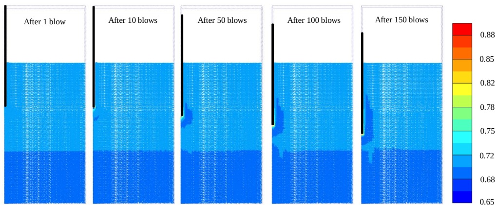
Figure 6.11: Calculated void ratio distribution after 1 blow, 10 blows, 50 blows, 100 blows and 150 blows of pile driving in saturated medium dense sand .
