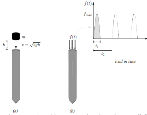
Figure 6.1: a) Illustration of hammer drop, b) corresponding force function ([5])
