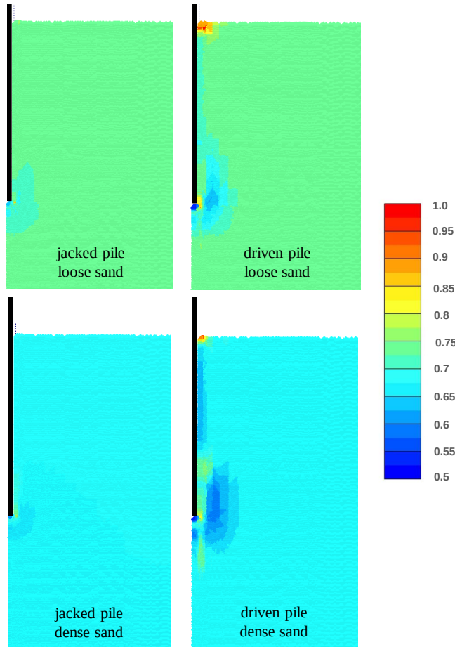
Figure 6.15: Void ratio distribution after 4.5D penetration. Comparison between jacked pile and driven pile for both loose and medium dense sand
