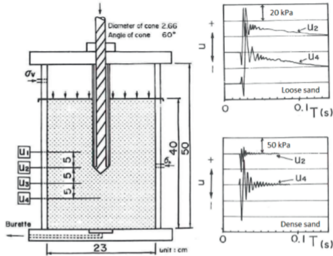
Figure 2.16: Changing of pore pressure during 1 blow of dynamic penetration test [30].
