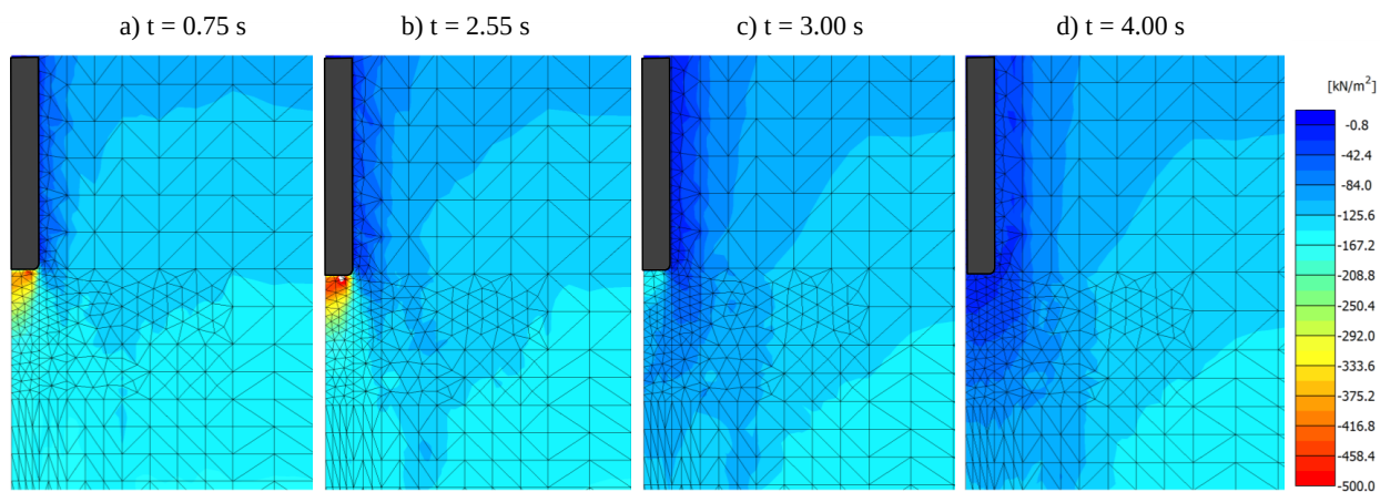
Figure 7.8: Vertical effective stress around the pile tip at different time during RLT 24-1-1
