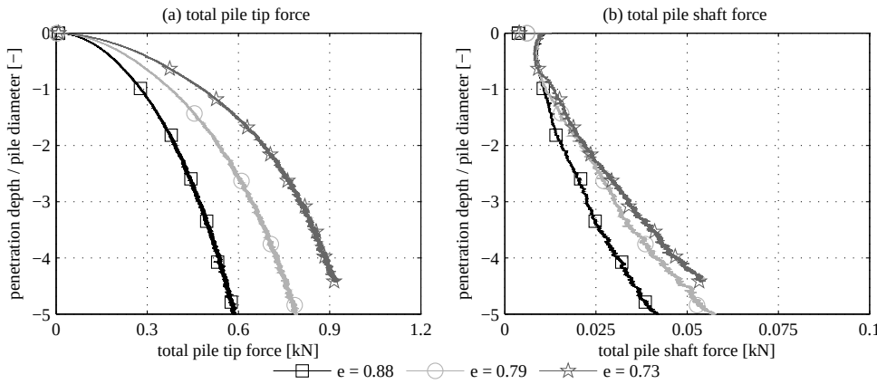
Figure D.9: Influence of initial void ratio on analysis results.
