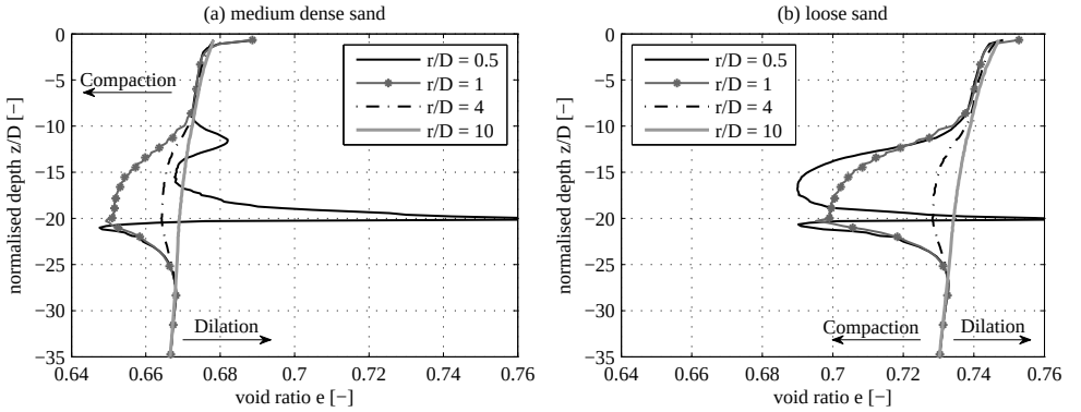
Figure 5.17: Void ratio distribution in vertical cross sections at different radial distances from the center of the pile after 10D penetration for a) medium dense sand ( e = 0.68 , R_D = 54\% ) and b) loose sand ( e = 0.75 , R_D = 36\% ).
