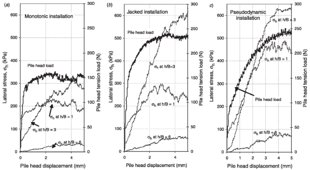
Figure 2.1: Lateral stress variation during static tension load tests after monotonic, jacked and pseudo dynamic installation of piles in fine silica sand. [4].
