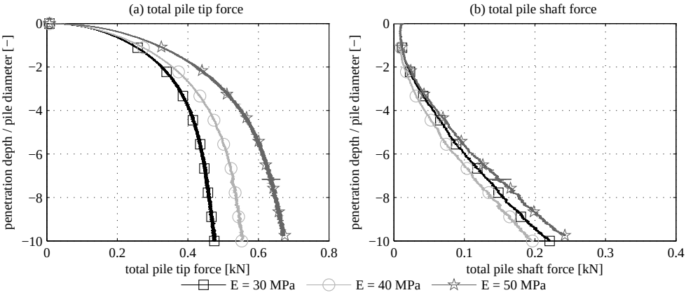
Figure D.3: Influence of soil stiffness on analysis results. Simulations with Mohr-Coulomb model, \varphi = 30^\circ and \psi = 0^\circ .
