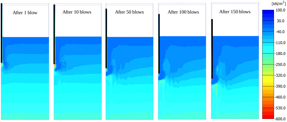
(b) vertical effective stress
