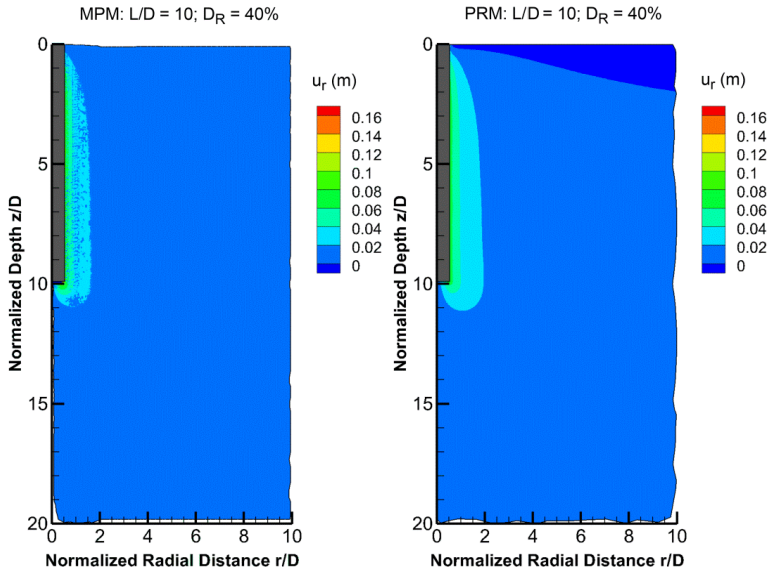
(a) MPM in the loose sand
