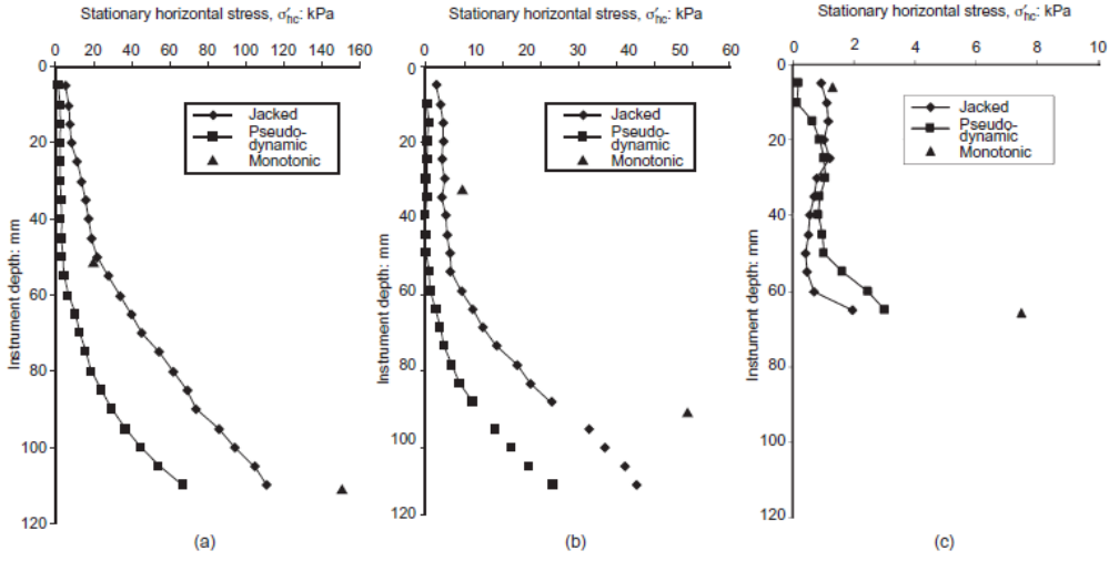
Figure 2.5: Variation of stationary horizontal stress with installation method: (a) h/B = 1 ; (b) h/B = 3 ; (c) h/B = 6 ([7]).
