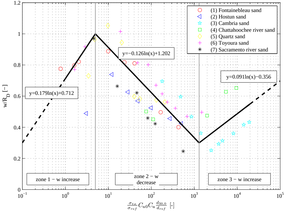
Figure 4.5: Normalised function of w depending on pressure and uniformity.
