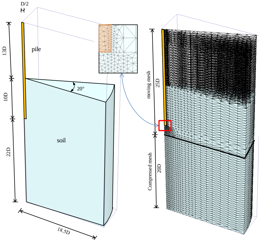
Figure 6.3: Geometry of considered problem and mesh discretization
