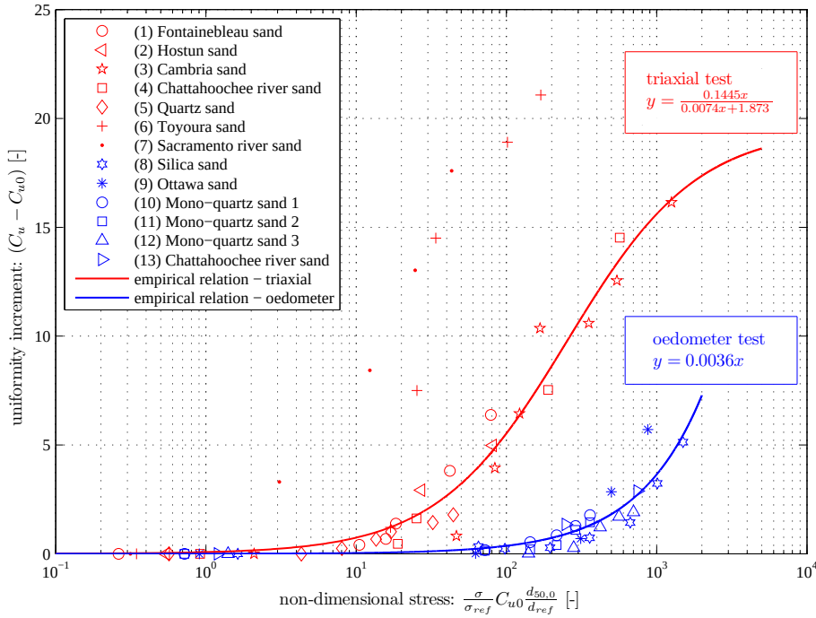
Figure 4.1: Dependency of the uniformity coefficient on the stress level in triaxial compression tests (red) and in one-dimensional compression tests (blue) for various sands listed in Table 4.1.
