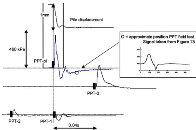
Figure 2.14: Behaviour of excess pore pressure during rapid pile load tests for medium dense sand [31].
