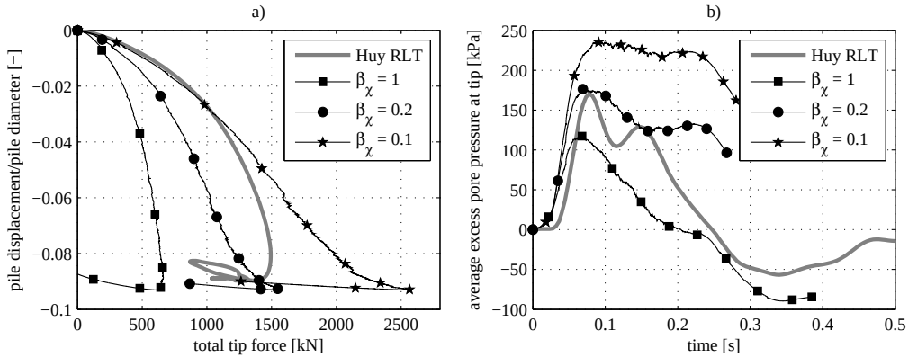
Figure F.3: Influence of different values of \beta_\chi , \beta_\chi = 1, 0.2 and 0.1 on the results of load-displacement curve during the rapid load test.
