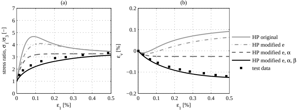
Figure 4.9: Triaxial response of dense Hostun sand ( R_D = 90\% ) at high cell pressures of 10 MPa. Comparison of test result [12] with different hypoplastic model modifications. a) stress ratio versus vertical strain, b) volumetric strain versus vertical strain.
