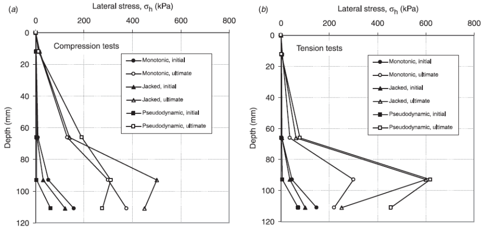
Figure 2.2: Lateral stress profiles before and at ultimate capacity in static load tests [4].
