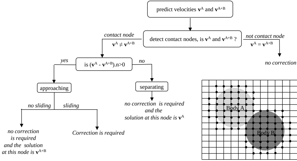
Figure 3.6: Flow chart of the contact algorithm for two bodies A and B by [38]
