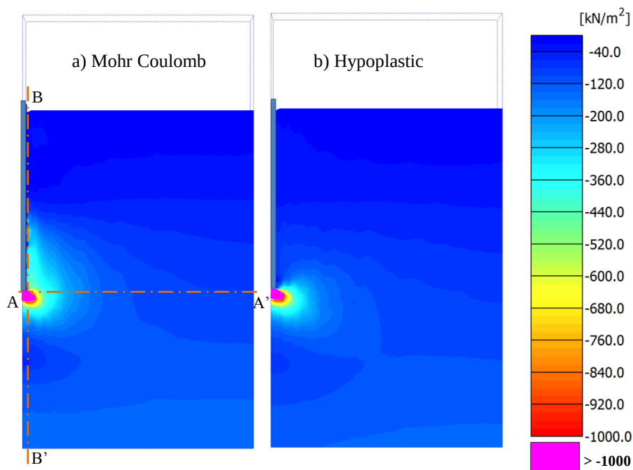
Figure 5.13: Radial stresses after 10D penetration for simulation using a) Mohr Coulomb model and b) hypoplastic model.
