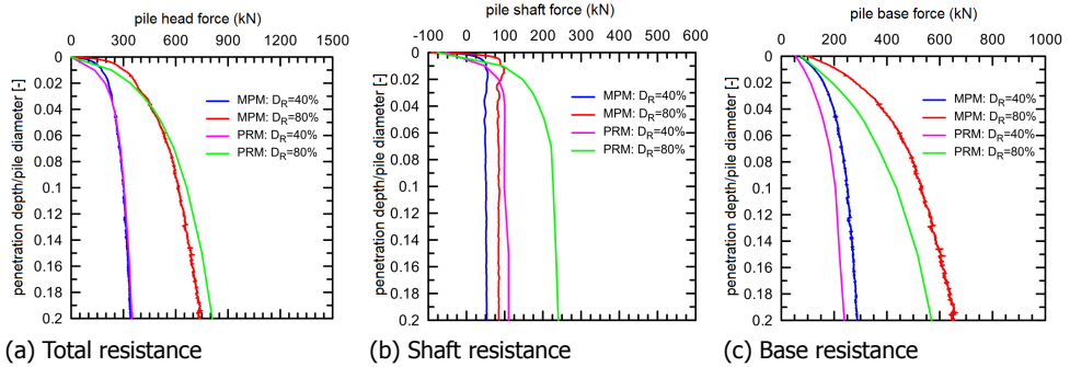
Figure 5.33: Soil resistance during the numerical static load tests (after [3]).
