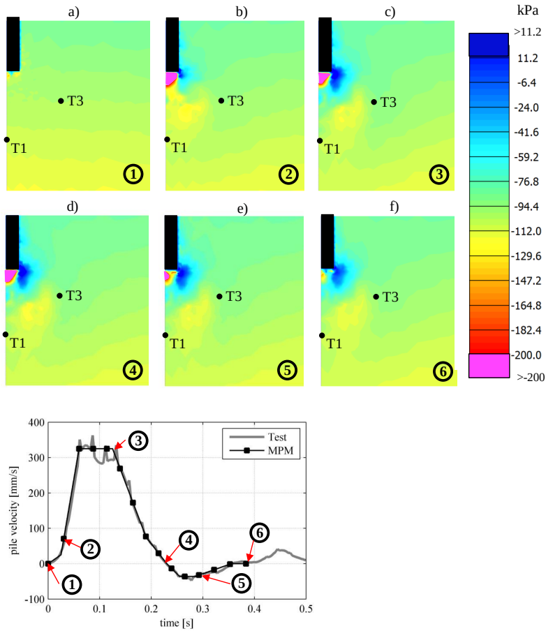
Figure 7.15: Pore pressure generated at different time during rapid load test for medium dense sand.
