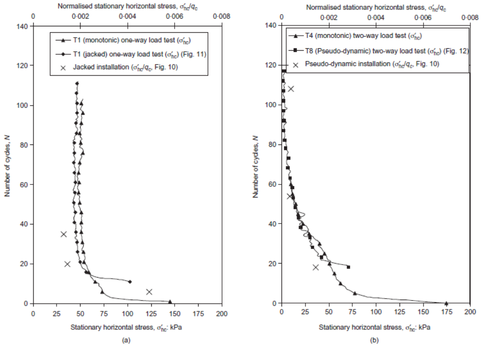
Figure 2.6: Degradation of stationary horizontal stress with cycling at h/B = 1 during load tests: (a) one-way compression load test; (b) two-way compression-tension load test ([7]).
