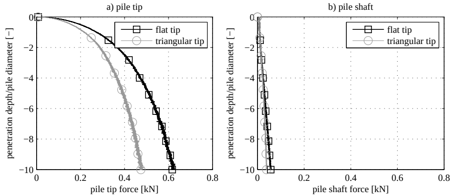
Figure 5.22: Comparison of load-displacement curve of the pile tip during installation between flat and triangular tip shape.
