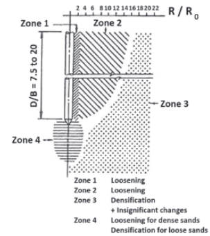
(b) zones of density change around cone penetrometer [16].
