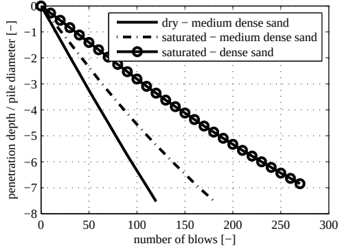
Figure 6.17: Penetration depth per blows, impulse load of 10000 kPa, pile diameter of 0.64 m.
