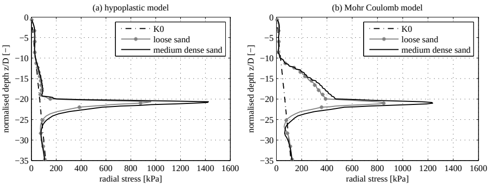
Figure 5.15: Radial stresses after 10D penetration at a vertical cross section BB' close to the pile shaft for medium dense and loose sand. MPM simulation with a) hypoplastic model, b) Mohr-Coulomb model
