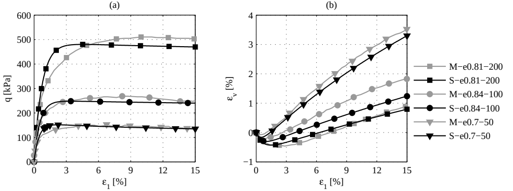
Figure C.3: Numerical simulation of triaxial compression test on loose sand specimens. (a) Deviatoric stress vs. axial strain and (b) Volumetric strain vs. axial strain. M-e0.81-200 means measurement data for specimen with void ratio of 0.81 at confining pressure of 200 kPa; S-e0.81-200 means simulation data for specimen with void ratio of 0.81 at confining pressure of 200 kPa
