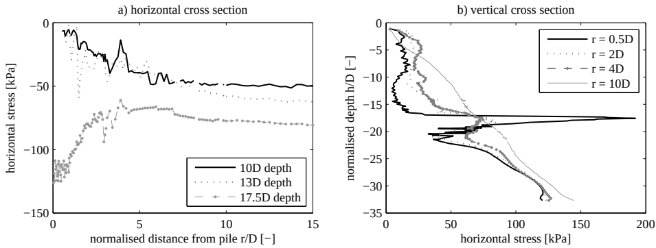
Figure 6.5: Calculated radial stress after 6.5D pile penetration (100 blows) in dry sand for different cross sections: a) horizontal cross section in different depth from the soil surface, b) vertical cross section for different distances to axis of symmetric.
