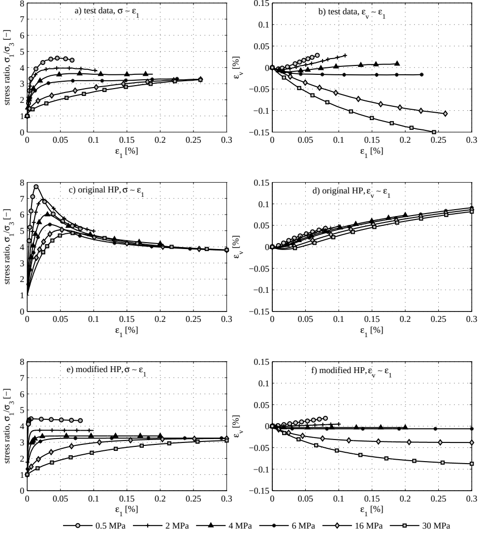
Figure 4.12: Triaxial response of Fontainebleau sand at cell pressures between 500 kPa and 30 MPa, a) and b) are test results [14], c) and d) are simulation results using original hypoplastic model, e) and f) are simulation results using modified hypoplastic model.
