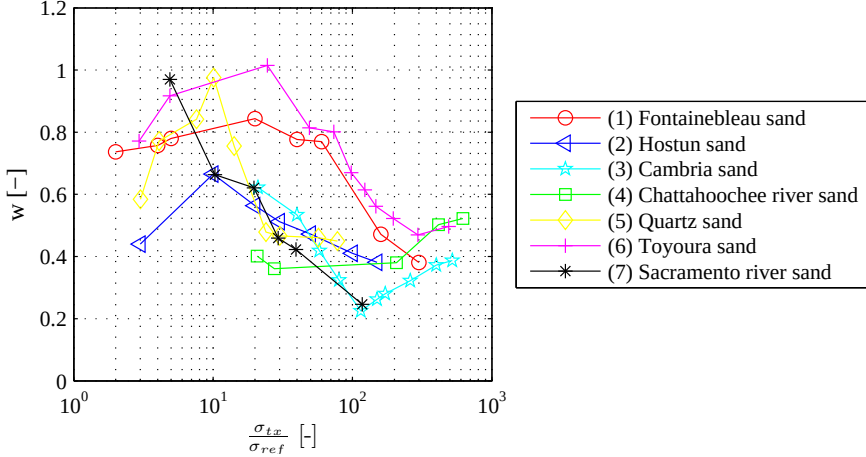
Figure 4.4: Dependency of exponent w (Equation 4.14) on cell pressure level for various granular soils under triaxial test conditions for sands listed in Table 4.1.
