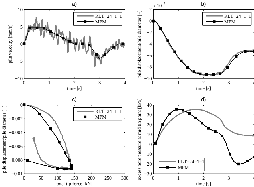
Figure 7.10: Comparison between centrifuge test and MPM for the first rapid load test RLT 24-1-1 (embedded pile with 1%D displacement)
