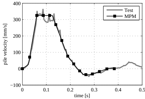
Figure F.1: Prescribed velocity applied on the pile head during rapid load test.
