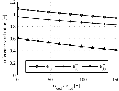
Figure 4.6: Dependency of reference void ratios on stress level (for Hostun sand, R_D = 90\% ).
