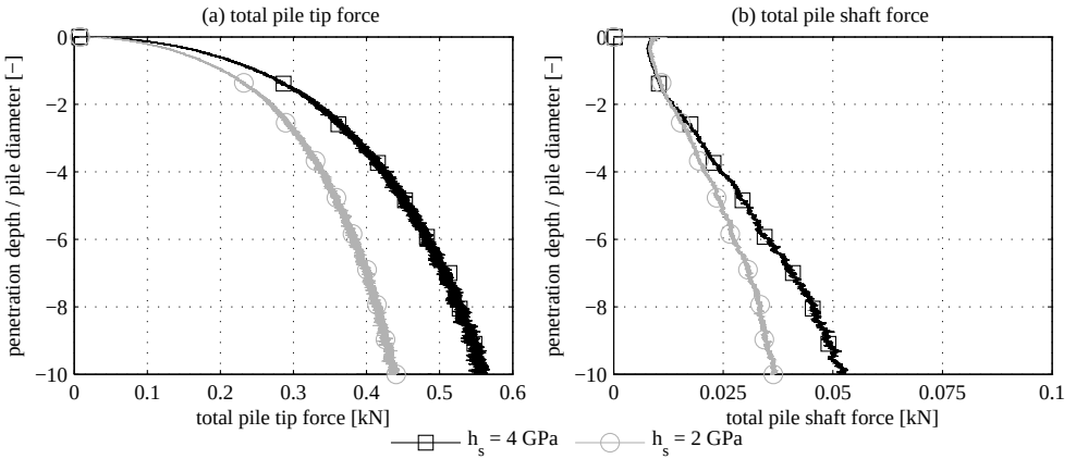
Figure D.6: Influence of h_s on analysis results.
