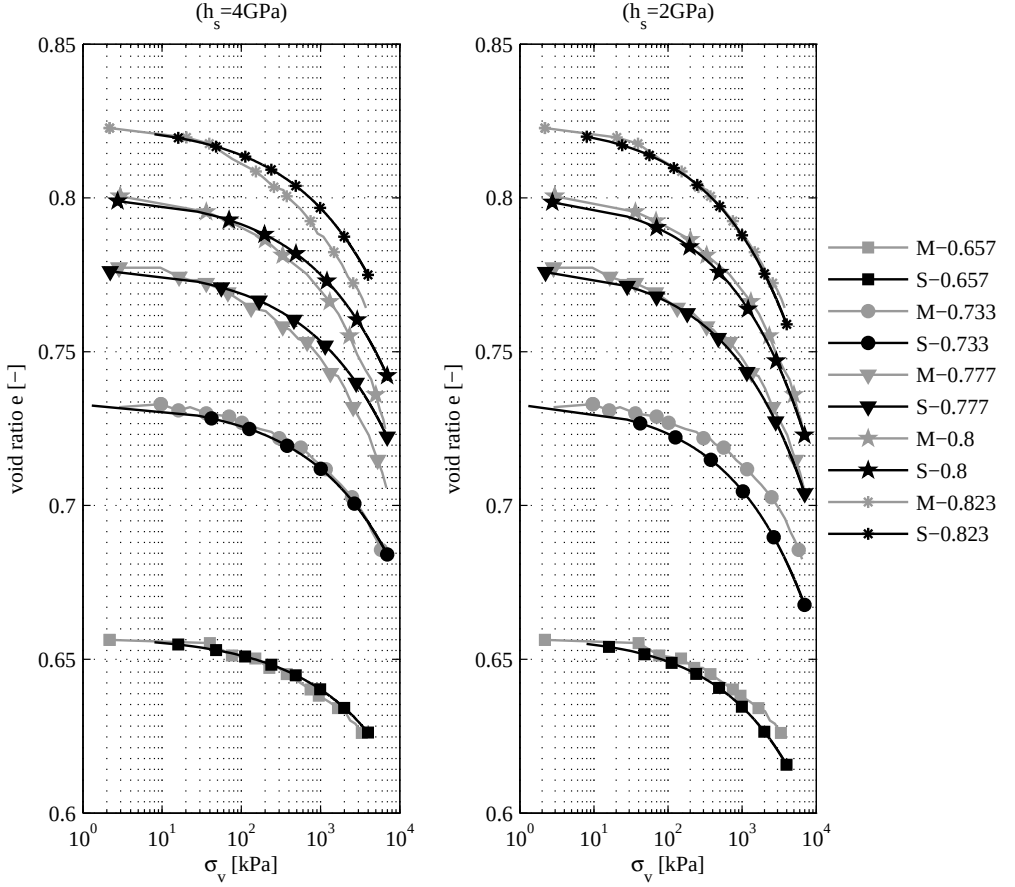
Figure C.1: Oedometric test on Baskarp sand, comparison between measurement and simulation.
