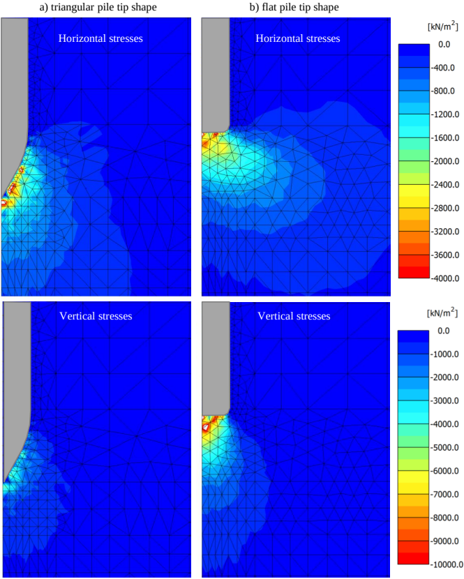
Figure 5.21: Vertical and horizontal stresses of soil around the pile tip after 10D penetration (simulation with loose sand and hypoplastic model).
