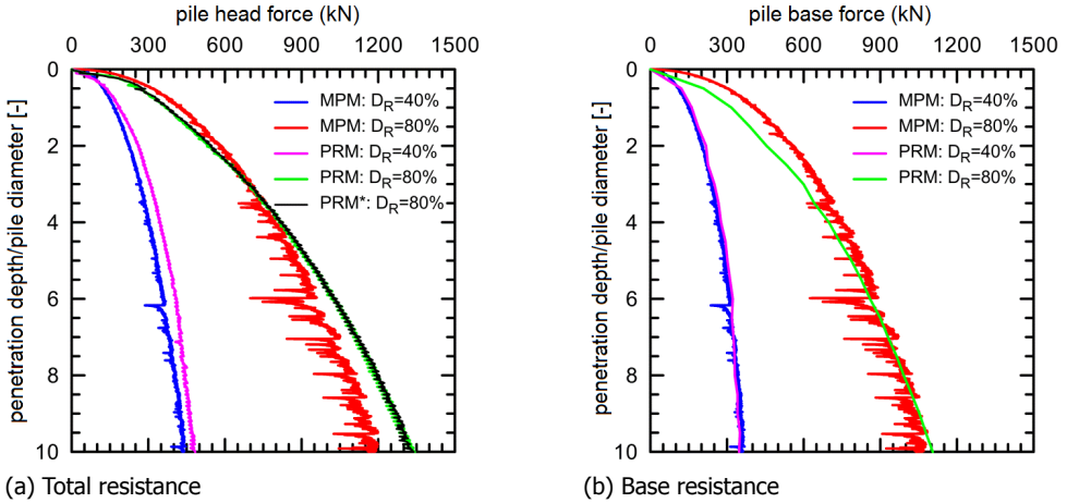
(a) Total resistance (b) Base resistance Figure 5.27: Penetration resistance during the pile installation (after [3]).
