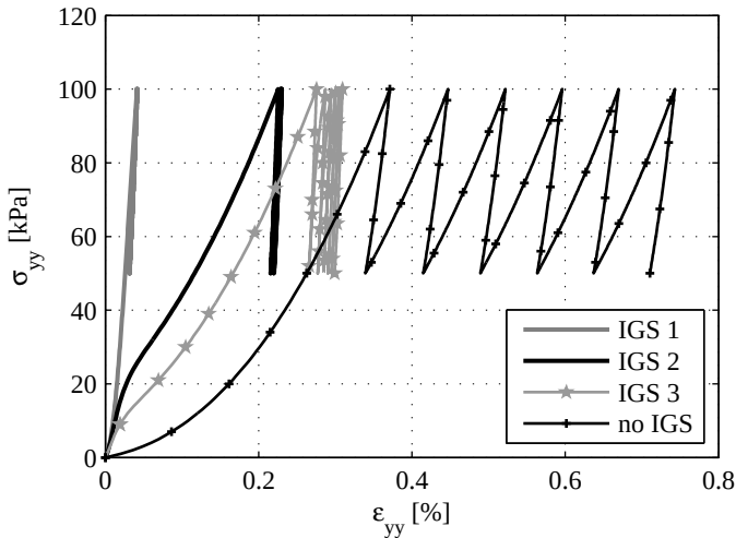
Figure C.4: Cyclic Odometric simulation on Baskarp sand with difference sets of small strain stiffness
