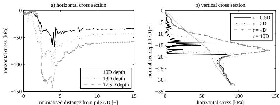
Figure 6.9: Calculated radial stresses after 6.5D pile penetration (150 blows) in saturated sand for different cross sections: a) horizontal cross section in different depth from the soil surface, b) vertical cross section for different distances to axis of symmetric.
