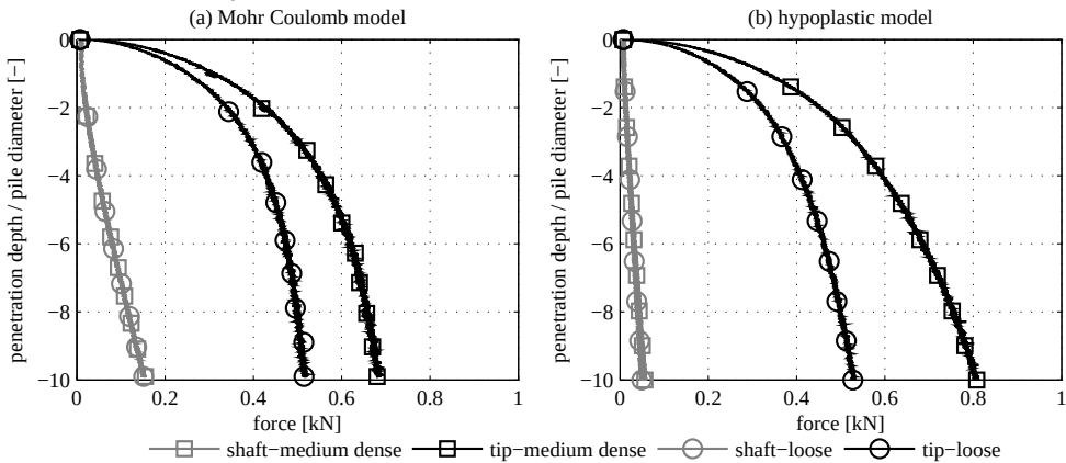
Figure 5.9: Total pile shaft and tip reaction curves obtained during installation for different densities. Comparison of Mohr Coulomb results and hypoplastic results.
