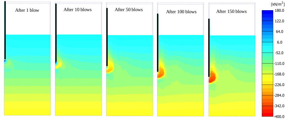
(c) pore water pressure
