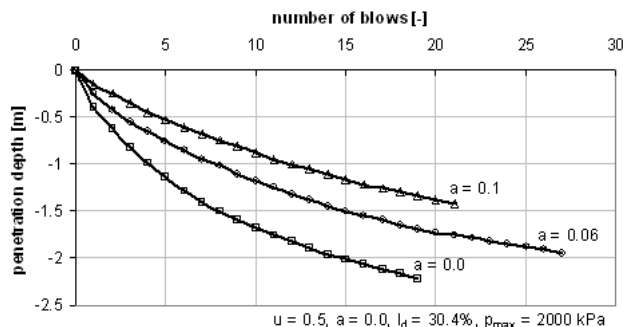
Figure E.1: Influences of damping on the load displacement curve.
