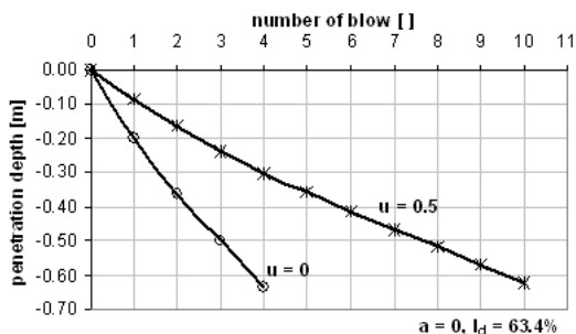
Figure E.2: Influences of skin friction on the load displacement curve.
