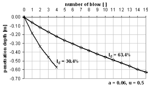
Figure E.3: Influences of sand density on the load displacement curve.
