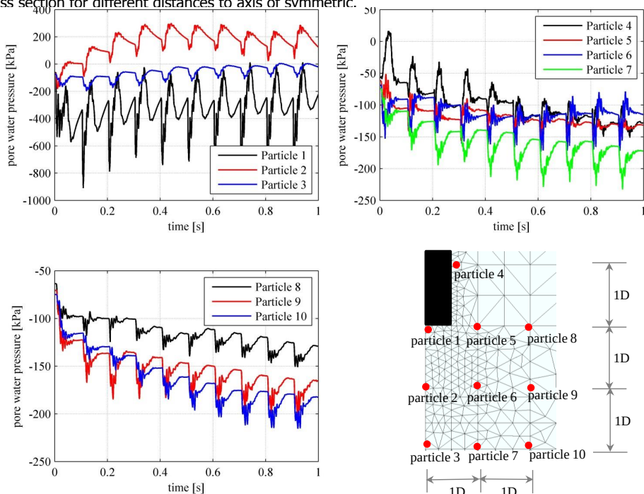
Figure 6.10: Developing of pore pressure during 10 blows for several particles around the pile tip.
