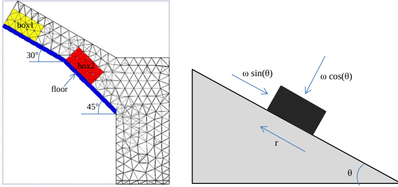
Figure 3.7: a) Geometry of sliding boxes problem generated for MPM calculation and b) forces acting on a sliding box [39].
