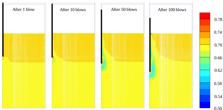
Figure 6.6: Calculated void ratio distribution around the driven pile after 1 blow, 10 blows, 50 blows and 100 blows.
