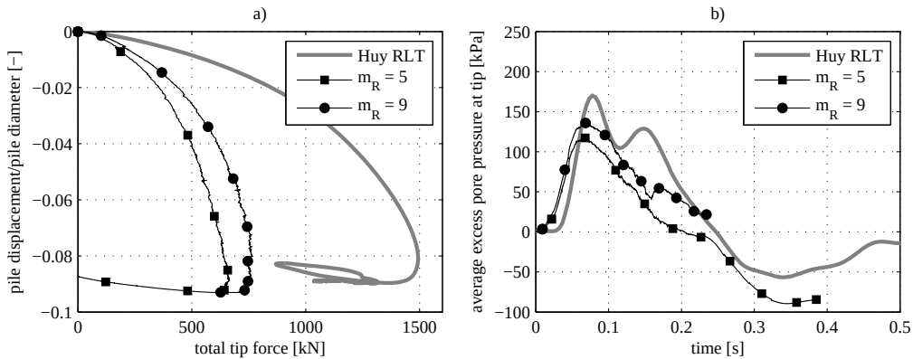
Figure F.4: Influence of different values of m_R , m_R = 5 , and 9 on the results of load-displacement curve during the rapid load test.
