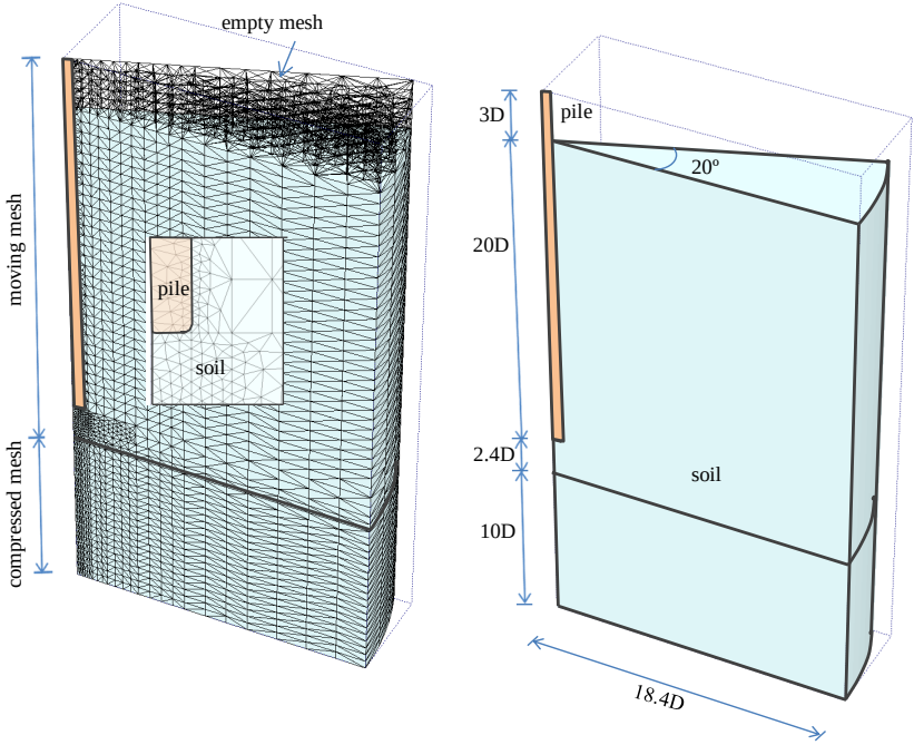
Figure 7.4: Mesh discretization and geometry of the considered problem for the pile without installation effects in Test 24.
