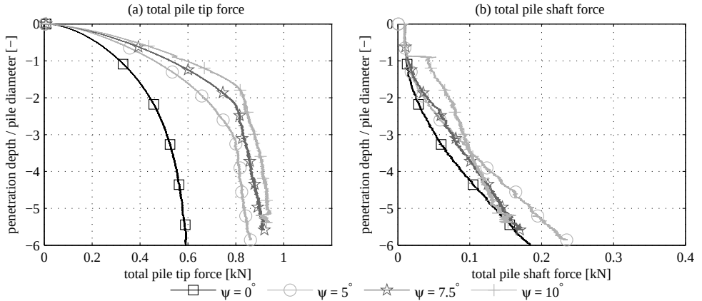
Figure D.5: Influence of dilation angle on analysis results. Simulations with Mohr-Coulomb model, E = 30 \text{ MPa} and \phi = 35^\circ .
