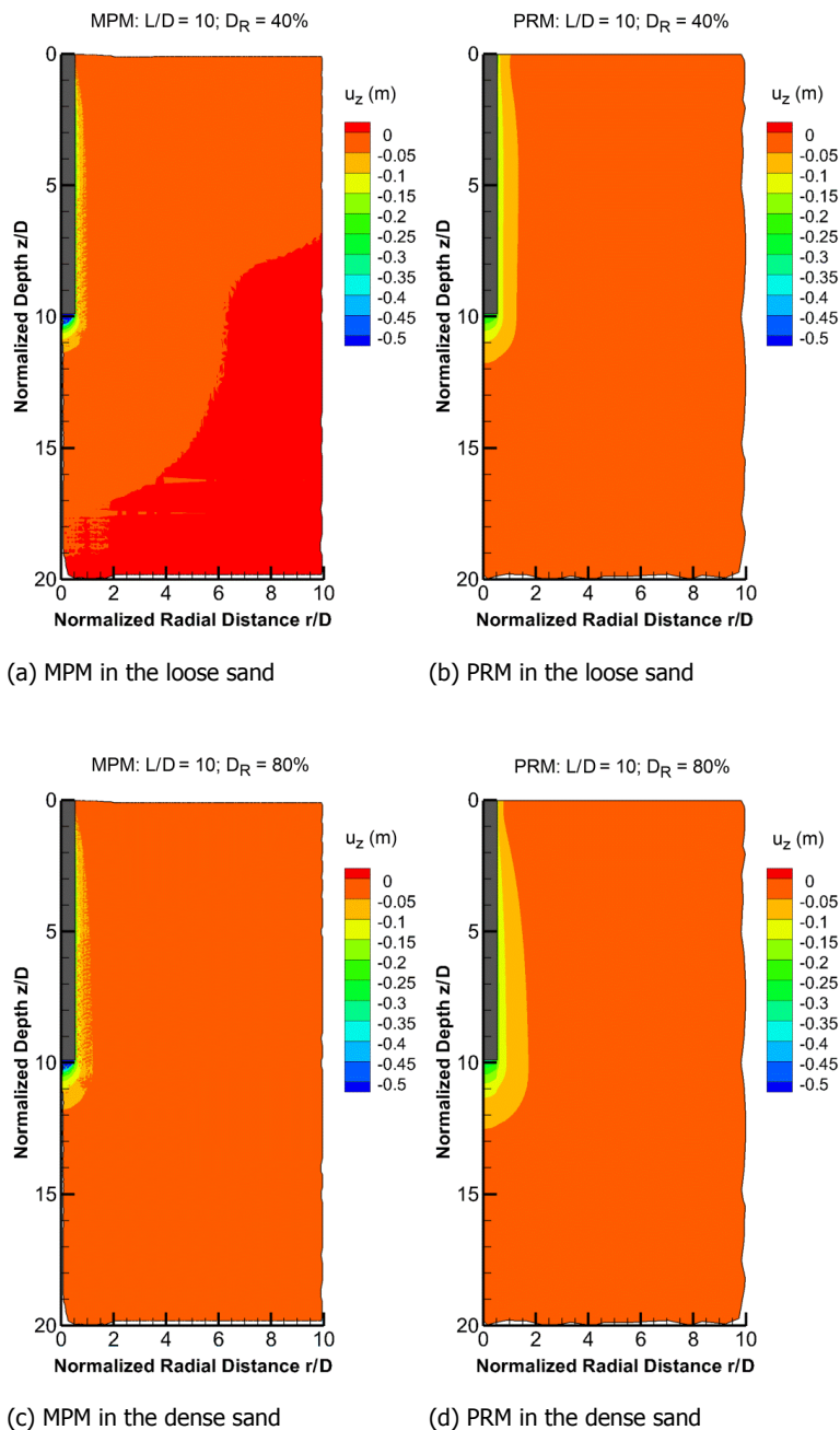
Figure 5.29: Vertical displacement after 10B pile penetration (after [3]).
