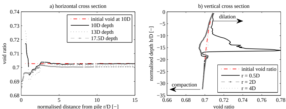
Figure 6.12: Cross section of void ratio after 6.5D pile penetration in saturated sand: a) horizontal cross section, b) vertical cross section.
