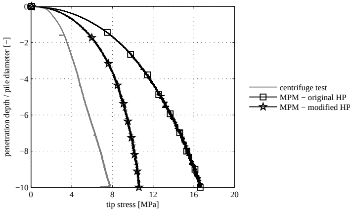
Figure 5.24: Evolution of stress under the pile tip during pile installation in medium dense sand ( R_D = 54\% ). Comparison of centrifuge test results and MPM simulation results using original and modified hypoplastic model.
