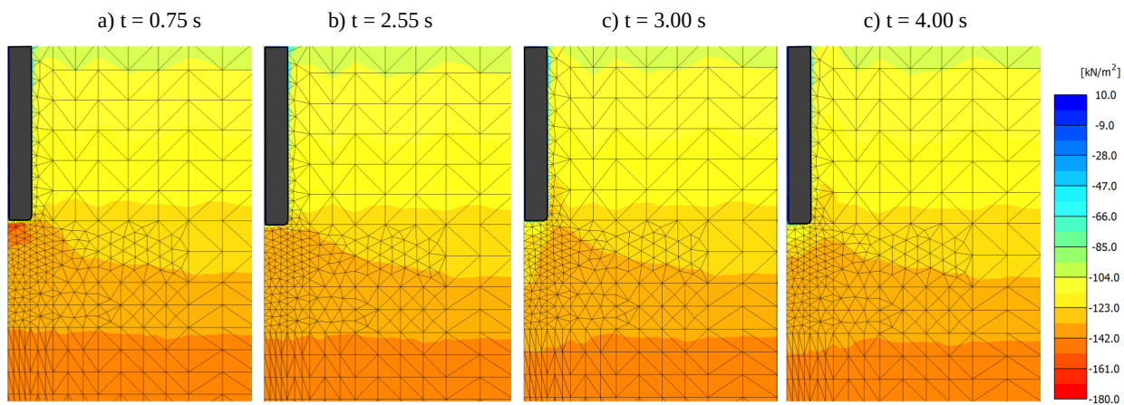
Figure 7.9: Pore water pressure around the pile tip at different time during RLT 24-1-1
