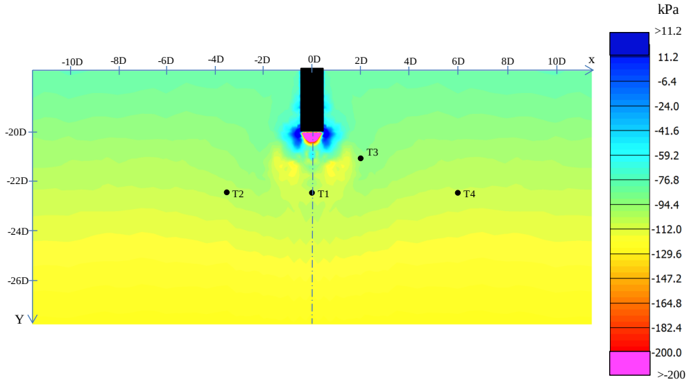
Figure 7.14: Pore pressure generated at time 4: t = 0.23 s in rapid load test for medium dense sand.
