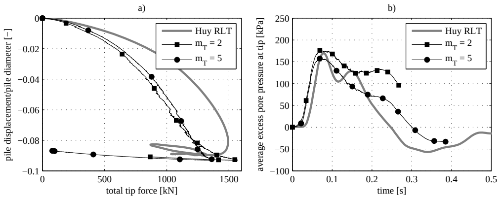
Figure F.5: Influence of different values of m_T , m_T = 2 , and 5 on the results of load-displacement curve during the rapid load test.
