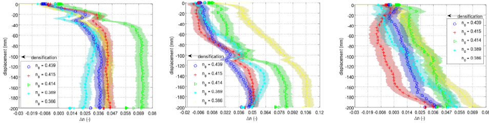
(a) instrument level 1, base (b) instrument level 1, mid (c) instrument level 1, upper Figure 2.10: Change in porosity during pile installation for different initial conditions at different measurement locations (after [3]).
