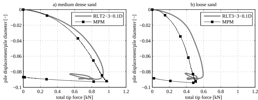
Figure 7.13: Comparison between centrifuge test and MPM for a) medium dense sand and b) loose sand.
