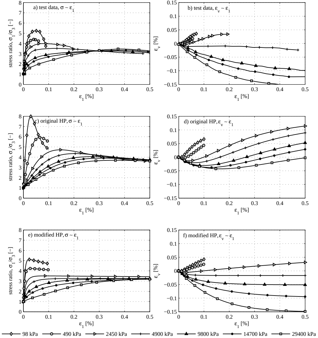
Figure 4.11: Triaxial response of Toyoura sand at cell pressures between 98 kPa and 29400 kPa, a) and b) are test results [13], c) and d) are simulation results using original hypoplastic model, e) and f) are simulation results using modified hypoplastic model.
