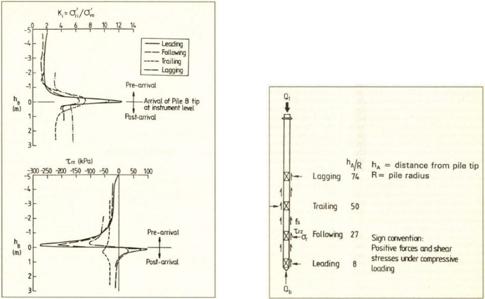
(a) stress measurement against h_B (b) The instrumented pile Figure 2.7: Normalised radial effective stress and shear stress of the first pile against location of the second pile [15].
