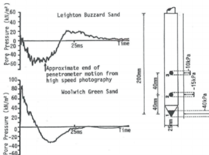
Figure 2.15: Changing of pore pressure during 1 blow at location 1 for Leighton Buzzard sand and Woolwich Green sand [29].
