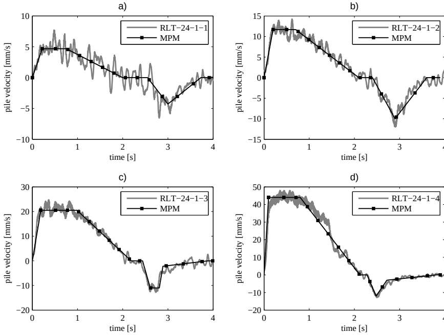
Figure 7.5: Prescribed velocity on the pile head during rapid load tests for wished in place pile with pile displacement of a) 1% D , b) 2% D , c) 5% D , d) 10% D .
