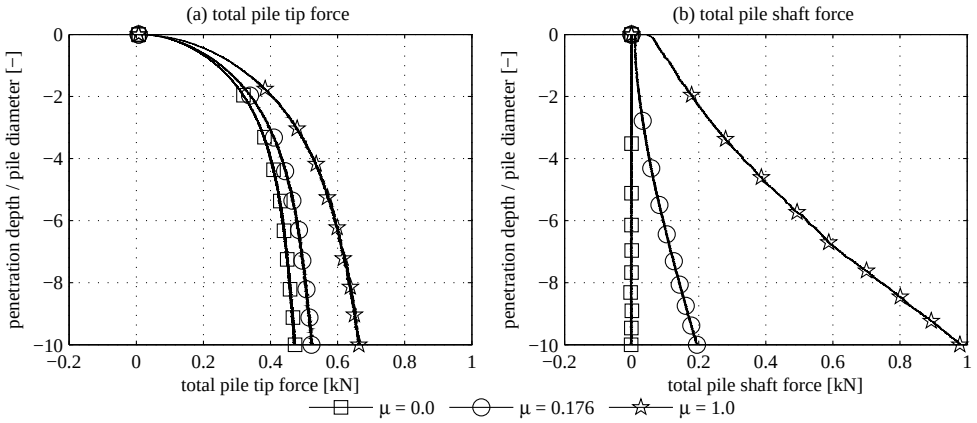
Figure D.2: Influence of coefficient of friction of contact \mu on analysis results. Simulations with Mohr-Coulomb model, E = 22 \text{ MPa} , \varphi = 30^\circ and \psi = 0^\circ .
