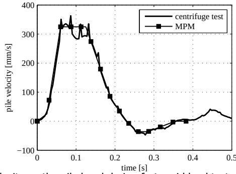
Figure 7.12: Prescribed velocity on the pile head during fast rapid load tests for jacked pile.
