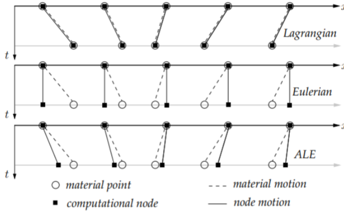
Figure 2.17: One-dimensional illustration of Lagrangian, Eulerian and ALE motions[66].
