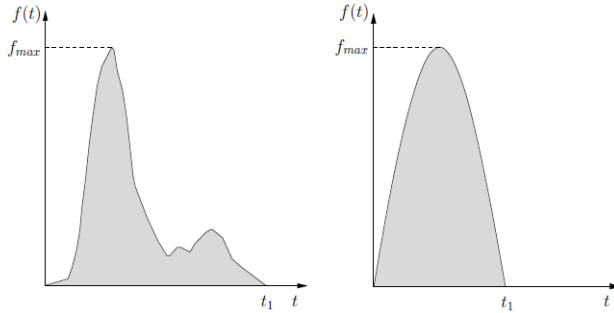
Figure 6.2: The forcing function for pile driving: (left) measured [19] and (right) the approximation to haversine time distribution [5]
