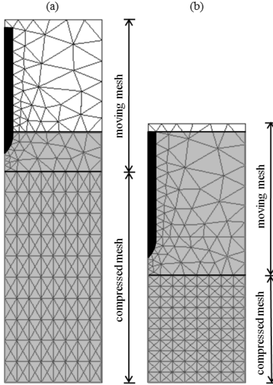
Figure 3.9: Concept of moving mesh for the pile driving problem: a) initial configuration, b) after pile penetration
