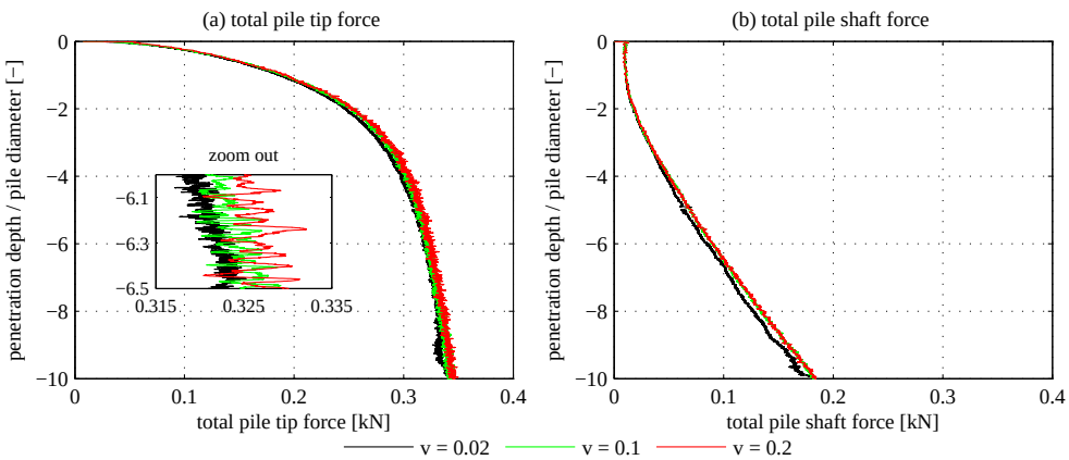
Figure D.1: Influence of installation velocity on analysis results. Simulations with Mohr-Coulomb model, E = 20 MPa, \varphi = 30^\circ and \psi = 0^\circ .
