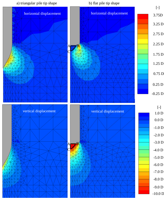
Figure 5.20: Displacement of soil around the pile tip after 10D penetration (simulation with loose sand and hypoplastic model).
