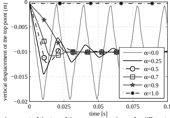
Figure 3.4: Vertical displacement of the top of the compression beam for different values of local damping \alpha
