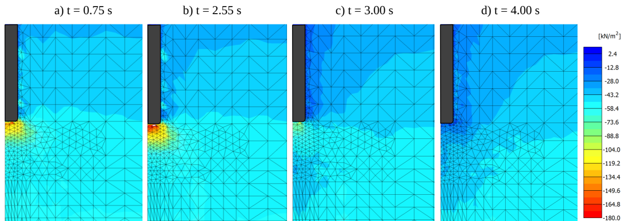
Figure 7.7: Horizontal effective stress around the pile tip at different time during RLT 24-1-1
