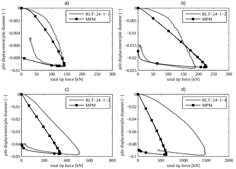
Figure 7.11: Load displacement curves during four rapid load test; comparison between centrifuge test and MPM for the pile without installation effect with pile displacement of a) 1% D , b) 2% D , c) 5% D , d) 10% D .
