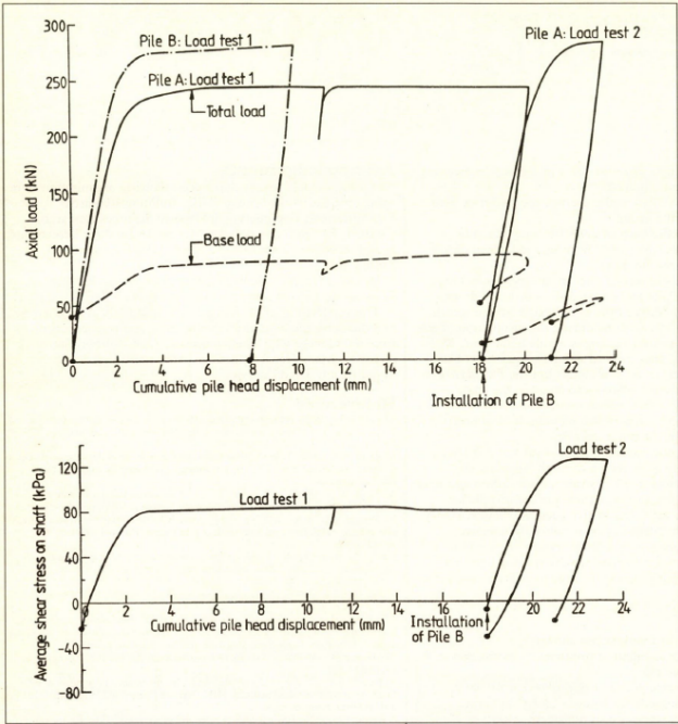
Figure 2.8: Pile tests on the first pile before and after installation of the second pile [15].
