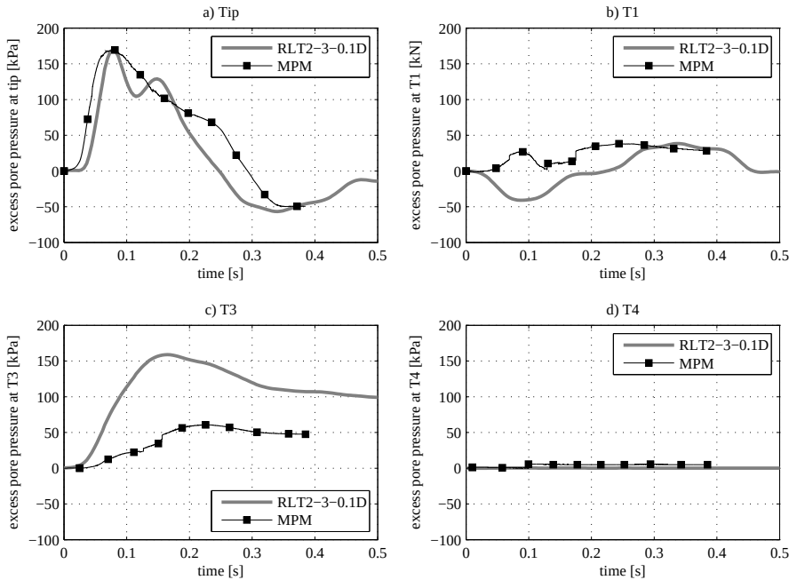
Figure 7.16: Pore pressure at different location during rapid load test for medium dense sand. Comparison between centrifuge test and MPM simulation.
