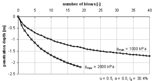
Figure E.4: Influences of driving pressure on the load displacement curve.
