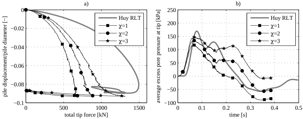
Figure F.2: Influence of different values of \chi , \chi = 1, 2 and 3 on the results of load-displacement curve during the rapid load test.
