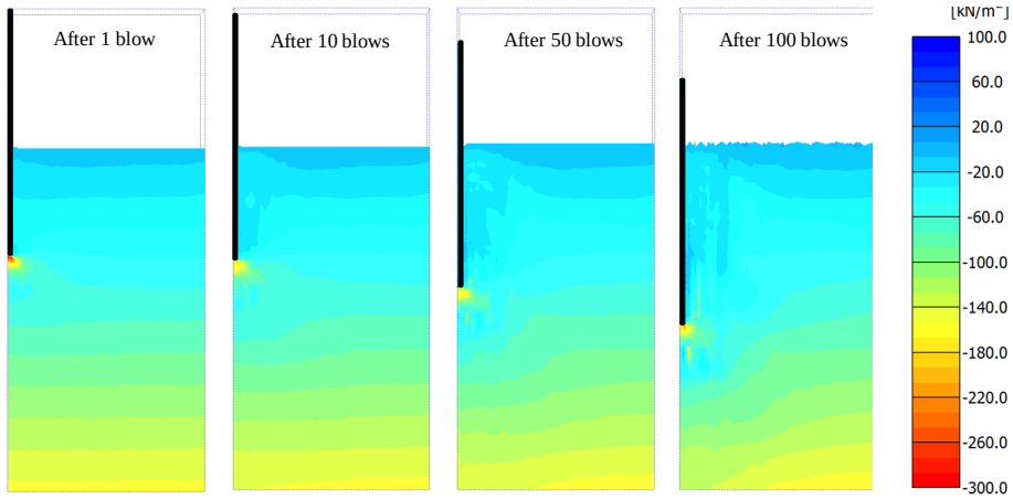
Figure 6.4: Calculated radial stress distribution around the driven pile after 1 blow, 10 blows, 50 blows and 100 blows.
