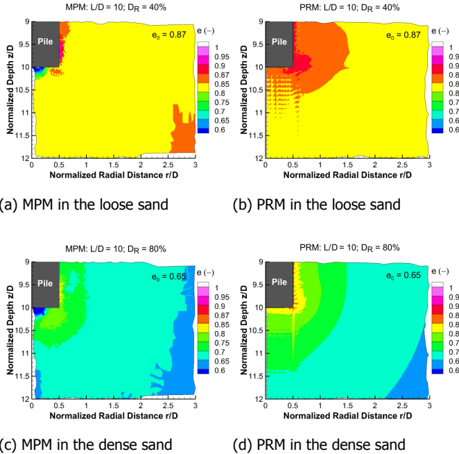
Figure 5.34: Void ratio around the pile base after unloading (after [3]).
