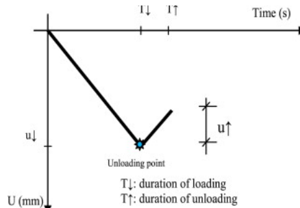
Figure 7.1: Displacement pattern of a rapid load test(after [7]).
