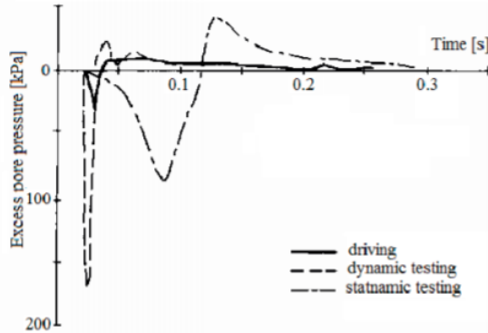
Figure 2.13: Behaviour of excess pore pressure during pile driving and loading [27].
