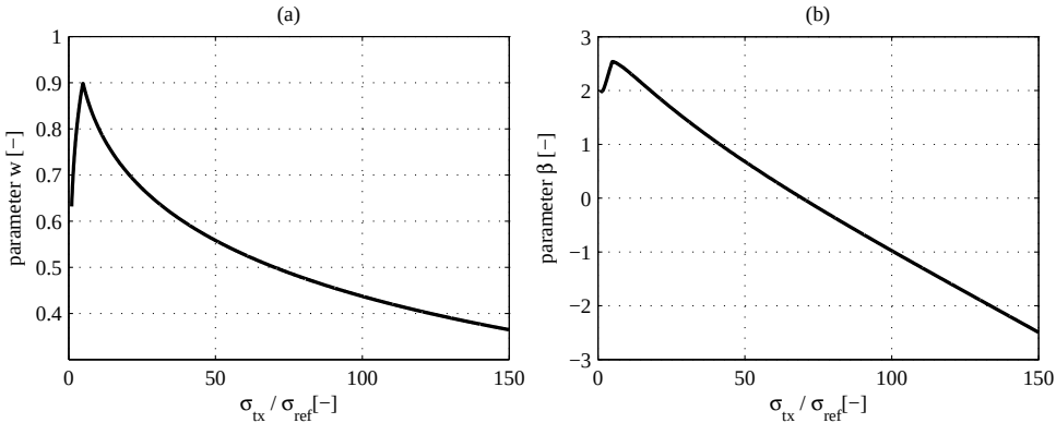
Figure 4.8: Relation between exponent \beta versus normalised stress p (for Hostun sand, R_D = 90\% ).
