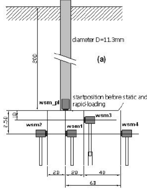
Figure 7.2: Positions of pore pressure transducers (after [7]). wsm_{pl} is the pore pressure transducer in the pile tip and wsm1 , wsm2 , wsm3 , wsm4 are the pore pressure transducers in the sand.
