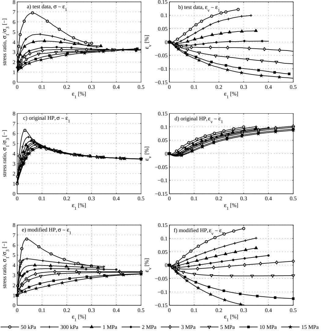
Figure 4.10: Triaxial response of Hostun sand at cell pressures between 50 kPa and 15 MPa, a) and b) are test results [12], c) and d) are simulation results using original hypoplastic model, e) and f) are simulation results using modified hypoplastic model.
