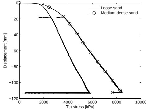
Figure 5.4: Change of stress under the pile tip during installation
