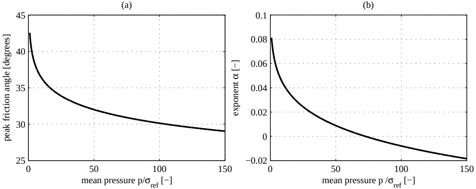
Figure 4.7: Relation between a) friction angle at peak \varphi_p versus mean pressure p and b) exponent \alpha versus mean pressure p (for Hostun sand, R_D = 90\% ).
