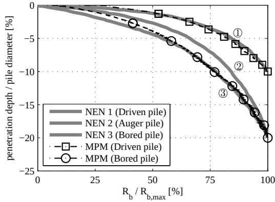
Figure 5.12: Comparing results of the design load test suggested by Dutch code (NEN 9997 – 2011) with MPM simulations ( R_b is effective stress of pile tip during SLT and R_{b,max} is effective stress of pile tip after SLT).
