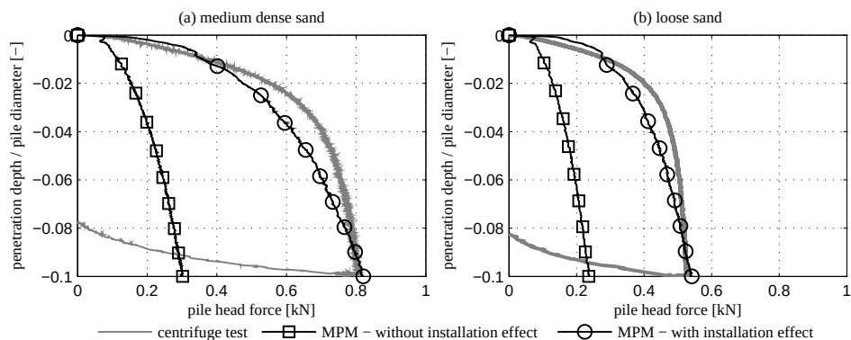
Figure 5.11: Load-displacement curve of the pile base during SLT for a) medium dense sand ( e = 0.68 , R_D = 54\% ) and b) loose sand ( e = 0.75 , R_D = 36\% ). Comparison of centrifuge test results and MPM simulations.
