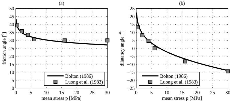
Figure 4.3: Comparison of triaxial test data on Quartz sand ( R_D = 95\% ) at high stress levels [3, 14]. a) relation between stress level and friction angle, b) relation between stress level and dilatancy angle.
