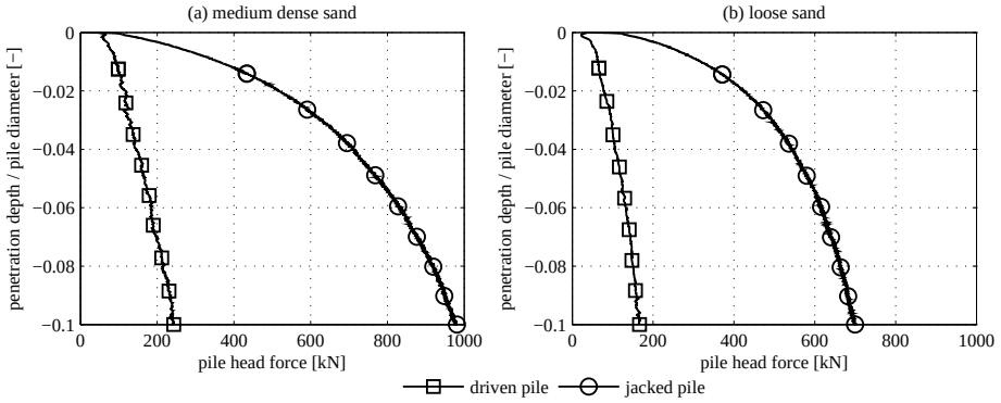
Figure 6.16: Load displacement curve during static load test. Comparison between jacked pile and driven pile for both loose and medium dense sand
