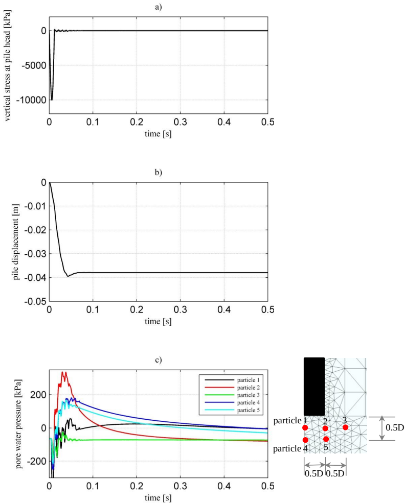
Figure 6.18: Measurement during first blow, a) vertical stress of the pile head vs time, b) pile displacement vs time, c) pore water pressure at different locations vs time.
