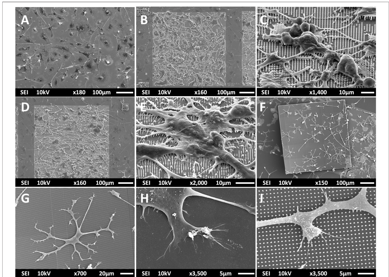
FIGURE 6 | SEM images of primary microglia on: (A) a flat fused silica substrate; (B,C) micro-pillar arrays; (D,E) NP1 nano-pillar arrays (pillars printed directly on the substrate); (F,G) NP2 nano-pillar arrays (pillars printed on a pedestal). Ramified microglia were noticed on both NP patterns, but pillars of NP2 had higher structural integrity compared to those on NP1 due to the support of the pedestal. Interaction of microglial filopodia with (H) the flat substrate; (I) nano-pillar arrays (NP2). (C,E) images are acquired at a 45° angle.
