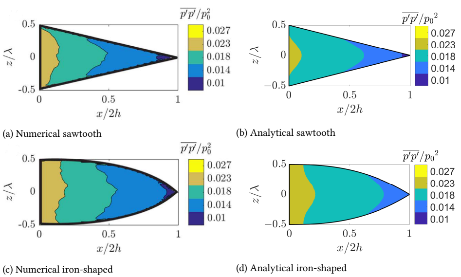
Figure D.1: Simulated distribution of the pressure fluctuations over the serration surface from the work of Avallone et al. (2017) [16] (a and c) compared against the predicted one (b and d). Figures a and b show the sawtooth serration geometry and c and d the iron-shaped serration geometry. Figures a and c are reprinted under the license number 5153050767352.
