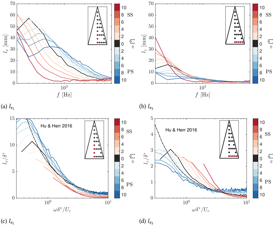
Figure 5.18: Variation of the stream (a and c) and spanwise (b and d) correlation length at the root of the serration with frequency and Strouhal number for different angles of attack ( Re = 2,000,000 ).
