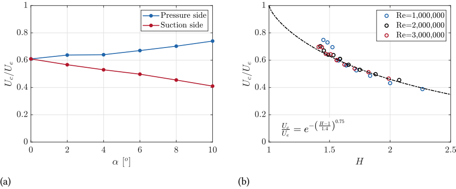
Figure 5.17: Measured convective velocity at different angles of attack at Re = 2,000,000 (a) and fitting of the convective velocity with the boundary layer shape factor, H (b).
