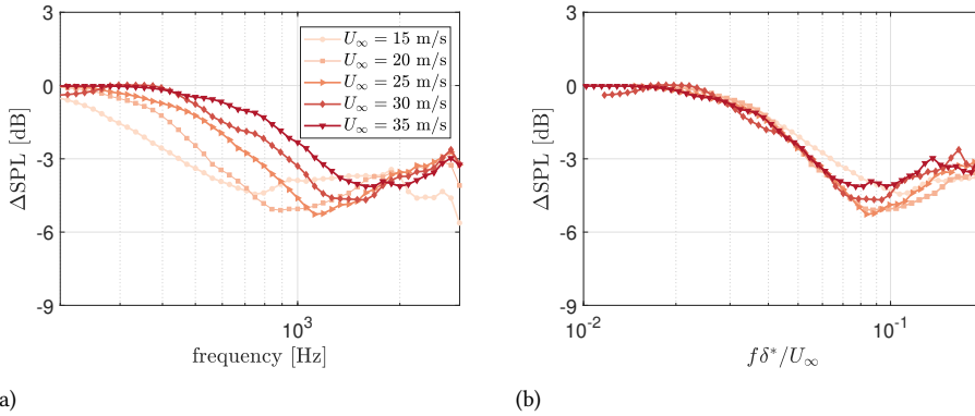
Figure 7.1: Measured noise reduction ( \Delta\text{SPL} ) obtained at different flow speeds at \alpha = 0^\circ . Figure (a) shows the noise reduction measured against the dimensional frequency, and (b) shows the noise reduction versus the non-dimensional frequency obtained using the boundary-layer displacement thickness.
