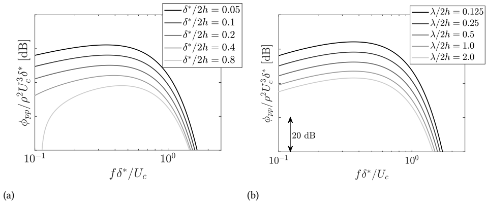
Figure 6.4: Predicted wall-pressure spectrum due to the presence of vortex pairs for different values of \delta^*/2h (a), and of \lambda/2h (b).
