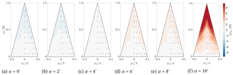
Figure 6.10: Distribution of the wall-pressure fluctuations over the serration surface measured on the suction side at different angles of attack, Re = 2 \times 10^6 and f\delta^*/U_c \approx 0.4 . Delta values are computed as the difference with respect to the pressure fluctuations measured by the sensor at the centre root of the serration ( x_1/2h = 0.10 , x_3/\lambda = 0.0 ) for each angle of attack.
