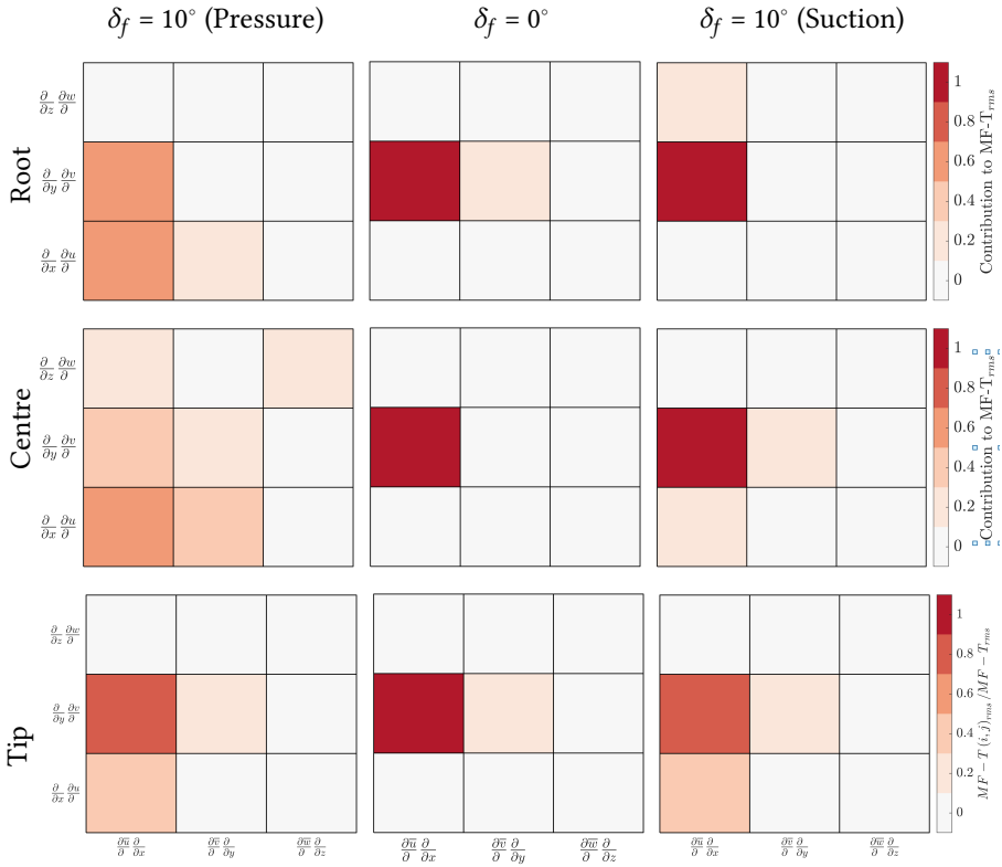
Figure 5.10: Relative contribution of the root-mean-squared of each component \frac{\partial \bar{U}_i}{\partial x_j} \frac{\partial u_j}{\partial x_i} to the mean shear-turbulence (MS-T) interaction term of the pressure Poisson equation estimated along the edges of the serration (one momentum thickness above the wall). Different flap angles, \delta_f = 0^\circ (b, e, and h) and \delta_f = 10^\circ on the pressure (a, d, and g) and suction sides (c, f, and i) are represented.
