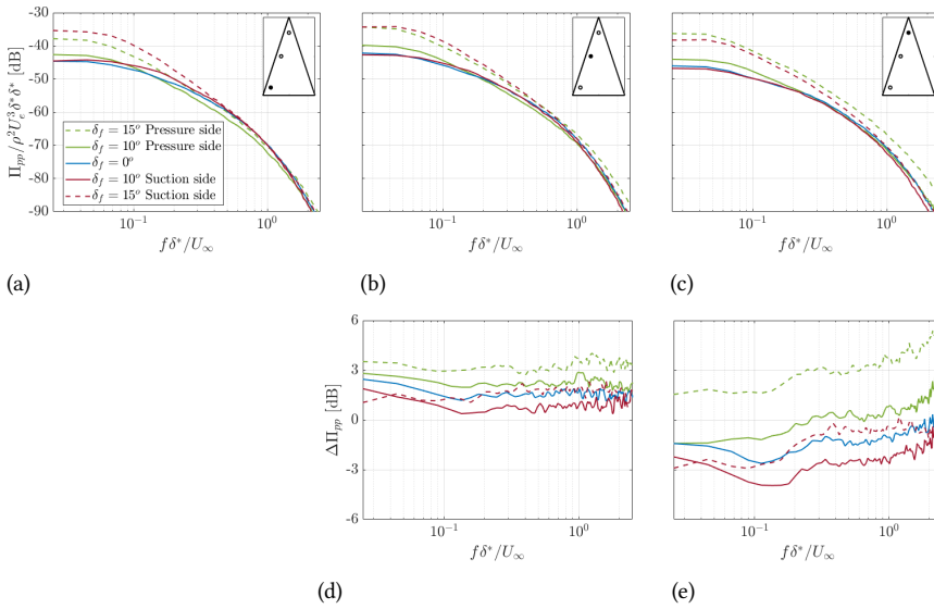
Figure 5.8: Variation of the scattering energy spectrum along the serratation edge and relative change in relation to the root ( x_1/2h = 0.1 ), at x_1/2h = 0.1 (a), x_1/2h = 0.5 (b and d), and x_1/2h = 0.8 (c and e).
