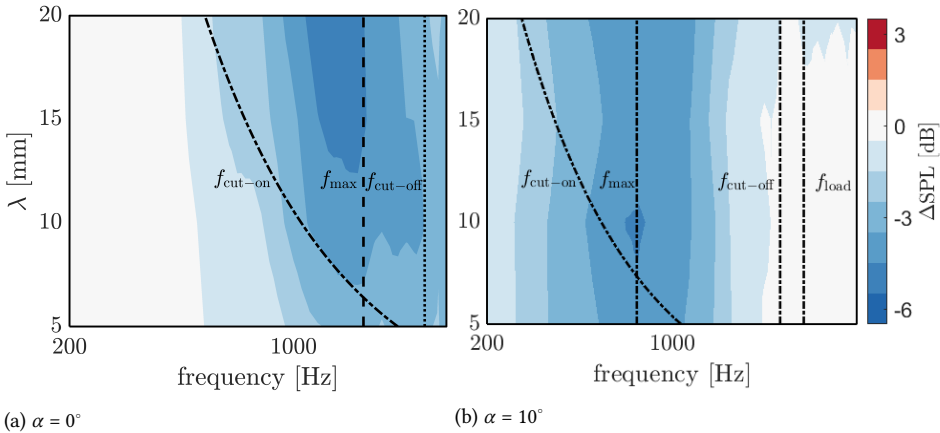
Figure 7.6: Contour plot of the variation of noise reduction for \alpha = 0^\circ (a), and \alpha = 10^\circ (b) at U_\infty = 30 m/s with the variation of serration wavelength while the height is kept constant ( 2h = 30 mm). Black lines show the theoretical predictions for the cut-on, max, cut-off, and loading noise frequencies.
