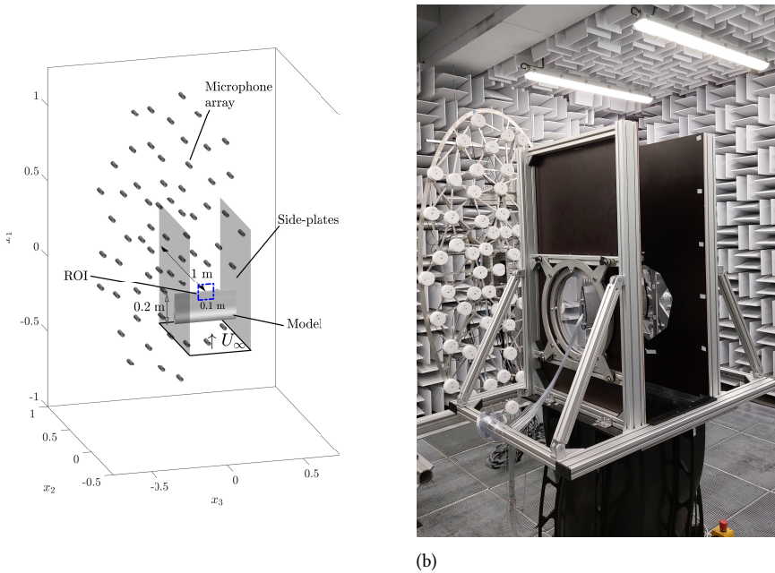
Figure 4.13: Experimental setup for acoustic measurements. (a) Schematic of the experiment, and (b) picture of the model mounted in the wind-tunnel facility.
