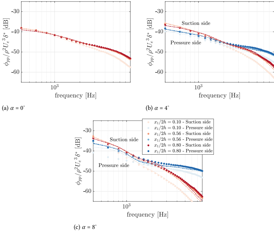
Figure 6.13: Comparison between measured \phi_{ppp} (circular marks) and predicted wall-pressure spectrum (dashed dotted lines) along the serration edge for three different angles of attack ( Re = 2 \times 10^6 ). Levels are made non-dimensional with respect to the boundary-layer displacement thickness at \alpha = 0^\circ . The analytical predictions are created using the spectrum at the centre and root ( x_1/2h = 0.1 , x_3/\lambda = 0.0 ) of the serration as reference.
