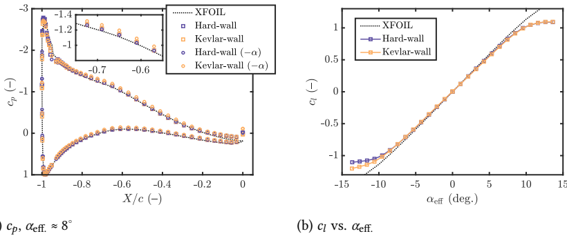
Figure 4.9: Comparison of c_p distribution (a), and c_l (b) from the LTT test with hard-walls and Kevlar-walls of the baseline NACA 633-018 airfoil at Re_c = 3 \times 10^6 .
