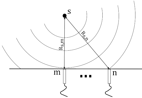
Figure 3.3: Illustration of the acoustic field created by a punctual monopole source at a distance R_s from an array of microphones.
