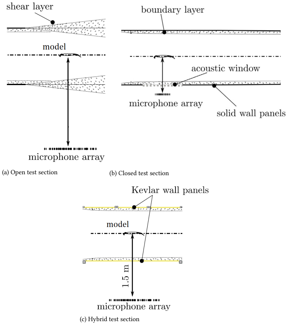
Figure 3.5: Illustration on the differences between the three test sections used for aeroacoustic measurements, i.e. open test sections (a), closed test sections (b), and hybrid test sections (c). Figure is adapted from [87].
