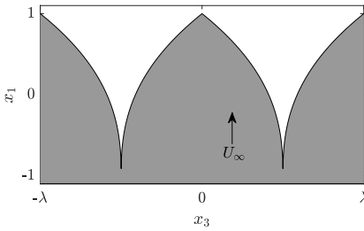
(a) Concave-shaped serrations
