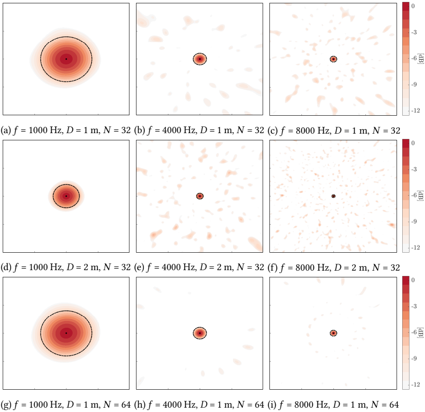
Figure 3.4: Acoustic source maps obtained at three different frequencies ( f = 1000, 4000, and 8000 Hz) for a monopole source at the centre of the map using three different array designs. a-c shows the source maps for an array with 1.0 m array diameter ( D ), and 32 microphones ( N ). d-f shows the source maps for an array with 2.0 m array diameter ( D ), and 32 microphones ( N ). g-i shows the source maps for an array with 1.0 m array diameter ( D ), and 64 microphones ( N ). Black dashed lines shows the expected beamwidth using equation 3.12.
