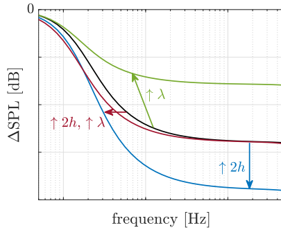
Figure 2.13: Example predicted variation of the noise reduction depending on the serration dimensions. The predictions are obtained with the rapid method from Lyu and Ayton 2020 [22]. The black line represents the reference noise reduction while the other lines illustrate the effect of different modifications of the serration geometry. Negative values of \Delta\text{SPL} indicate noise reduction.
