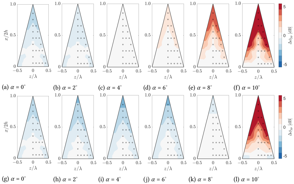
Figure 5.21: Wall-pressure fluctuations over the serration surface for f = 500 Hz at different angles of attack and Re = 2 \times 10^6 . Reference is set to the sensor at the centre root of the serration. Figures (a) to (f) shows the measured wall-pressure levels at the suction side and figures (g) to (l) at the pressure side.
