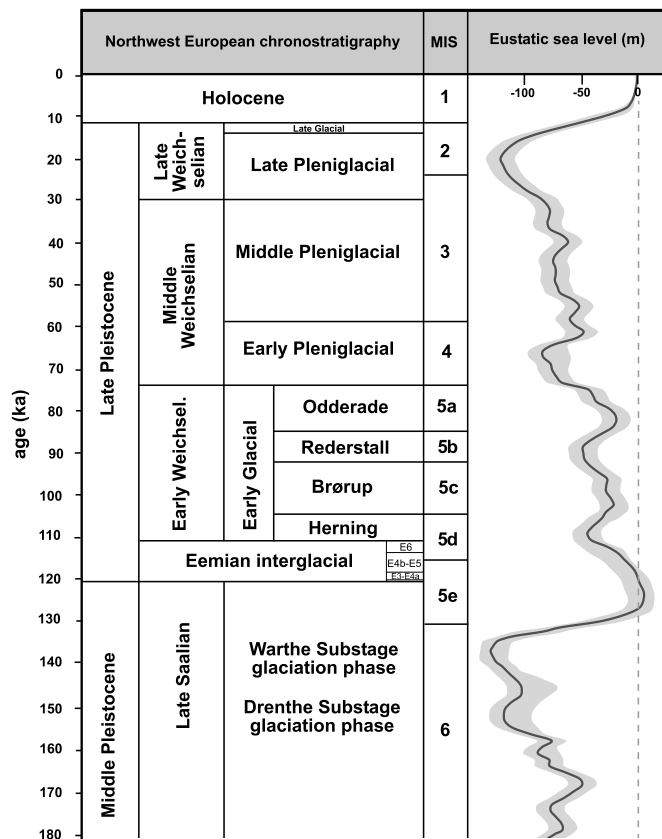
Fig. 2. Chronostratigraphic chart comprising the Northwest European sub-division of the late Quaternary (after Busschers et al., 2007; Peeters et al., 2015) updated with the latest insights regarding the timing of the Eemian in NW Europe (from Sier et al., 2015; Peeters et al., 2016). The composite eustatic sea-level curve (dark grey line) and associated confidence interval (light grey area) is from Waelbroeck et al. (2002) with adjustments after Medina-Elizalde (2013). Eemian pollen assemblage zones (PAZs) are indicated (cf. Zagwijn, 1961, 1996): the short 500-year interval of PAZs E1-E2 is not visualised. Correlations with the marine isotope record are based on Bassinot et al. (1994).
