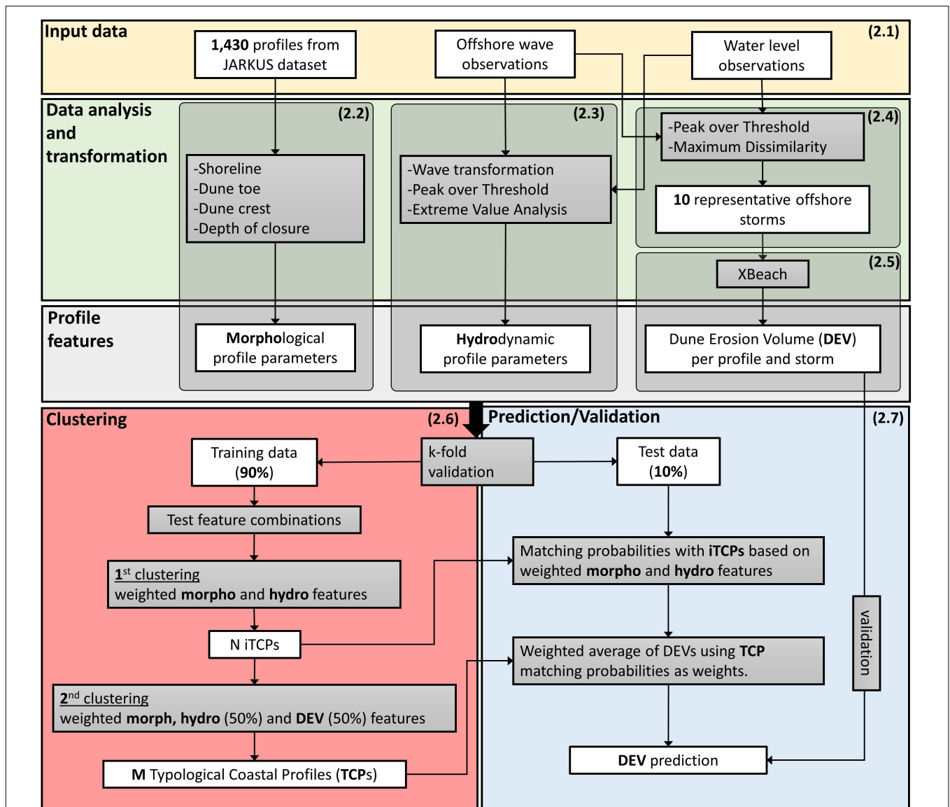
FIGURE 1 | Flow diagram of the methodology followed in the present study to reduce the initial dataset of Dutch coastal profiles to M typical coastal profiles (TCPs), based on their morphological, hydrodynamic and dune erosion characteristics, which were calculated using various observations, data analysis and modeling. The extracted TCPs were used to make predictions of dune erosion volume (DEV) for a set of test profiles using the simulated DEV as benchmark for the validation. Parentheses in top right corners of boxes indicate the section number that each part is described in.
