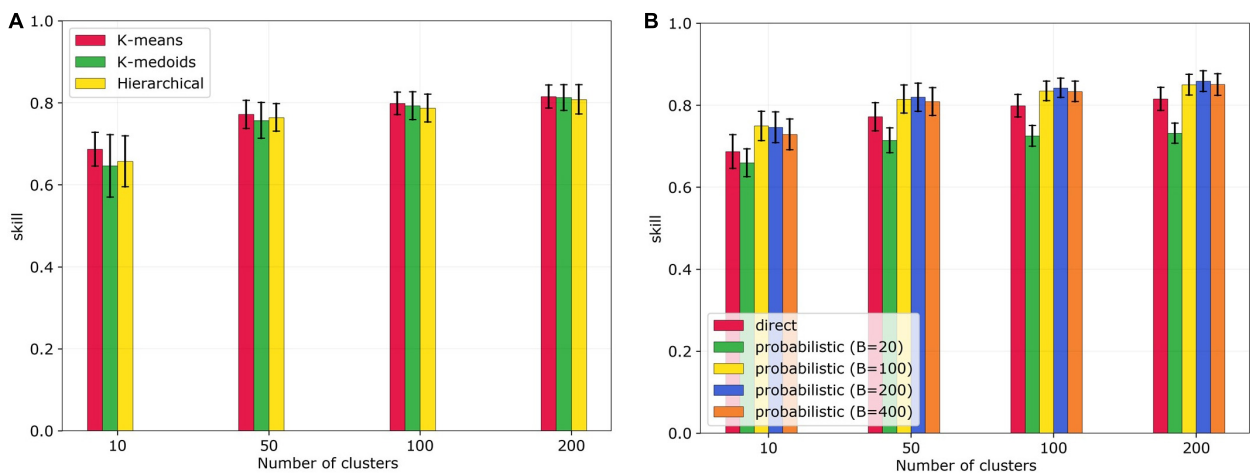
FIGURE 9 | Sensitivity analysis for clustering algorithms and matching methods. (A) Prediction skill for different clustering techniques and number of clusters, using the direct matching method. (B) Prediction skill for different matching methods (direct and probabilistic with different B values) and number of clusters, using K -means clustering. Bars indicate the mean values and lines the standard deviation of the 10-fold cross-validation.
