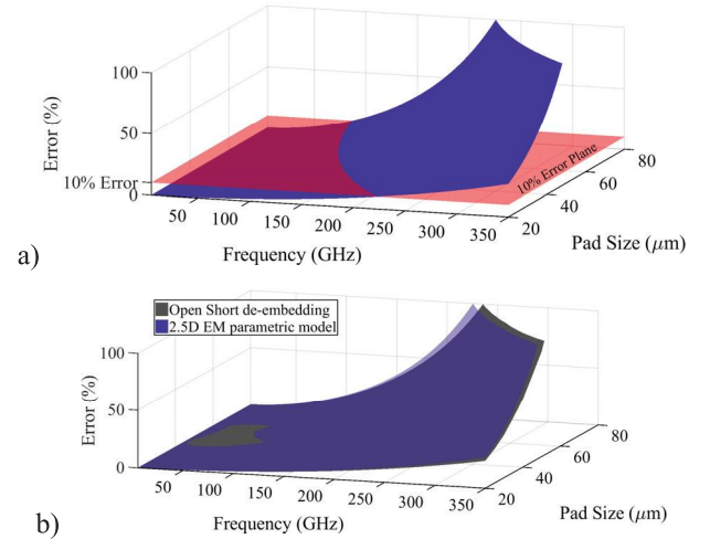
Fig. 4: Surfaces representing the C_{Ref} error using the CPWG circuit model for open-short de-embedding versus frequency and the varying (square) size of the pad (a) and a comparison to the deembedding error applying open-short elements extracted from 2.5D EM simulated pad/line fixture instead (b).
