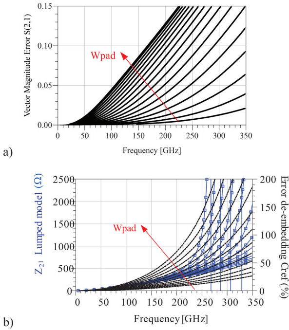
Fig. 6: a) Vector magnitude error of the lumped model versus CPWG representation of Fig. 2 with W_{pad} variation between 20 and 80 \mu m^2 . b) Magnitude of the Z_{21} parameter (blue) of the lumped fixture overlaid with the error of the extracted de-embedded C_{ref} (black).
