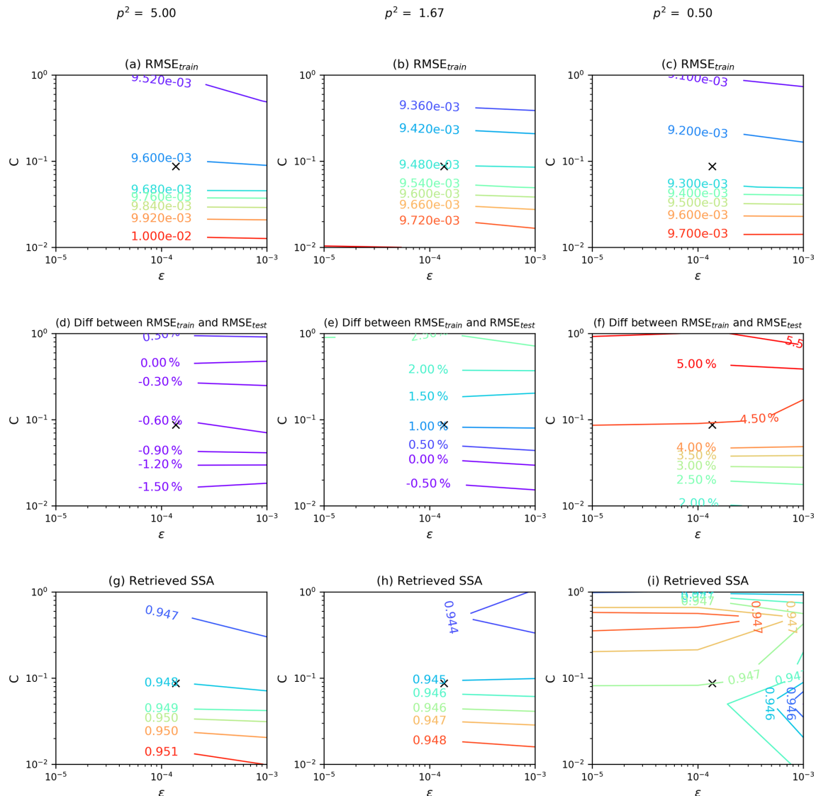
Figure 7. The performance of the SVR model as a function of hyper-parameters ( C , \varepsilon and p ). The cross markers represent the values of C and \varepsilon according to Cherkassky and Ma (2004). A p^2 value equal to 1.67 is sufficient to obtain a relatively high accuracy and also prevents overfitting of the training data set.
