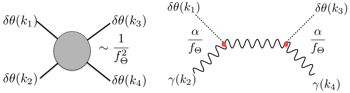
Figure 5. Left: four magnon scattering. In EFT, the amplitude can be calculated as shown in ref. [122]. As shown in ref. [118], it is the leading contribution to the magnon linewidth for T \sim T_N . For temperatures far below the spin wave mass, this term is Boltzmann suppressed. Right: feynman diagram for the s -channel of the process eq. (2.49) mediated by the axion term in the Lagrangian. The parametric dependence of the vertex factors is shown in red. This process is suppressed by two powers of \alpha compared to the four magnon amplitude, eq. (2.45).
