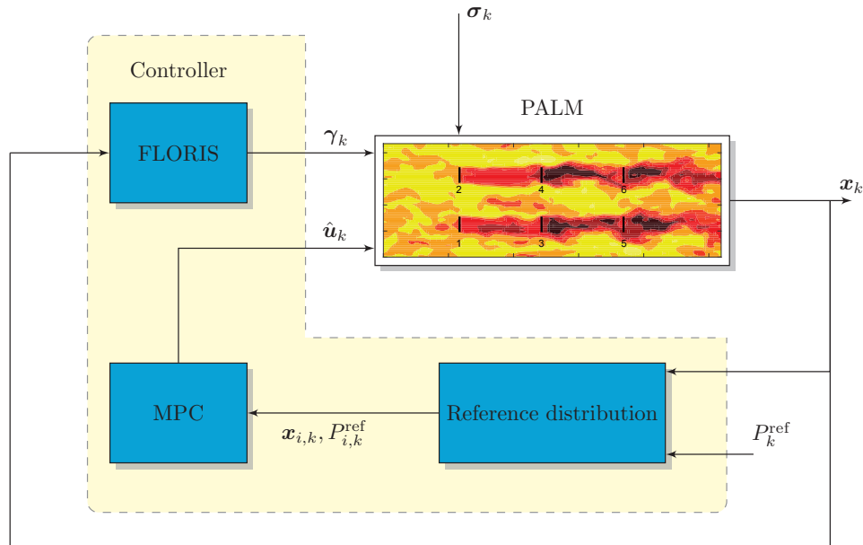
Figure 1: General idea of the closed-loop control framework with measurements x_k . The signals P_k^{\text{pref}} and P_{i,k}^{\text{pref}} are power reference signals for the farm and individual turbines, respectively. The control signals are the filtered thrust coefficients \hat{u}_k and yaw angles \gamma_k and \sigma_k the external wind farm perturbation such as, e.g. , boundary conditions.
