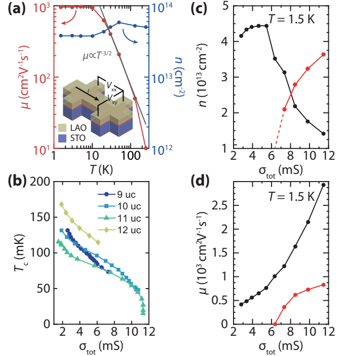
FIG. 2. (a) Carrier density ( n ) and mobility ( \mu ) as a function of temperature ( T ) measured for the pristine state. Inset: schematic representation of the measurement configuration. (b) Superconducting critical temperature ( T_c ) as a function of sample conductance ( \sigma_{\text{tot}} ) for different thicknesses of the LAO film. (c) Carrier densities and (d) mobilities as a function of \sigma_{\text{tot}} .
