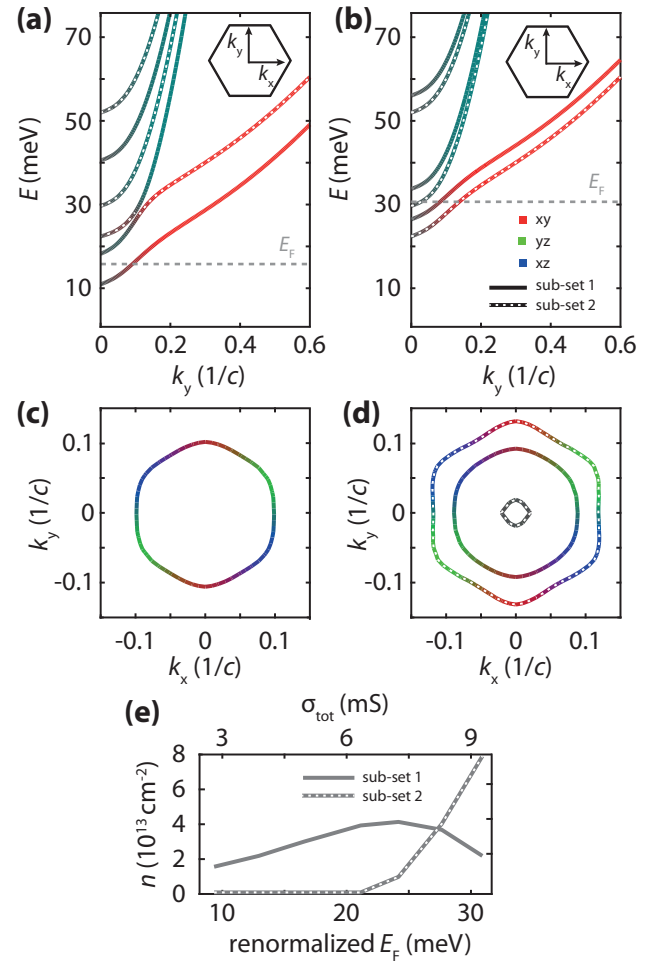
FIG. 3. (a),(b) Band structure along k_y at low and high filling, respectively. Dashed gray line indicates the renormalized Fermi level. Color indicates the orbital character. Stoke indicates the band subset. Inset shows the hexagonal Brillouin zone as well as the k_x ( \Gamma K ) and k_y ( \Gamma M ) directions. (c),(d) Corresponding Fermi surfaces. (e) Evolution of the carrier density pertaining to the first ( n_1 ) and second ( n_2 ) subset of bands as a function of renormalized Fermi level and respective sample conductance.
