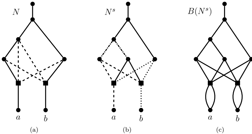
Fig. 5. (a) A non-binary tree-based network N on \{a, b\} . A base tree is indicated by the solid edges. (b) A semi-binary resolution N^s of N that is not tree-based with a cherry cover. (c) The bulged version of N^s that does not have a cherry cover. This can be seen as follows. There are four edges incident to the leaves and each of these edges can only be covered by reticulated cherry shapes. However, it is not possible to add four such reticulated cherry shapes without covering any middle edge of a reticulated cherry shape more than once.
