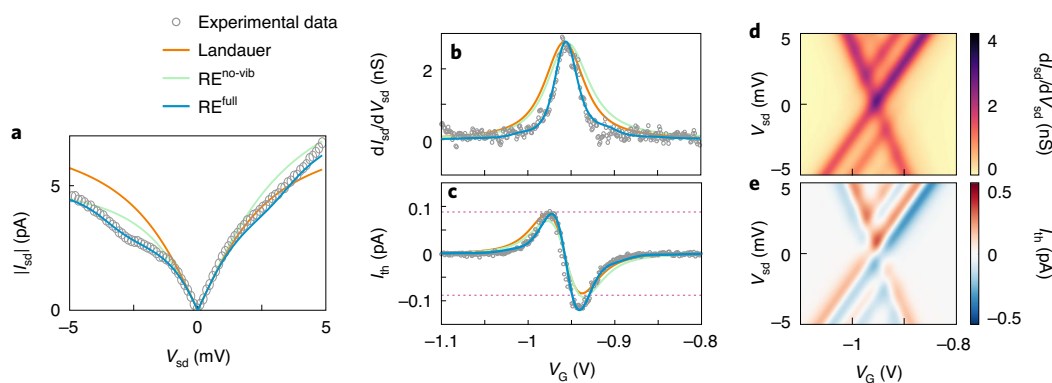
Fig. 3 | Comparison to theoretical model. a , I_{sd} – V_{sd} curve on resonance at V_G = -0.96 V. b , Gate-dependent zero-bias differential conductance. c , Thermocurrent extracted from Fig. 2. The grey circles show the experimental data, the solid lines show fits using a single-level Landauer approach (orange), a rate equation approach including spin entropy (green) and a rate equation approach including spin entropy and a vibrational mode (blue). The purple dotted lines in c indicate I_{th,max} . Calculated differential conductance ( d ) and thermocurrent ( e ) as a function of bias and gate voltage using the rate equation approach including spin entropy and a vibrational mode, and the parameters extracted from the fit in a .
