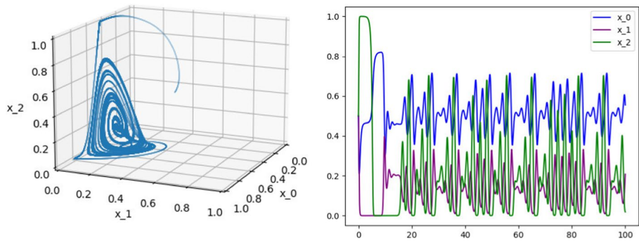
Fig. 5 A learning trajectory approaching a chaotic attractor in the polymatrix replicator [50] (left) and a plot of values of its coordinates (right). The game is characterized by unstructured interactions between payoffs and therefore breaks the assumptions of Theorems 3 and 4
