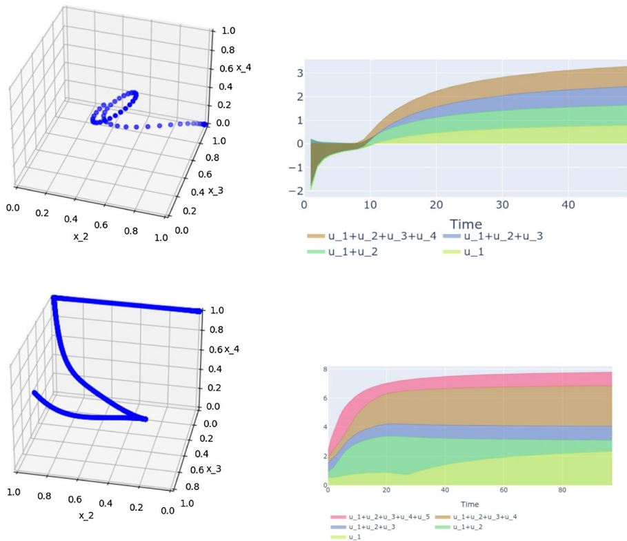
Fig. 3 Time-average payoffs and social welfare of a sample learning trajectory in the matched–misaligned pennies game (top), and in the asymmetric 5-penny game with p = 3 (bottom, projection onto first three variables)
