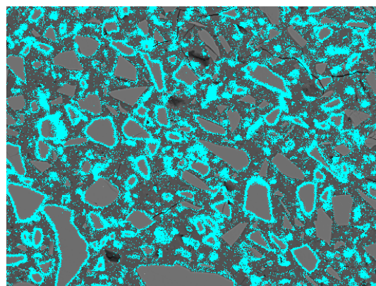
(c) BSE image with unselected pixels from density plot referring to NaMgAlSiCa gel.
