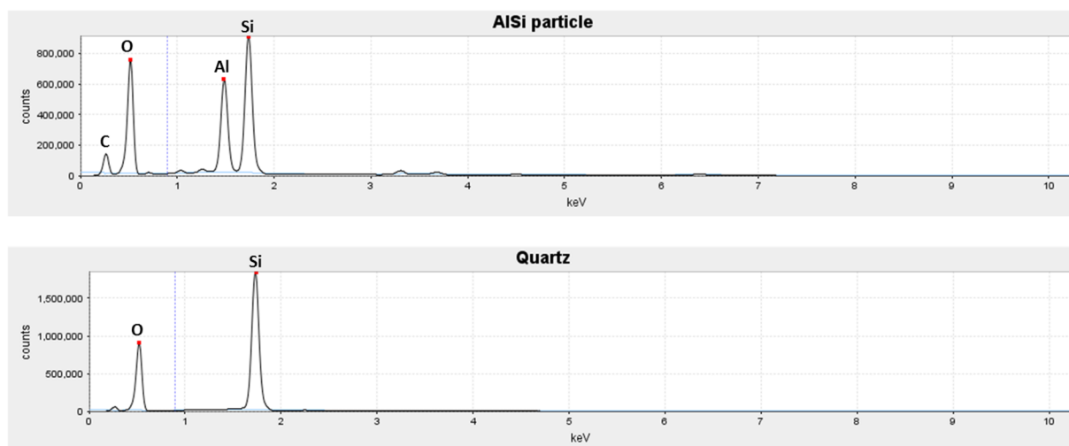
Figure 11. PARC sum spectra for AlSi pixels (blue coloured in the composite map, Figure 12) and Quartz ( \text{SiO}_2 , yellow coloured in the composite map, Figure 12), indicating the presence of O, Al, and Si by their characteristic X-ray lines.
