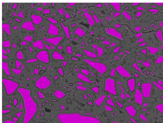
(b) BSE image with selected pixels from density plot referring to GBFS particles (image width = 250 μm).
