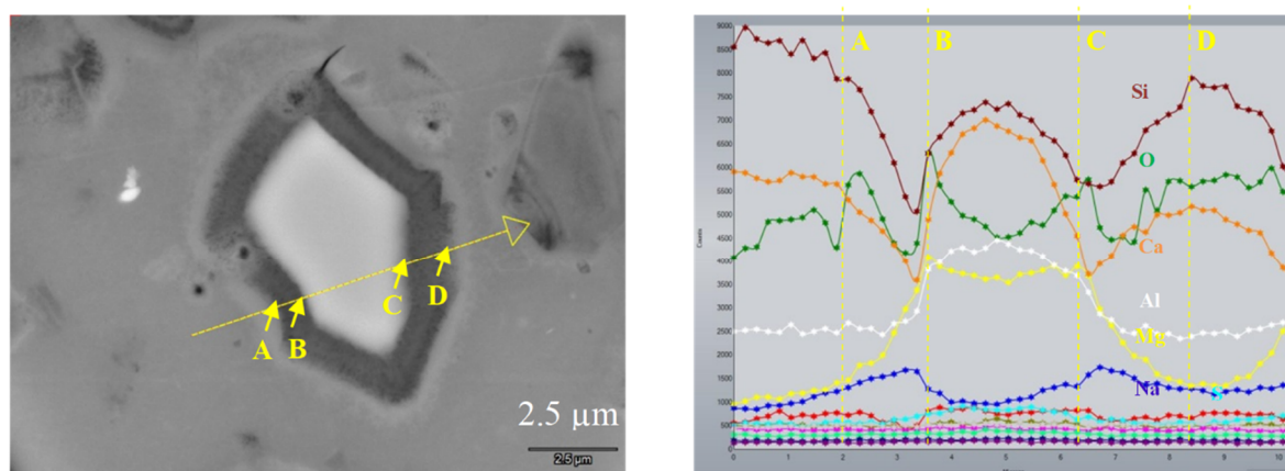
Figure 16. The BSE image of the microstructure around a reacted GBFS particle of the paste S100 after 1 year of reaction ( left ) and corresponding EDX linescan-profiles along the yellow arrow for the constituent elements (Si, O, Ca, Al, Mg, Na) ( right ).
