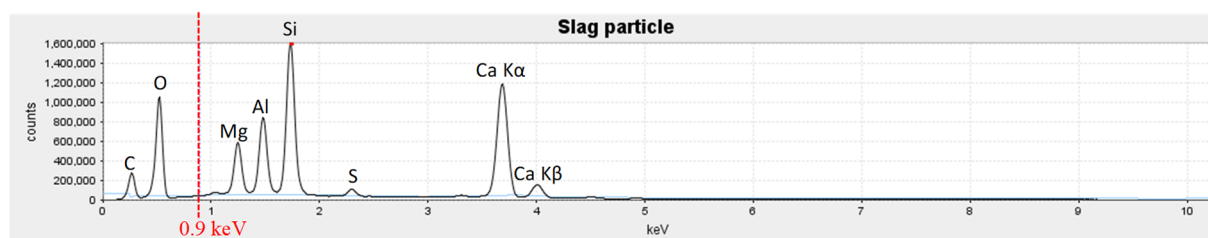
Figure 8. PARC sum spectrum for a GBFS particle (purple coloured in the PARC map, Figure 9), indicating the presence of Mg, Al, Si, S, and Ca by their characteristic X-ray lines.
