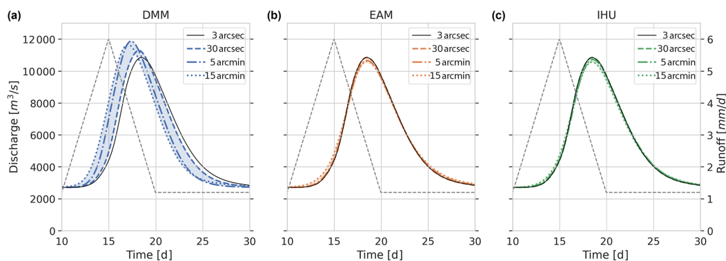
Figure 7. Simulated discharge at the river mouth of the Rhine near Rotterdam for a synthetic accumulated runoff event (grey line) and based on models with native 3 arcsec resolution flow directions (black line) in comparison to upscaled flow directions based on the DMM (blue; a), the EAM (orange; b) and IHU (green; c) at a 30 arcsec (dashed line), 5 arcmin (dash-dotted line) and 15 arcmin (dotted line) resolution. Note that the simulated discharges for the 30 arcsec EAM and IHU runs largely overlap with that of the native 3 arcsec run.
