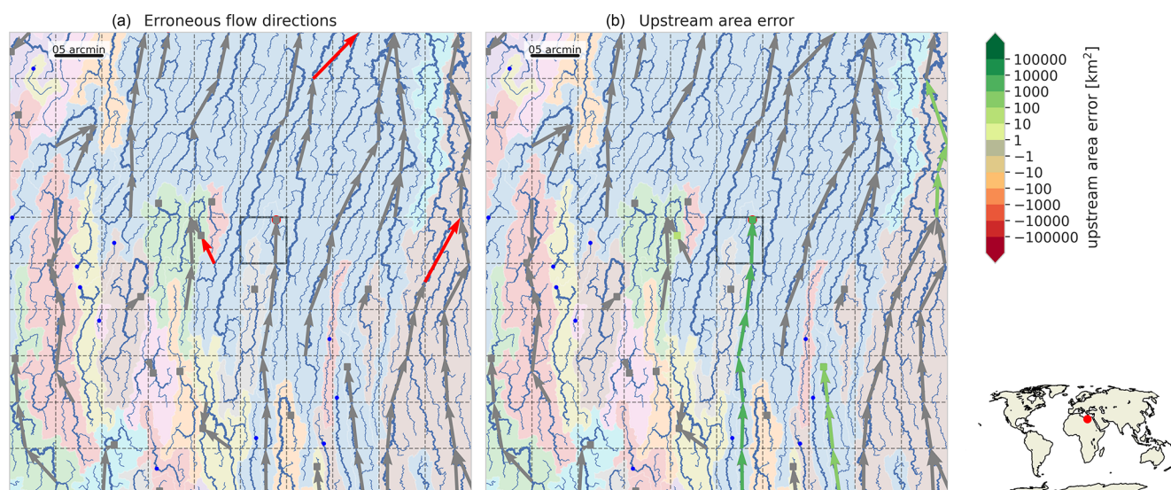
Figure C4. Largest basin ( 16\,717 \text{ km}^2 ) with a relative upstream area error of more than 10 % at the 5 arcmin resolution indicated with a highlighted cell. See the caption of Fig. C1 for a full description.
