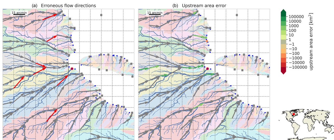
Figure C2. Largest exorheic basin ( 6830 \text{ km}^2 ) which is not resolved at the 15 arcmin resolution indicated with a highlighted basin outlet. See the caption of Fig. C1 for a full description.
