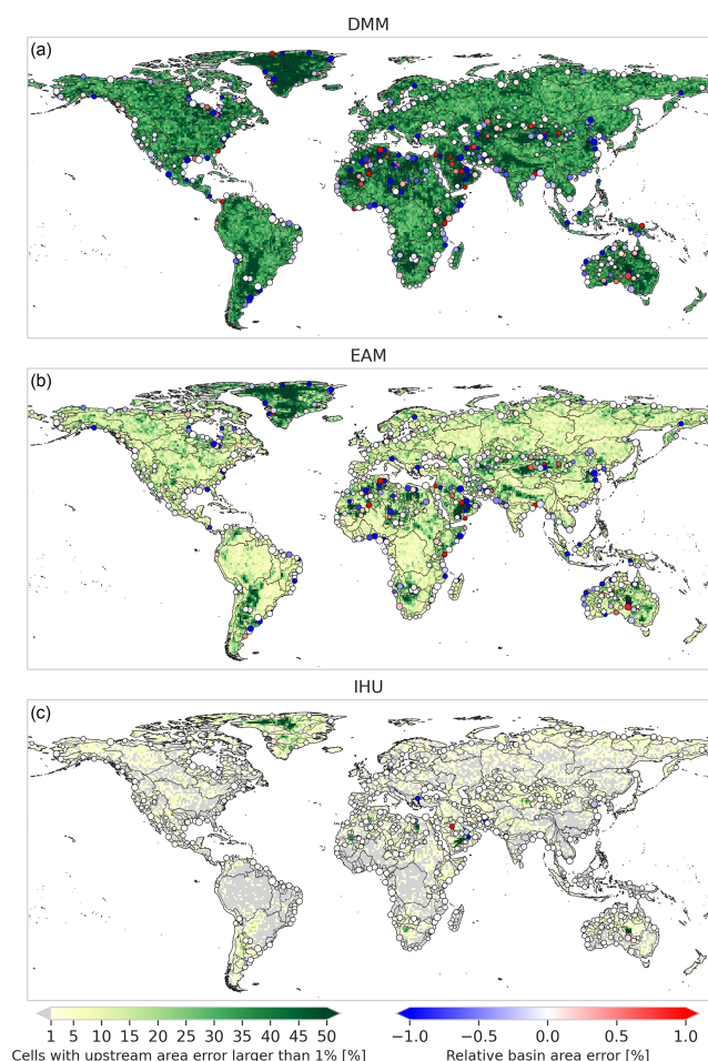
Figure 5. Relative upstream area error ( \epsilon_{\text{rel}} at a 5 arcmin resolution ( \sim 10 km)) for the DMM (a), the EAM (b) and IHU (c). The background colors show the percentage of cells per 1 \times 1^\circ tile with a relative upstream area error of more than 1 %, while the markers show the relative upstream area error at the outlets or sinks of the 500 largest basins globally (black lines).
