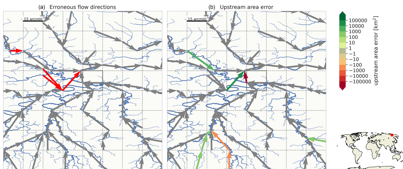
Figure C6. Second-largest local upstream area error ( -220\,876\text{ km}^2 ) at the 15 arcmin resolution indicated with a highlighted cell. See the caption of Fig. C1 for a full description.
