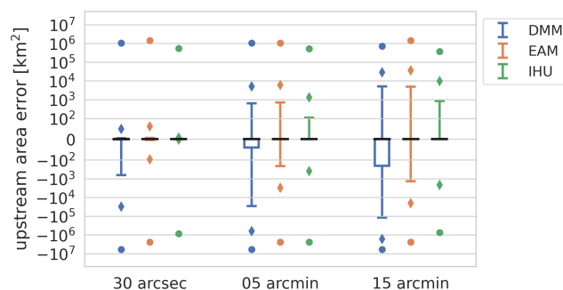
Figure 4. Absolute upstream area for the DMM (blue), the EAM (orange) and IHU (green) at three different resolutions from 30 arcsec ( \sim 1 km; left column) to 15 arcmin ( \sim 30 km; right column), where the black lines indicate the median error, the box the 25th–75th percentiles, the whiskers the 1st–99th percentiles, the diamonds the 0.1th–99.9th percentiles, and the dots the min and max errors.
