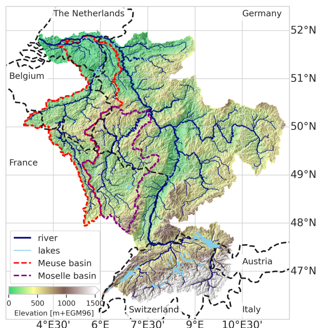
Figure 3. Study area. Rhine basin with average elevation, rivers and basin outlines based on the MERIT Hydro IHU 30 arcsec dataset (this paper); lakes are derived from the HydroLAKES dataset (Messinger et al., 2016).
