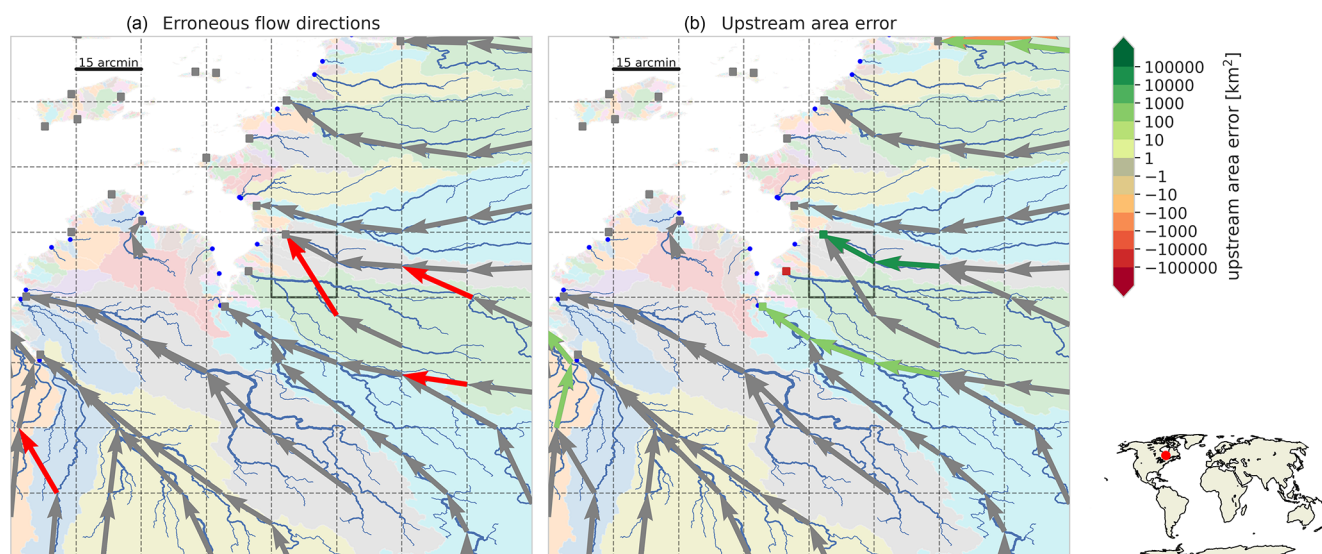
Figure C5. Largest basin ( 42\,017\text{ km}^2 ) with a relative upstream area error of more than 10 % at the 15 arcmin resolution indicated with a highlighted cell. See the caption of Fig. C1 for a full description.
