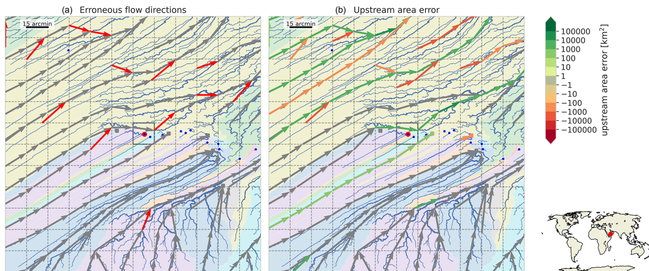
Figure C1. Largest endorheic basin ( 6996 \text{ km}^2 ) which is not resolved at the 15 arcmin resolution indicated with a highlighted basin pit. The blue lines show the fine-resolution river; the background colors show basin boundaries; the dashed lines show the coarse-resolution grid, and the arrows show the upscaled flow directions pointing from the outlet pixel or the original cell to the outlet pixel of the destination cell. Flow directions are red if erroneous (a), and green denotes a positive and red a negative upstream area error (b).
