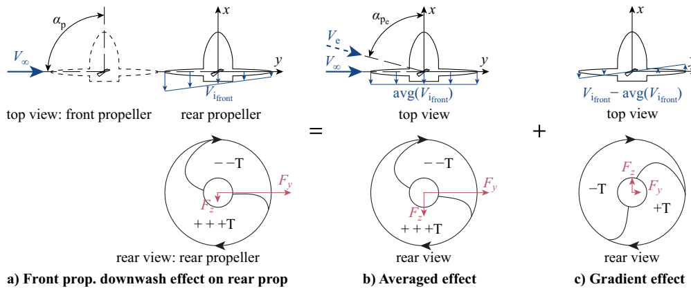
Fig. 16 Sketch showing the typical effect of SBS interaction on rear propeller (prop.) forces at \alpha_p = 90^\circ deg, relative to isolated propeller at \alpha_p = 0^\circ deg.
