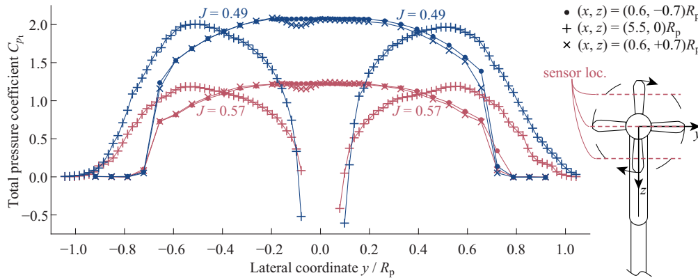
Fig. 14 Lateral distribution of C_{p_t} at x/R_p = 0.6 behind the pusher propeller for data 0.7 R_p below and above the propeller center and at x/R_p = 5.5 for data across the center, for V_\infty = 20 m/s and \alpha_p = 0 deg.
