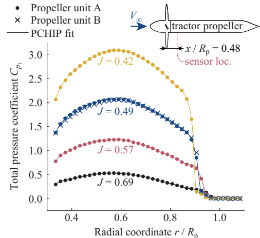
Fig. 12 Radial distribution of C_{p_i} at x/R_p = 0.48 at single azimuthal location (loc.) behind the two propeller units for V_\infty = 20 m/s and \alpha_p = 0 deg with piecewise cubic Hermite interpolating polynomial fit.
