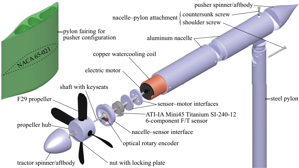
Fig. 4 Exploded view of propeller unit A with F/T sensor, indicating the various components.
