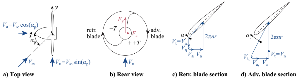
Fig. 9 Sketch showing the typical effect of angle of attack on propeller forces, relative to propeller at \alpha_p = 0 deg, including velocity triangle for retreating (retr.) and advancing (adv.) blade section with induced velocity components V_{ai} and V_{ti} .
