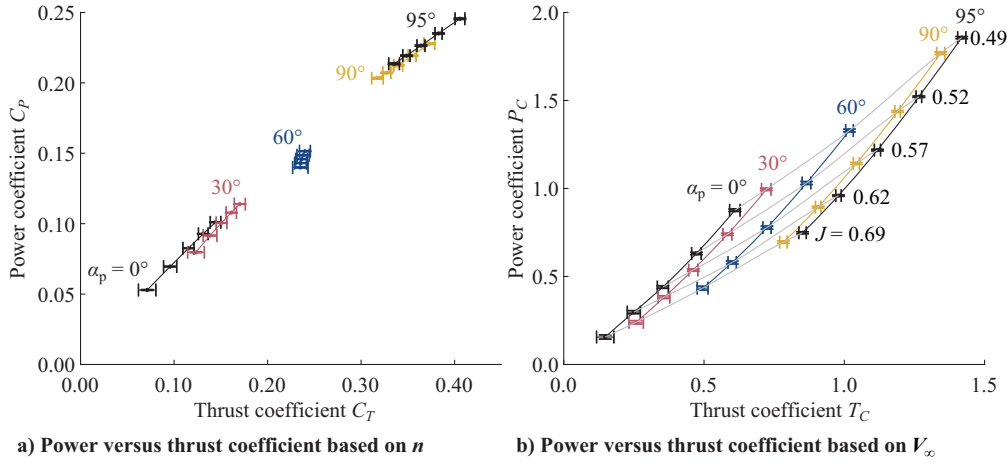
Fig. 10 ISO propeller power vs thrust at various J and propeller angles of attack for V_\infty = 20 m/s, measured with the F/T sensor.
