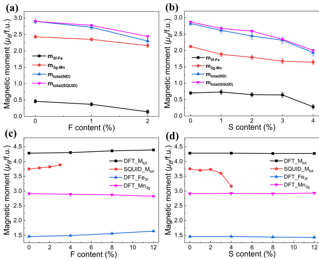
Fig. 7. Experimental magnetic moments obtained from ND and SQUID magnetization measurements at RT for (a) \text{Mn}_{0.60}\text{Fe}_{1.30}\text{P}_{0.64}\text{Si}_{0.36}\text{F}_x ( x = 0.00, 0.01, 0.02 ) and (b) \text{Mn}_{0.60}\text{Fe}_{1.25}\text{P}_{0.66-y}\text{Si}_{0.34}\text{S}_y ( y = 0.00, 0.01, 0.02, 0.03, 0.04 ) alloys. The magnetic moments derived from DFT calculations and magnetization measurements at 5 K as a function of (c) F and (d) S content.
