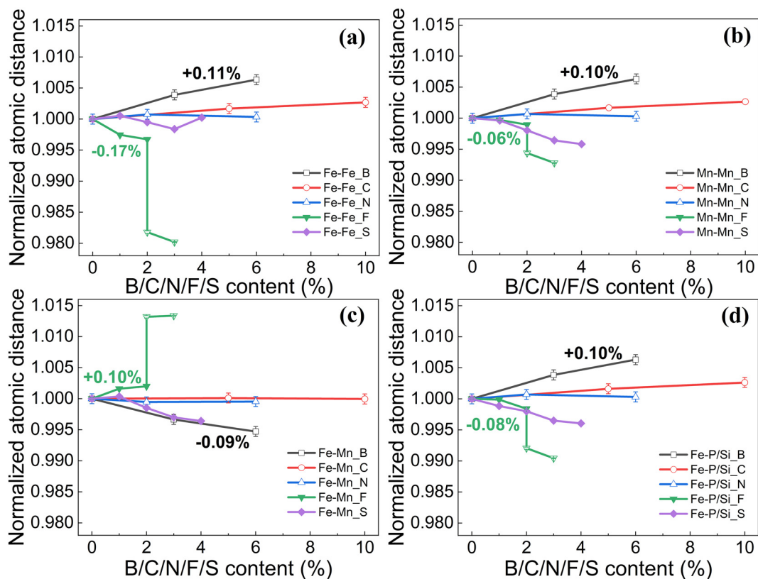
Fig. 8. Normalized interatomic distances of (a) Fe-Fe, (b) Mn-Mn, (c) Fe-Mn and (d) Fe-P/Si as a function of different B, C, N, F and S dopant concentrations for (\text{Mn,Fe})_2(\text{P,Si}) -based materials, determined from neutron diffraction. Note that the marked normalized atomic distance has been rescaled per dopant concentration (at.%).
