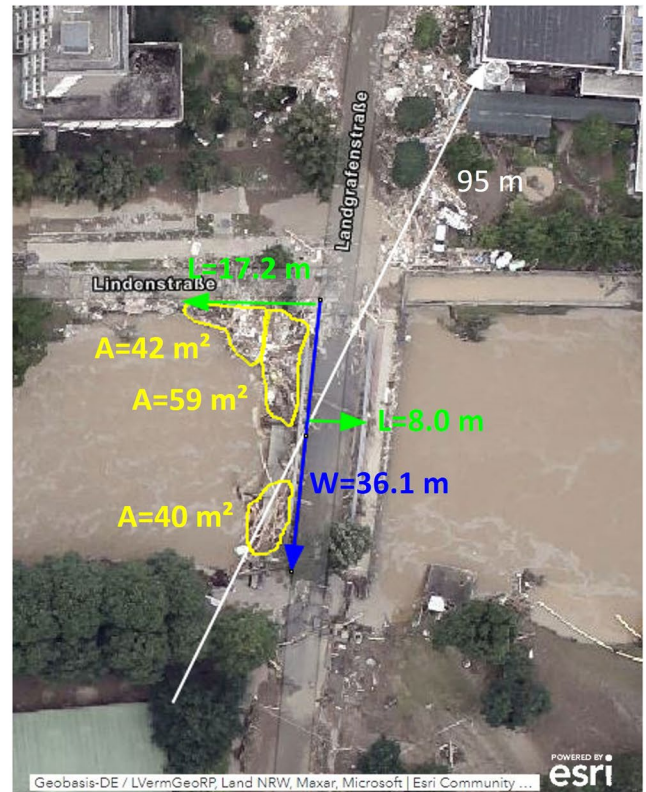
Fig. 3 Example of measurement of accumulation dimensions (W: width, L: length, H: height) and volume V, using photos from different perspectives (bridge 10016 in the database, Bad Neuenahr, Germany). Known dimensions of the bridge or surroundings are used for scale (indicated in white). Distances and areas directly measured on the photos are indicated in blue, green, magenta and yellow. The height of the three (yellow) areas is estimated rather than measured directly on the photo, given the lack of an undistorted straight-on perspective. Note the entanglement of debris with the bridge arch.
