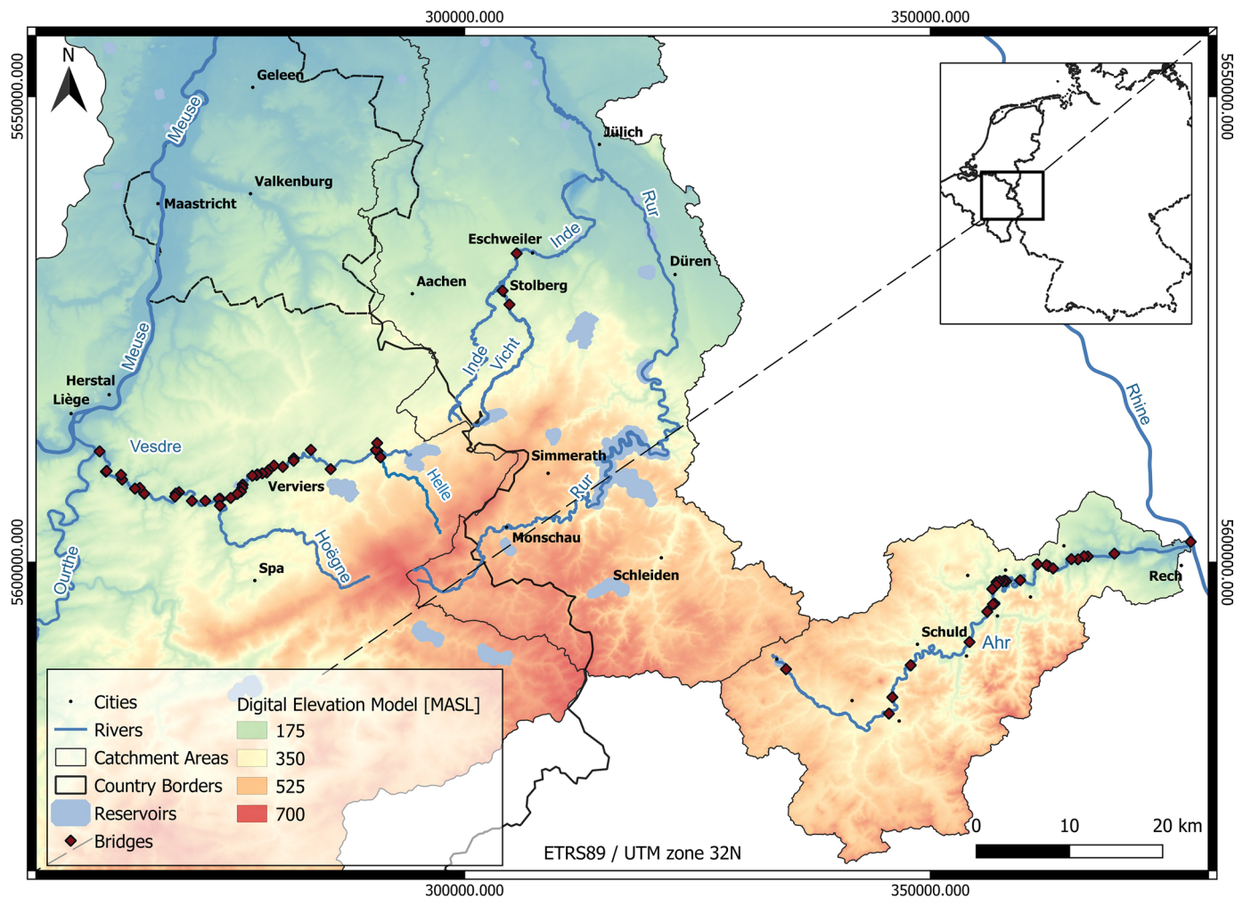
Fig. 1 Surveyed rivers and bridges with debris accumulations in Belgium and Germany 31 .
