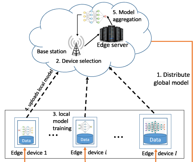
Fig. 1. Framework of FL-enabled edge devices. Each selected edge device downloads the global model from the edge server, then uses its source data to update a local model. The edge server aggregates the local models to update the global model, which is distributed to the edge devices.
