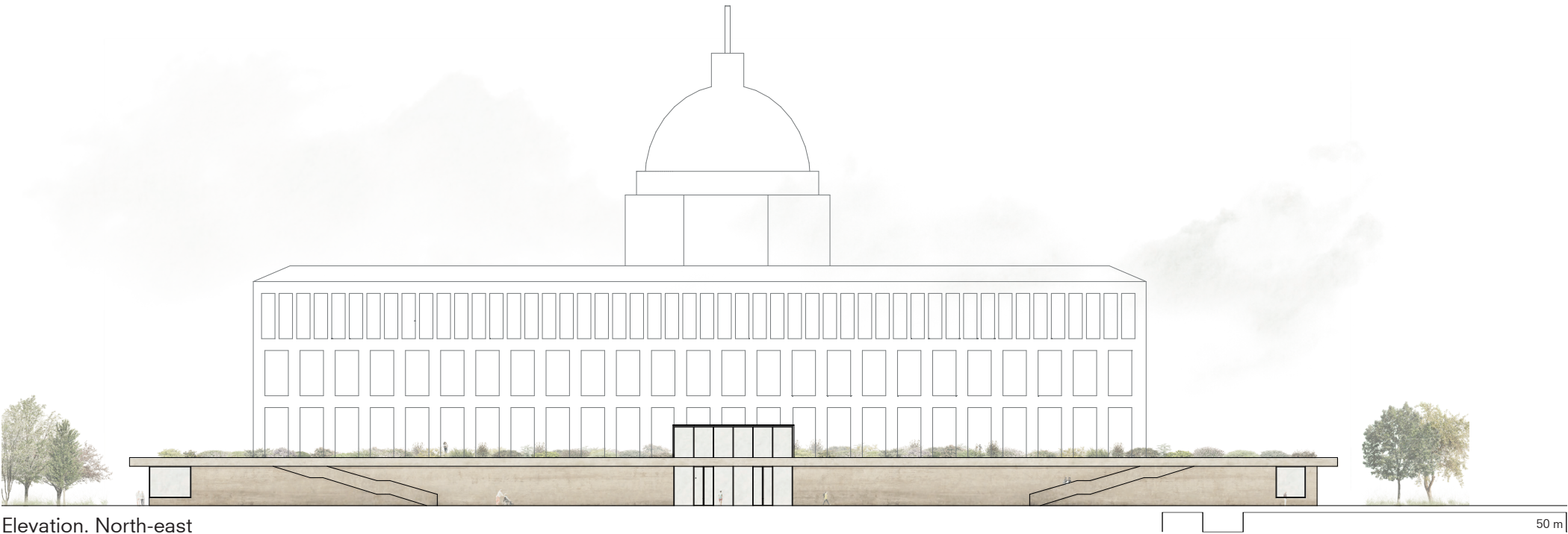
Elevation. North-east
