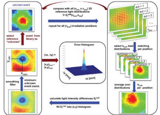
Fig. 3. Workflow chart of the CAP version of the kNN algorithm for extracting the interaction position of an unknown impinging gamma ray in the monolithic LaBr 3 (Ce) scintillator, in this case taken from a reference library to quantify the spatial resolution from the FWHM (Full Width Half Maximum) of the error histogram created from deviations between real and calculated photon interaction positions.
