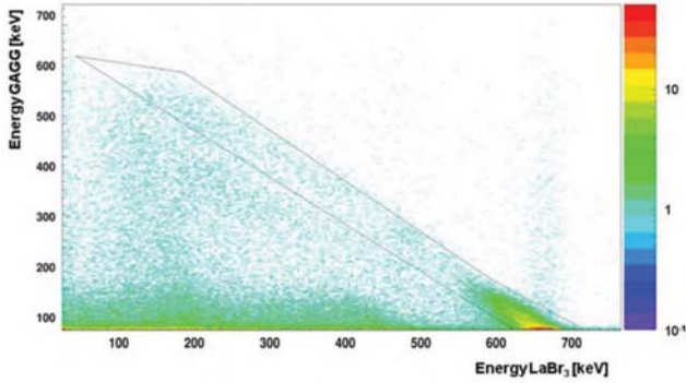
Fig. 4. Registered sum energy in the GAGG detector array (scatterer) versus the sum energy registered in the LaBr 3 (Ce). The black trapezoid encloses the coincident Compton scattering events selected as the data basis for the subsequent reconstruction calculations.
