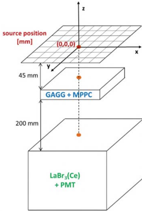
Fig. 2. Sketch of the Compton camera setup: the GAGG and LaBr 3 (Ce) detectors were placed in a distance of 200 mm. The 137 Cs source was placed in a distance of 45 mm from the scatterer component in a central position on the (x,y) plane: (0,0,0) [mm] in the coordinate system of the setup.
