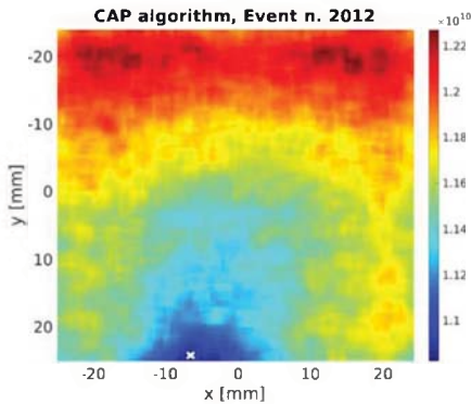
Fig. 5. Example of position reconstruction using CAP algorithm for one event registered in the monolithic LaBr 3 (Ce) scintillator. The white cross at the lower border indicates the calculated position of the photon source.
