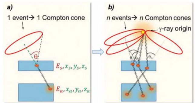
Fig. 1. Sketch of the image reconstruction process using a Compton camera system, composed of a scatterer and an absorber component. a) Compton scattering of an incident photon, where energies and positions are recorded in each of the two detector components, the scatterer and the absorber. Via the Compton kinematics, the Compton cone can be reconstructed: the energy and position information allows, respectively, to determine its axis and its aperture angle (scattering angle \theta ). b) The intersection of different cones reconstructed from all the different photon events allows to reconstruct the photon source position, corresponding to the interaction position of the proton / ion beam in the patient.
