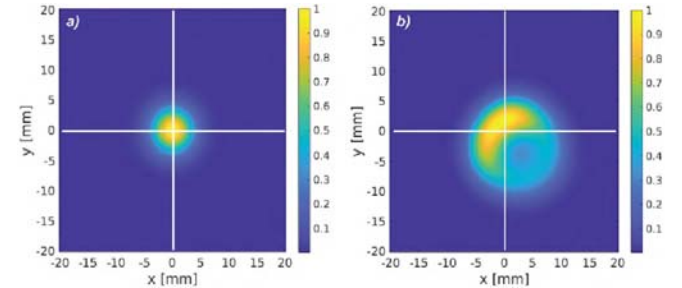
Fig. 6. Reconstructed source position images from a) simulated data and b) experimental data.
