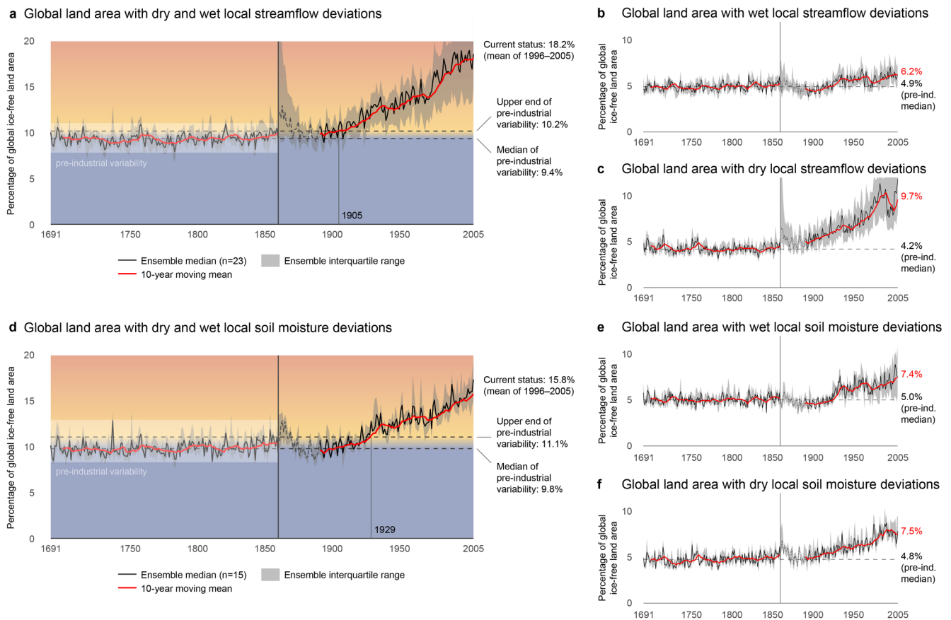
Extended Data Fig. 1 | Percentage of global ice-free land area with local deviations, separately for summed, wet and dry deviations. Panels show the percentage of land area with local streamflow (a–c) and soil moisture (d–f) deviations, dry and wet local deviations summed (a, d), and for wet (b, e) and dry (c, f) local deviations separately. Shown is the annual percentage, which is computed as an average of monthly percentages. The annotated years mark the 10-year moving (trailing) mean transgressing the upper end of pre-industrial variability (95th percentile of the pre-industrial percentage of land area with local deviations; Fig. 1d). The ensemble median and interquartile range are computed
