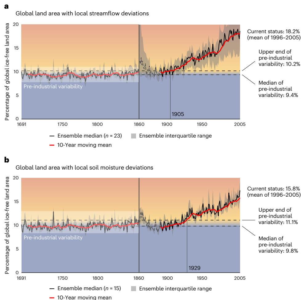
Fig. 2 | Percentage of global ice-free land area with local deviations. a,b, For streamflow (a) and soil moisture (b), the annual percentage is shown, which is computed as an average of monthly percentages. The annotated years mark the 10-year moving (trailing) mean transgressing the upper end of pre-industrial variability (95th percentile of the pre-industrial percentage of land area with local
