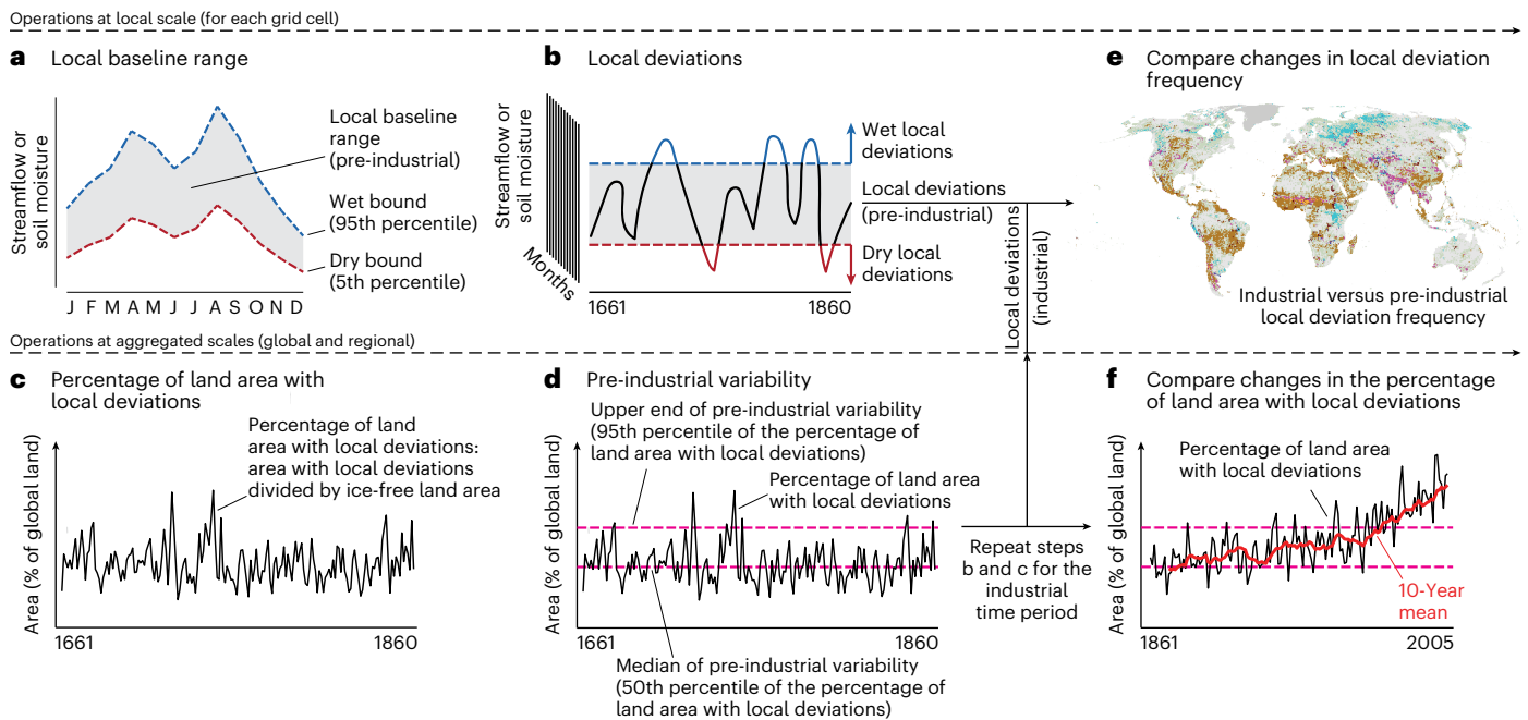
Fig. 1 | Methodological outline. a–f , The analysis steps consist of setting the local baseline range ( a ), identifying local deviations ( b ), computing the percentage of land area with local deviations ( c ), defining pre-industrial variability ( d ), and comparing the industrial period against the pre-industrial period locally ( e ) and at global and regional scales ( f ). The steps a–d are described in detail in Methods.
