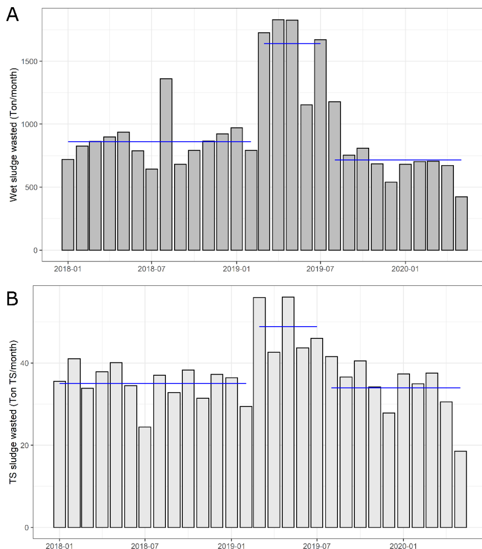
Figure 2. Monthly waste sludge production. (A) Tons of wet sludge produced (B) Tons of TS produced, based on the measured TS content of the waste sludge (40 g/L during normal operation and 31 g/L during the test period). The blue lines indicate the average sludge production in the periods before, during and after the test period.
