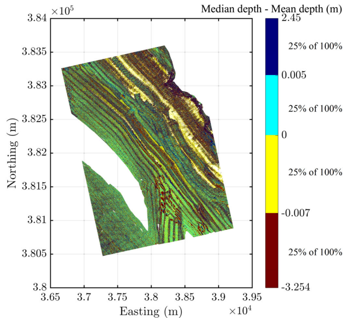
Fig. 3. (Color) Map of the difference between the median and mean depths for Area A. The range of values represented by each color is such that each range represents an equal percentage of the data.
