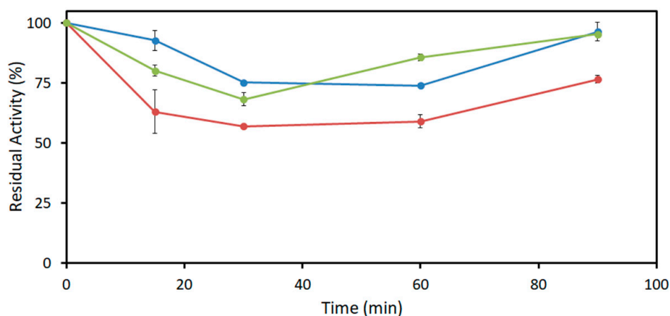
Figure 4. Time-dependent activity of Pa DERA C49M during incubation at different acetaldehyde concentrations (100 mM (blue), 200 mM (red) and 300 mM (green)) to estimate the residual activity using the standard assay protocol. The residual activity after incubation in the absence of acetaldehyde was 3.5 U/mg and was normalized to 100%.
