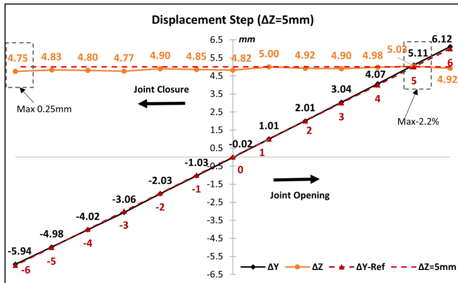
Fig. 13. Measurement result comparison ( \Delta Z = 5 mm).
