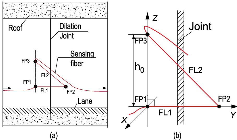
Fig. 5. Sensor layout for joint two-directional displacement measurement:(a) Field layout;(b) Installation status.
