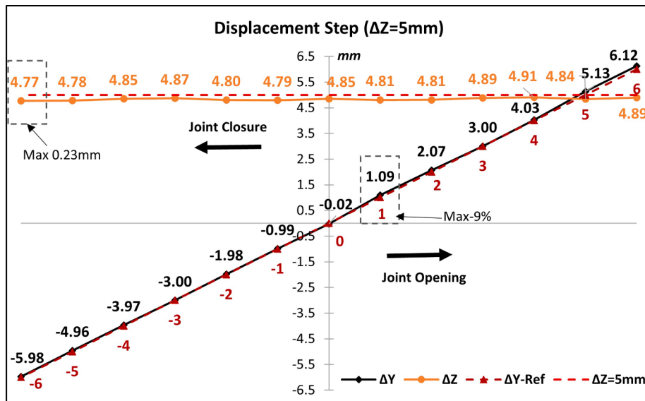
Fig. 9. Measurement result comparison of D-0.9 mm fiber ( \Delta Z = 5 mm).
