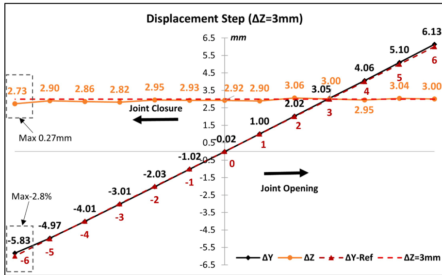
Fig. 12. Measurement result comparison ( \Delta Z = 3 mm).
