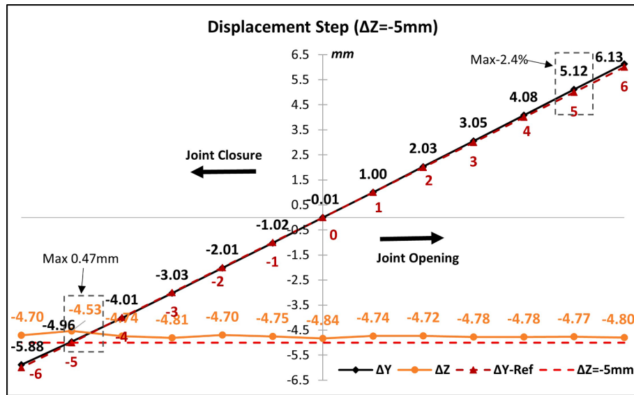
Fig. 16. Measurement result comparison ( \Delta Z = -5 mm).
