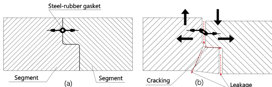
Fig. 1. Dilation joint deformation at tunnel roof: (a) schematic of a typical dilation joint and (b) deformed joint.
