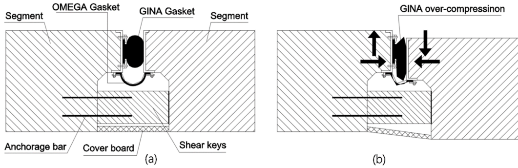
Fig. 2. Immersion joint deformation at tunnel roof: (a) Schematic of a typical immersion joint and (b) deformed joint.
