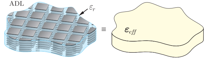
Fig. 3. A planar ADL slab hosted by a homogeneous dielectric of permittivity \epsilon_r to realize an equivalent anisotropic medium.
