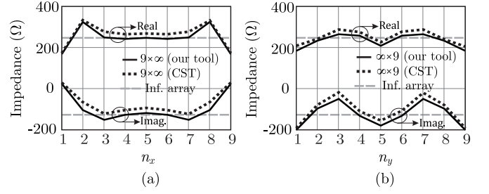
Fig. 7. Active input impedance for an array of (a) 9 \times \infty and (b) \infty \times 9 elements, at the frequency 0.5f_0 and as a function of the element index. The unit-cell geometry is defined in Tab. I.
