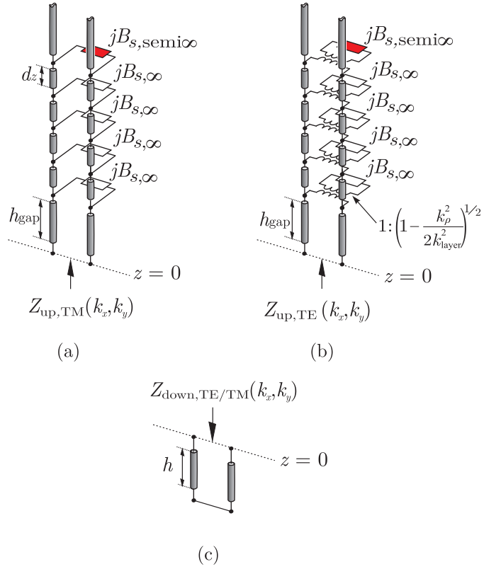
Fig. 4. Equivalent transmission-line model of a finite-height ADL for a generic (a) TM and (b) TE plane wave; (c) equivalent shorted line representing the backing reflector.
