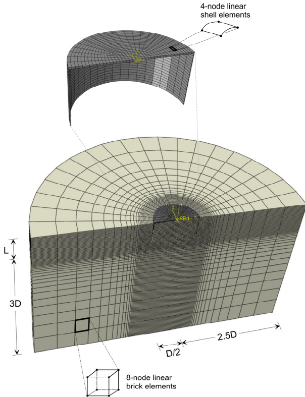
Figure 1. Numerical model.
