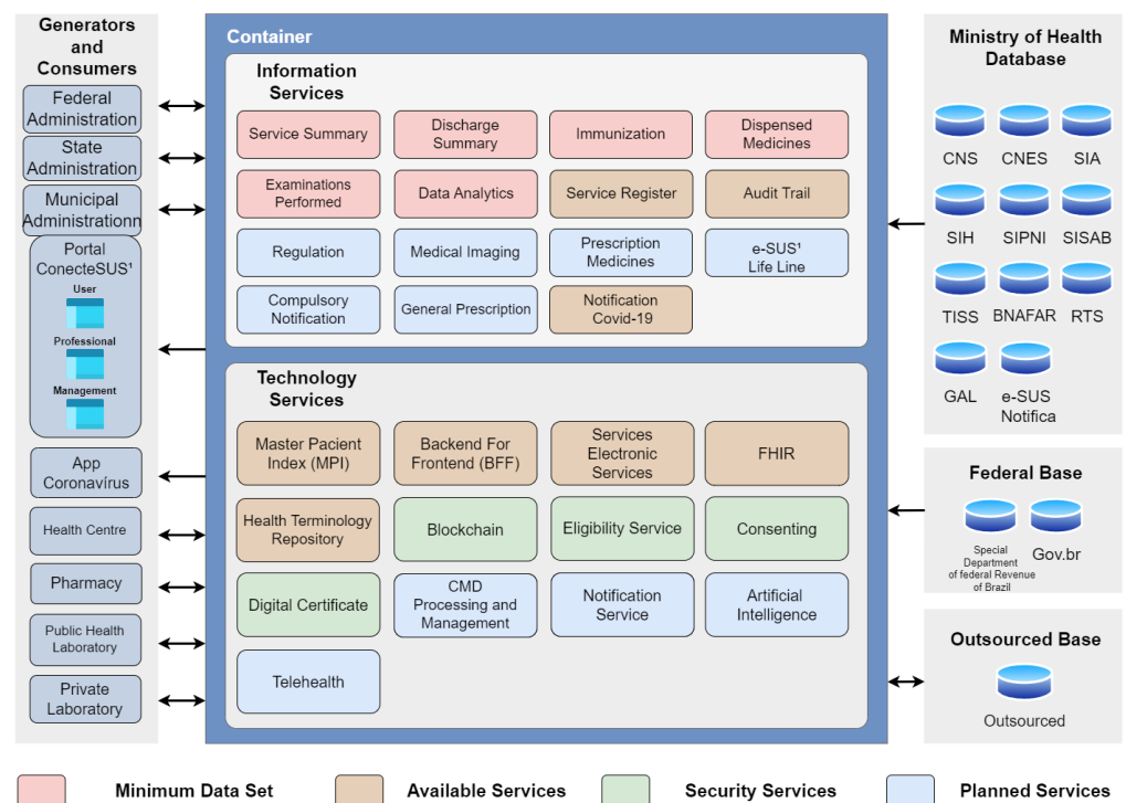
Figure 13. The RDNS architecture.
