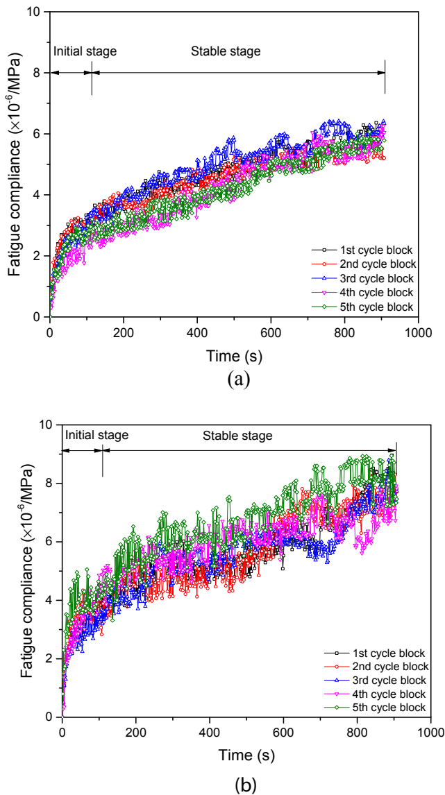
Fig. 20. The evolution of fatigue compliance for (a) w/c 0.4 and (b) w/c 0.5.
