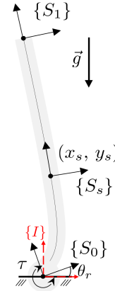
Fig. 1. Scheme of R-Soft Inverted Pendulum (R-SIP), the inherently under-actuated soft robotic system whose dynamics and control we characterize in depth in this work.
