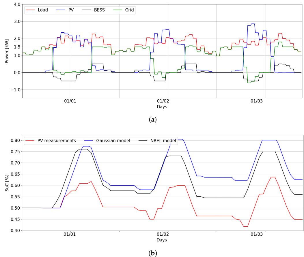
Figure 10. Power exchange using as a reference measured instant power measured (a), and (b) SoC of the battery during the peak-shaving operation, considering a maximum allowed power purchased from the grid of 1.5 kW.
