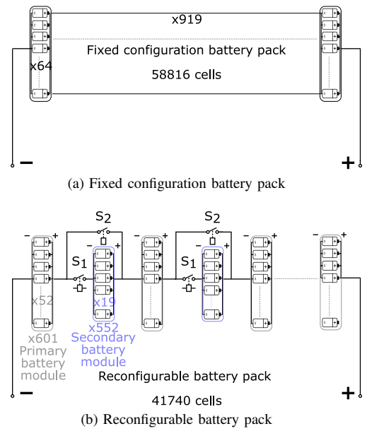
Fig. 3. Schematic of both battery packs
