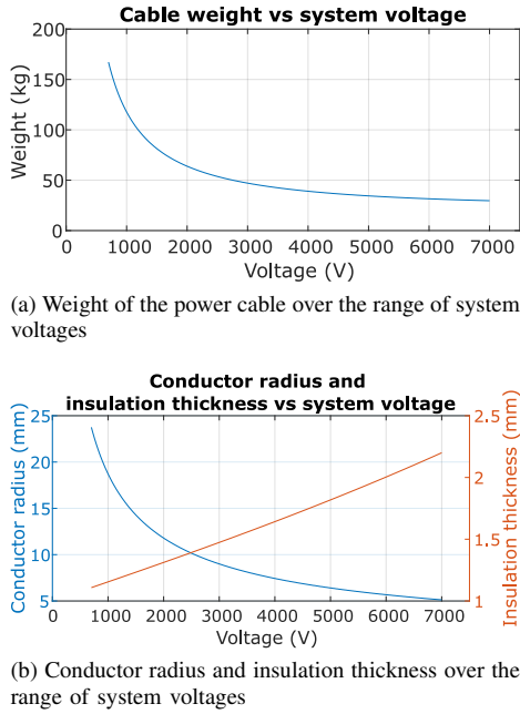
Fig. 2. Change in parameters of power cables over the range of system voltages
