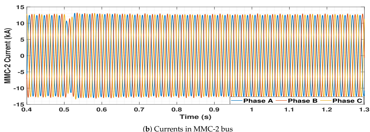
Figure 26. Currents in (a) MMC-1 bus and (b) MMC-2 bus upon OWF-2 disconnection event.
