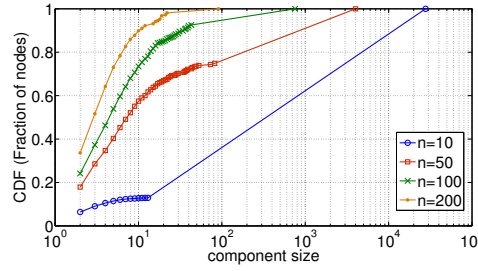
Fig. 13. The CDF of component size for different values of interaction threshold n (Dota-League, SM graph).
