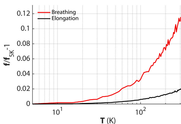
Fig. 8. Relative change of frequency with temperature for the first RBM (breathing) and the longitudinal mode (elongation) for the (8, 8) CNT in the fully clamped configuration. Frequency at 5 K: 34.9 GHz (radial), 127.1 GHz (longitudinal).
