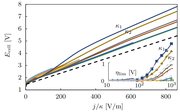
Fig. 7. The cell voltage recorded with the set-up of Fig. 2 for conductivities \kappa_1 = 2.04 S/m, \kappa_2 = \sqrt{2}\kappa_1 = 2.89 S/m, etcetera. The dashed line gives E_0 + j/l/\kappa using the parameters of Table 1. The inset plot gives the hydroxide depletion concentration overpotential \eta_{\text{lim}} = E_{\text{cell}} - E_{\text{eq}} - \eta_a - \eta_c - j/l/\kappa - ARj , where the gray dashed lines give the parametrization of Eqs. (6)–(9).
