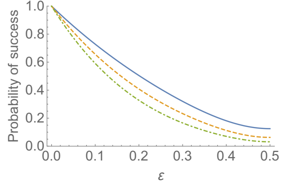
FIG. 3. Optimal success probability. The optimal success probability p_{\text{succ}}^{\text{opt}} is plotted as a function of \epsilon in the [0,0.5] range for N = 3, 4 , and 5 (solid, dashed, and dot-dashed curves, respectively). The function assumes values from 1 to \frac{1}{2^N} . The function goes from 1 , when no operation is performed over system B , to \frac{1}{2^N} , when a perfect GHZ projector is performed.
