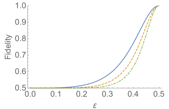
FIG. 4. Optimal fidelity. The optimal fidelity F^{\text{opt}} is plotted as a function of \epsilon for N = 3, 4 , and 5 (solid, dashed, and dot-dashed curves, respectively). Since the function is symmetrical with respect to \epsilon = 0.5 , the plot is represented only in the [0,0.5] range. The function goes from 0.5 , when no entanglement is generated, to 1 , when the final state is the maximal entangled |\text{GHZ}\rangle .
