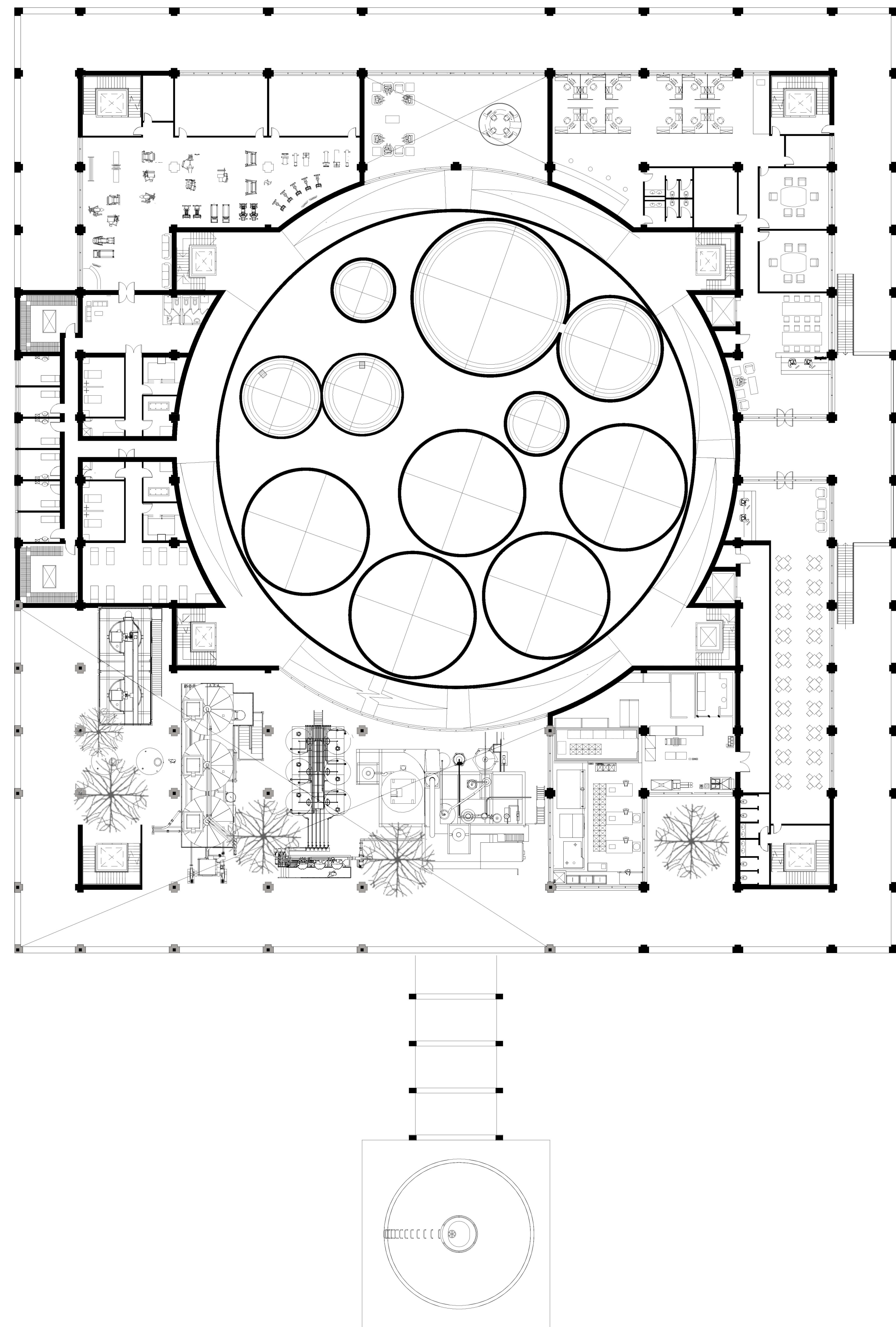
First floor plan 1:250
