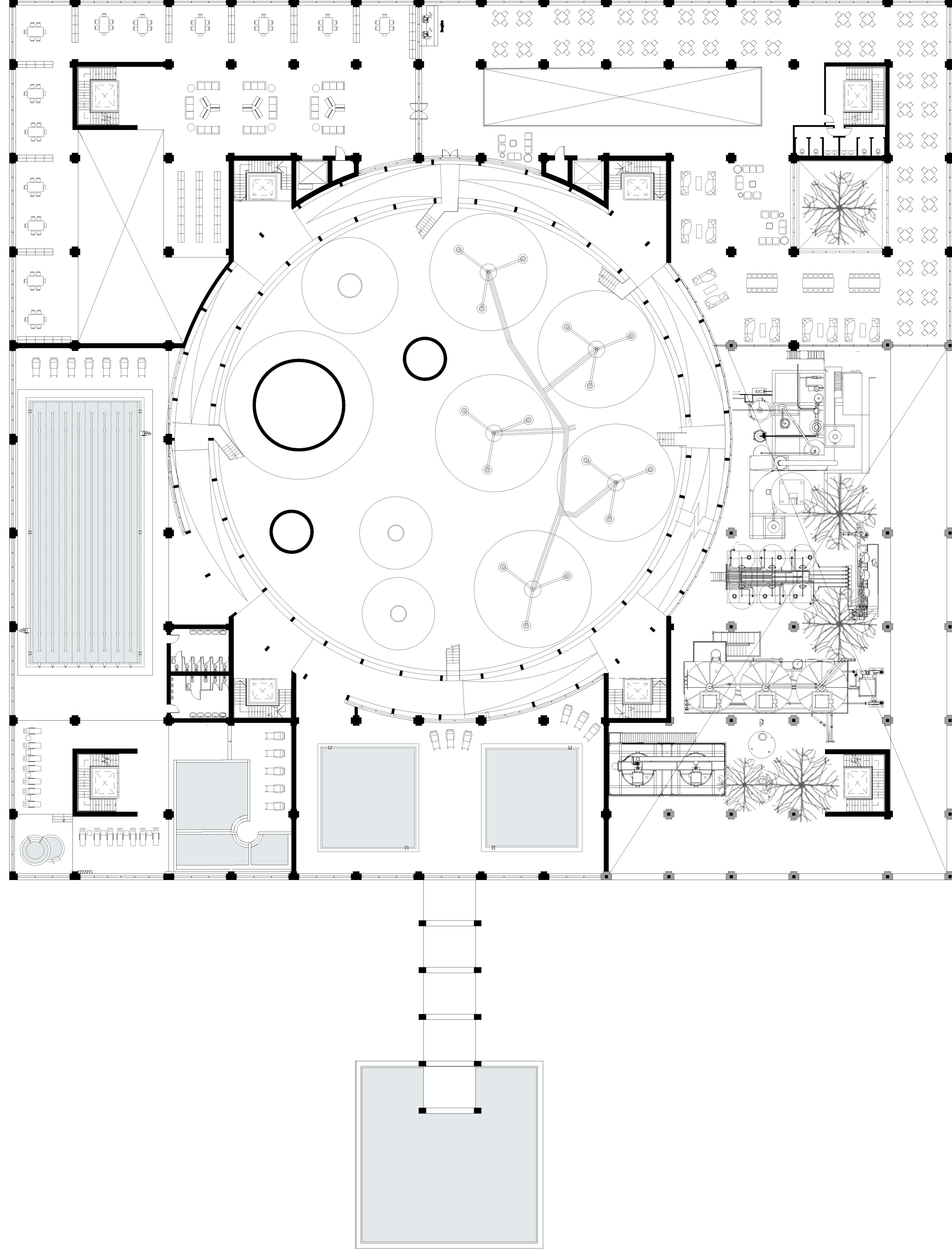
Second floor plan 1:250
