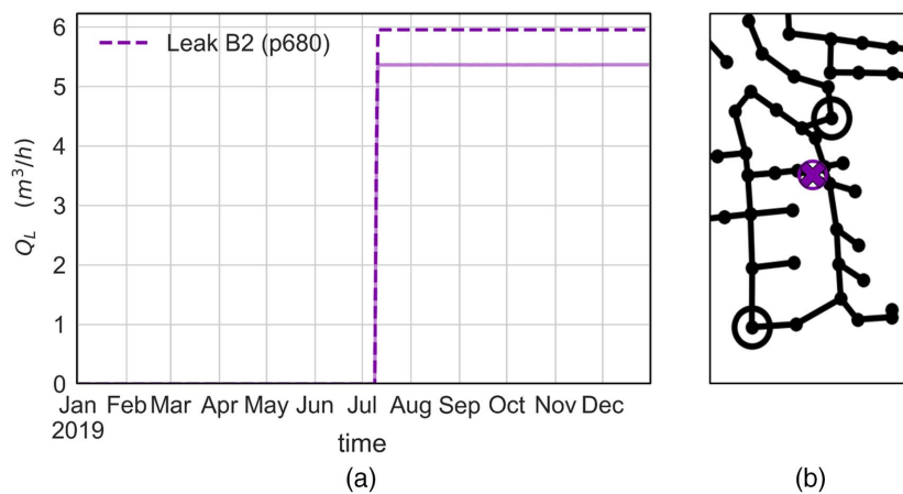
Fig. 7. Results of leak detection and localization for the unknown leaks in Area B in 2019: (a) identified leakage outflows over time; and (b) estimated locations of the leaks. The cross is the estimated leak location, the circle indicates the real locations.
