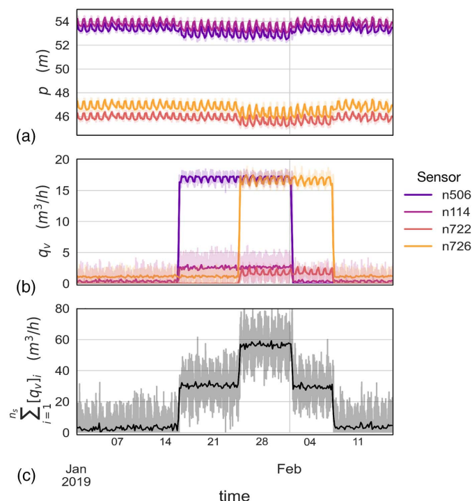
Fig. 5. Dual model signals for first two leaks in Area A in 2019 (location at Pipes p827 and p523 with magnitudes of approximately 27 m³/h each): (a) pressure measurements p over time; (b) sharp and localized signal of the virtual leak outflows q_v over time calculated by the dual model at the same measurement locations; and (c) the sum over all virtual leak flows in the dual model serves as good estimates for leak size.
