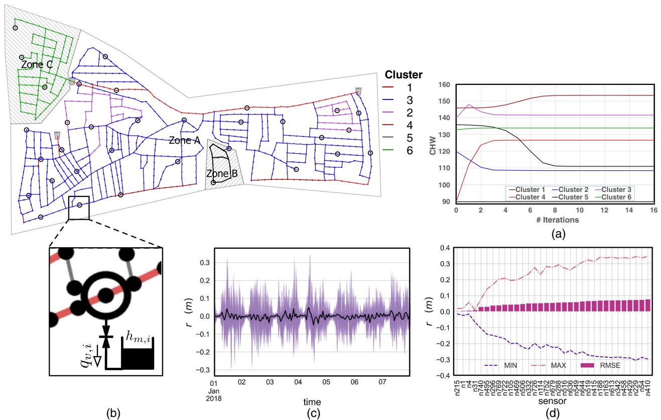
Fig. 2. Network colored by calibration clusters of Hazen-Williams roughness coefficients. Pressure measurements are shown as circles. (a) Roughness iterations; (b) the principle of the dual model, where the pressure measurements are replaced by the combination of a valve and a virtual reservoir whose head is equal to the measured head h_i , and the dual model transforms h_i into virtual leakage flows q_{v,i} ; (c) pressure residuals for the first week of 2018; and (d) the minimum, maximum, and root-mean-square errors (RMSEs) in increasing RMSE order.
