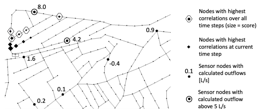
Fig. 10. Snapshot of the leakage isolation tool: calculated outflows at virtual reservoirs of sensor nodes and correlation results; small diamonds for current time step and large diamonds for sum of all time steps (the size represents the score).
