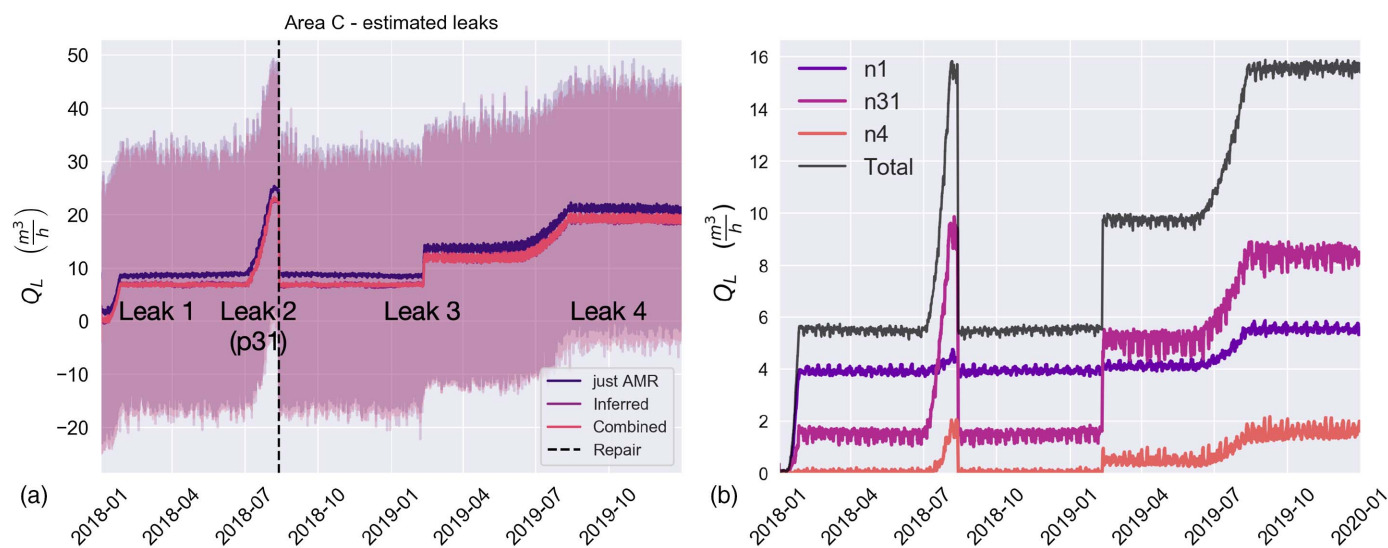
Fig. 4. Leakage outflow in Area C: (a) estimated by comparing the virtual inflow measurement and the demand model; and (b) as provided by the dual model.
