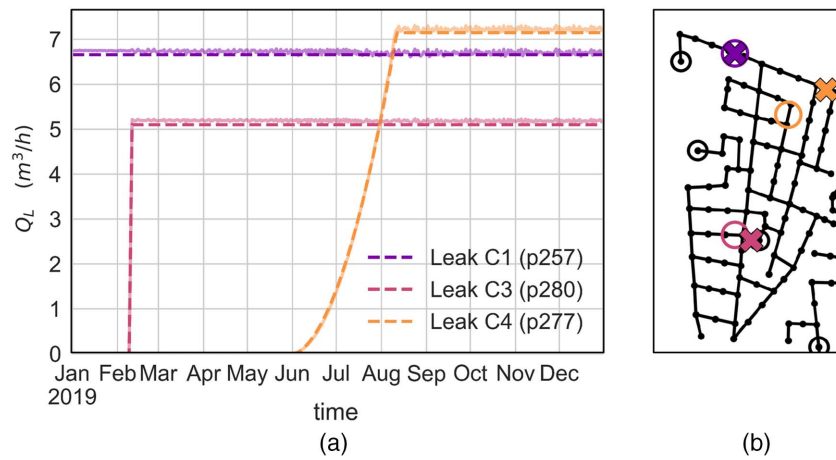
Fig. 6. Results of leak detection and localization for the unknown leaks in Area C in 2019: (a) identified leakage outflows over time; and (b) estimated locations of the leaks. Crosses are the estimated leak locations, circles indicate the real locations.
