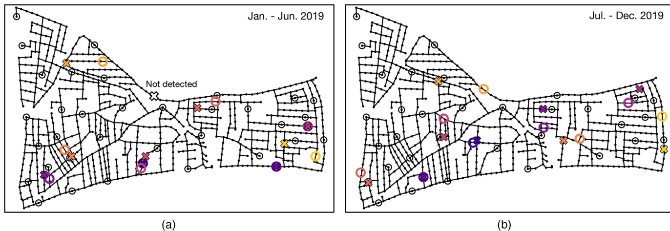
Fig. 9. Results of leak localization for the unknown leaks in Area A in 2019: (a) first half of the year from January to June; and (b) second half of the year from July to December. The not detected leak at Pipe 427 is shown as a white cross in (a). Crosses are the estimated leak locations, circles indicate the real locations.
