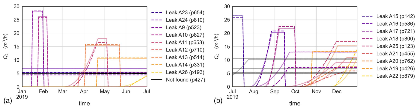
Fig. 8. Results of leak detection for the unknown leaks in Area A in 2019: leakage outflows for the (a) first half of the year; and (b) second half of the year. The second half also includes the ongoing leaks from (a) as shaded lines. Additionally, the missed detected leak at Pipe p427 is shown in (a).
