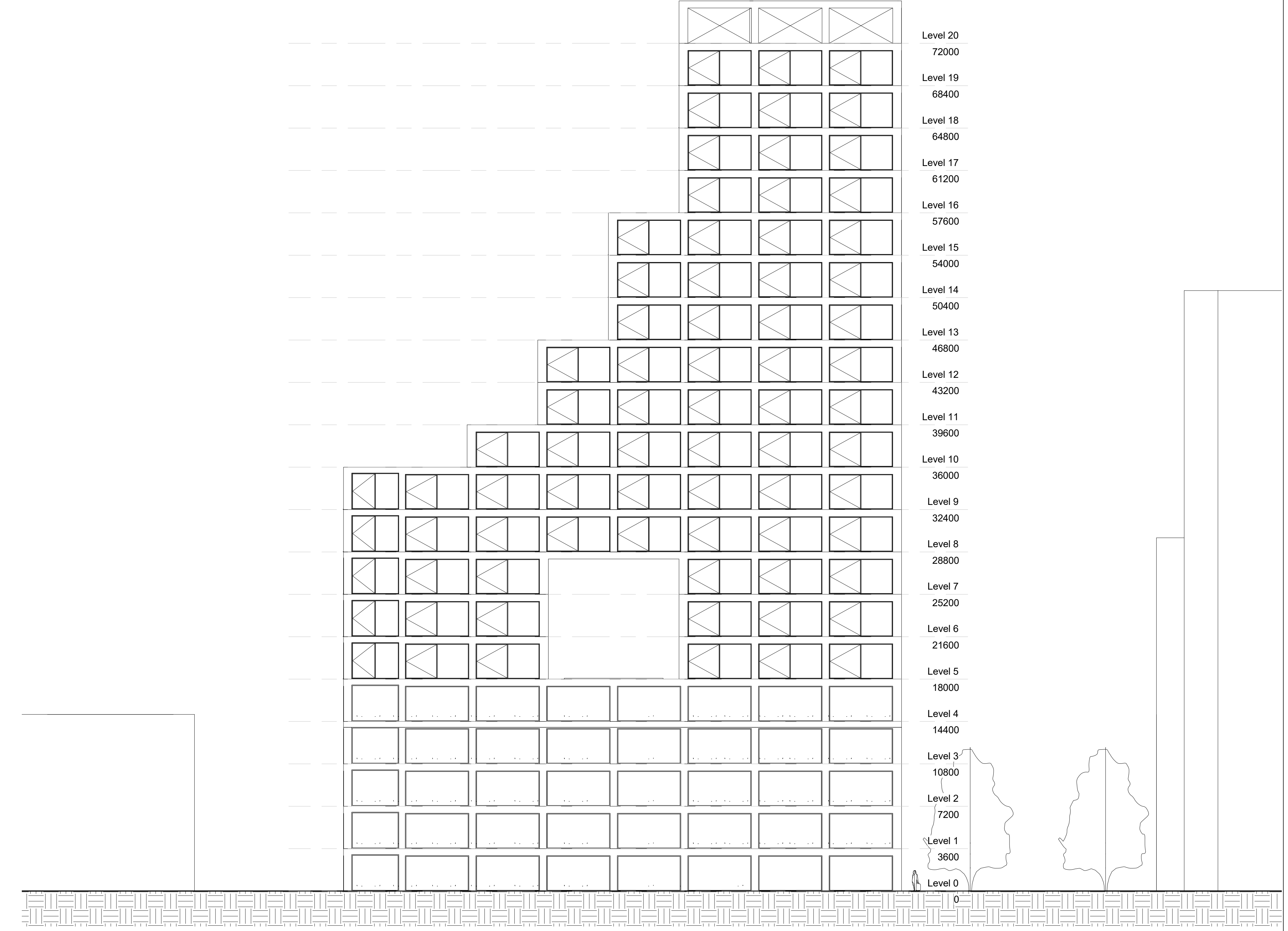
1 East Facade 1 : 200
